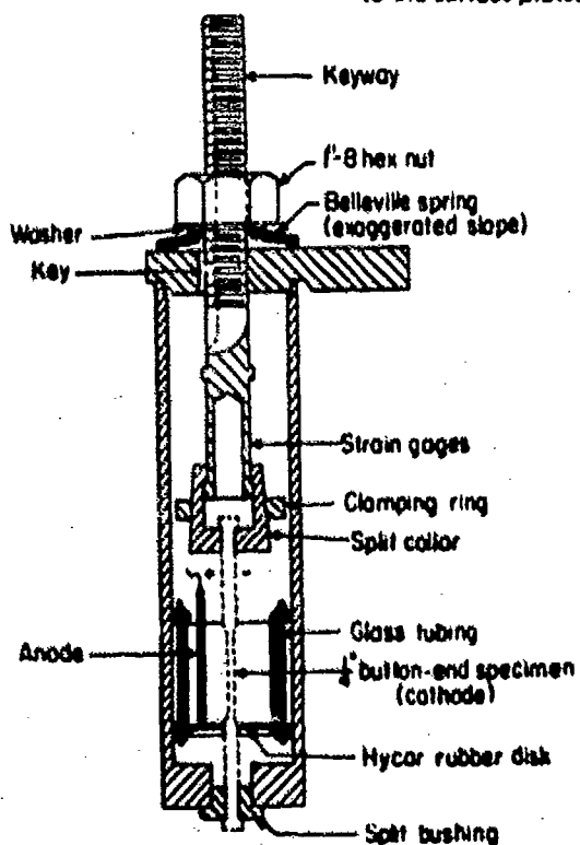
Fig. 1.11 - Static-loading device for testing 1/4 in. button head specimens. An electrolytic cell is incorporated for charging specimens with hydrogen while under stress.
