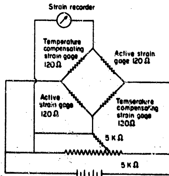
Fig. 1.17 - Strain gage wiring diagram.
