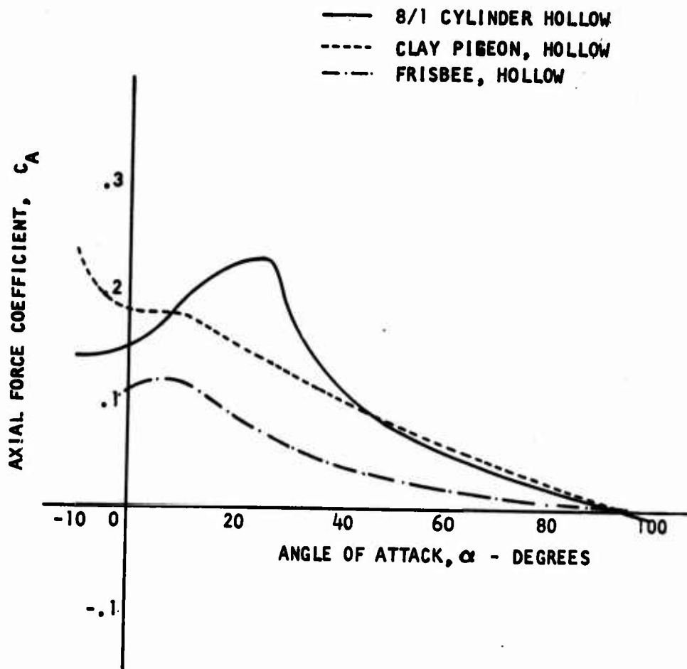
Figure 44. Axial Force Coefficients for Typical Hollow Self-Suspended Flare Shapes (Nonspinning)
