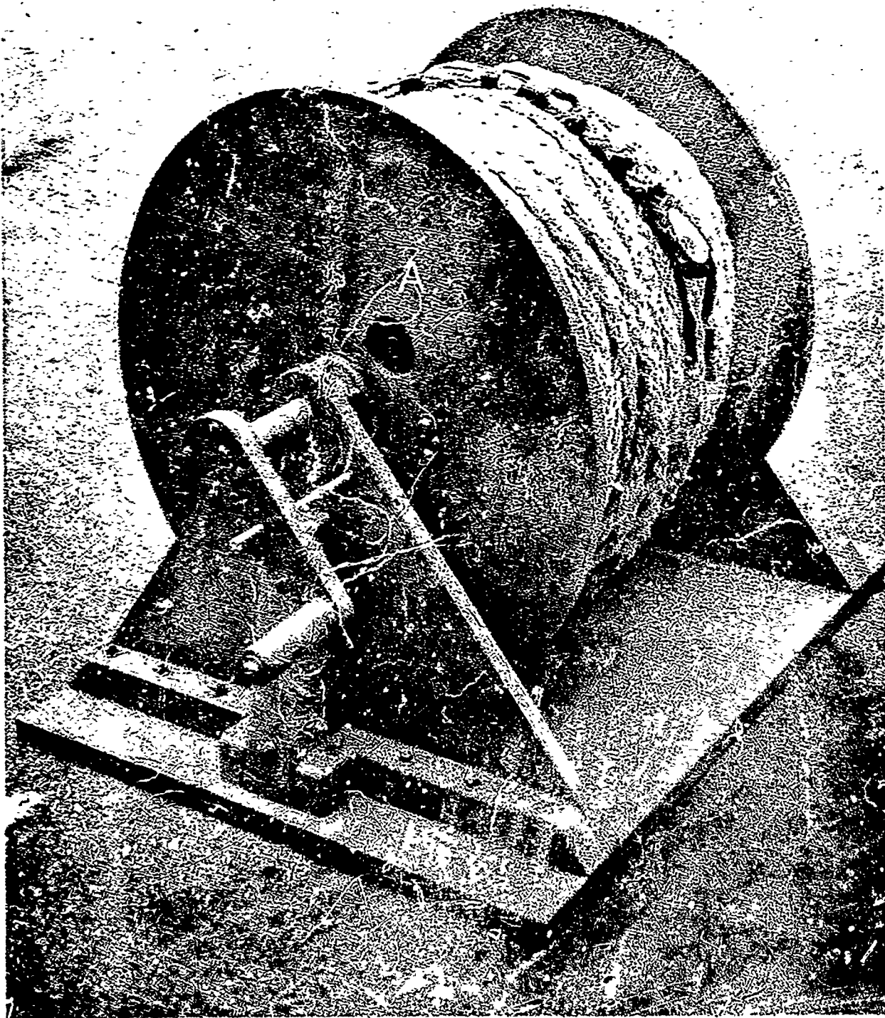
Figure 27. Winch
