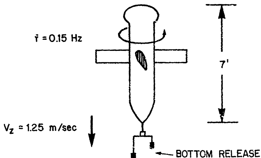
Figure 9. Free-Fall GEK.
