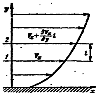
Figure 24.5. Illustration used to derive formula for finding molecular mean free path.
