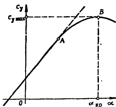
Figure 18.1. Lift coefficient of asymmetric profile versus angle of attack
