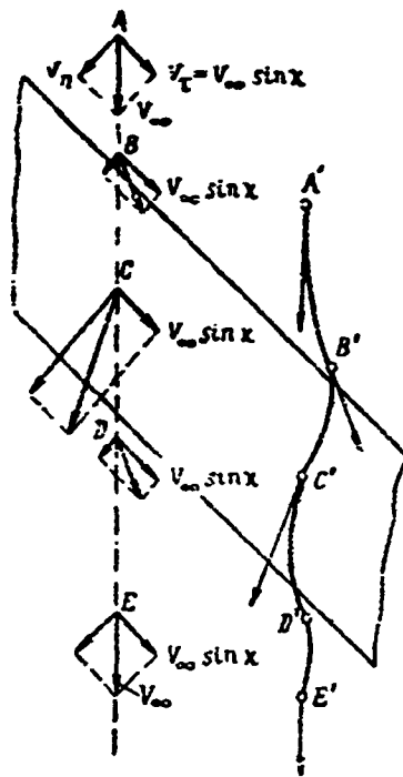
Figure 17.4. Variation of velocity and streamline direction near surface of yawed wing.
