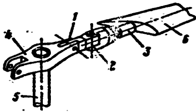
Figure 26.1. Main rotor blade mounting: 1 - horizontal hinge; 2 - vertical hinge; 3 - axial hinge; 4 - hub; 5 - shaft; 6 - blade.
