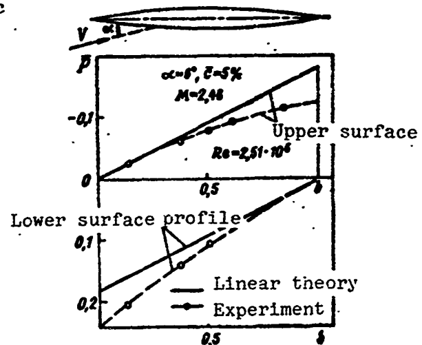
Figure 15.5. Comparison of theoretical and experimental values of pressure coefficients of a symmetric profile
