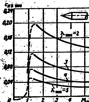
Figure 21.6. Wave drag coefficient of nose section of conical body of revolution versus M_\infty .
