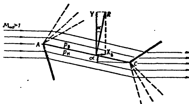
Figure 15.1. Supersonic flow past flat plate
