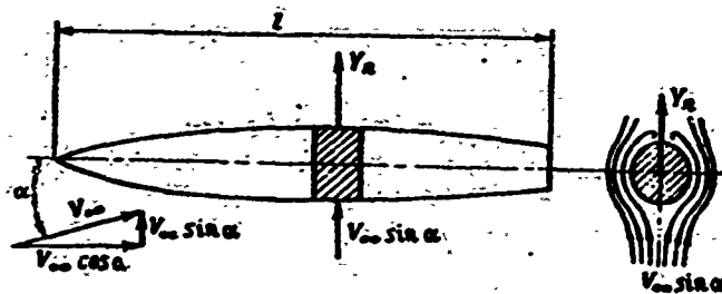
Figure 21.3. Normal force caused by crossflow on body of revolution.
