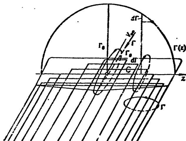
Figure 16.4. Vortex system of finite-span wing
