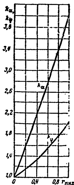
Figure 23.7. Curves for determining interference coefficients k_\alpha and k_\phi .
