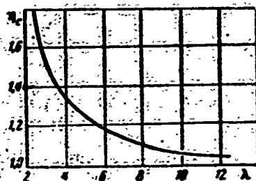
Figure 21.5. - Correction factor \eta_c versus fineness ratio of body of revolution.
