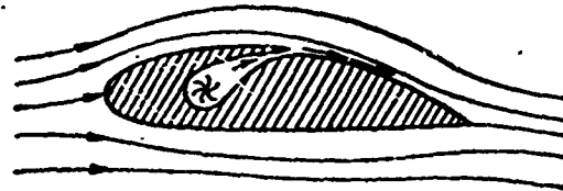
Figure 11.15. Separation-free flow past wing profile in presence of blowing
