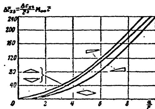
Figure 24.4. Coefficient \Delta \bar{c}_x w versus corrected angle of attack \alpha/\bar{c} for different profiles.
