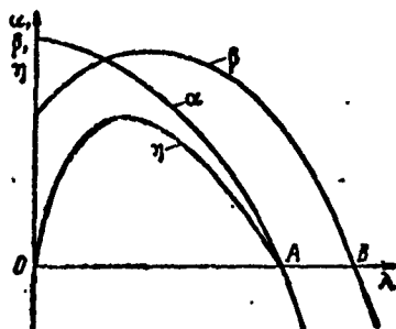
Figure 25.8. Propeller operating characteristics with \phi = constant.
