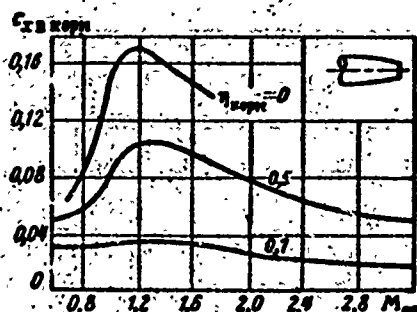
Figure 21.7. Wave drag coefficient of parabolic boattail versus M_\infty ( \lambda_{aft} = 2 ).
