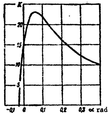
Figure 12.7. Wing profile efficiency versus angle of attack
