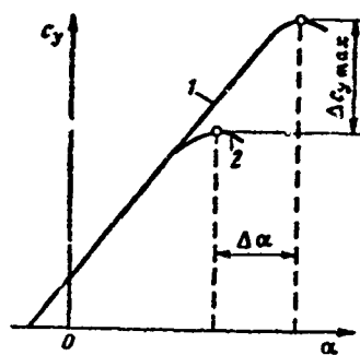
Figure 18.17. Curve c = f(\alpha) for wing with and without slats:
