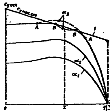
Figure 18.3. Change of spanwise c_y \sec distribution for trapezoidal wing with increase of \alpha
