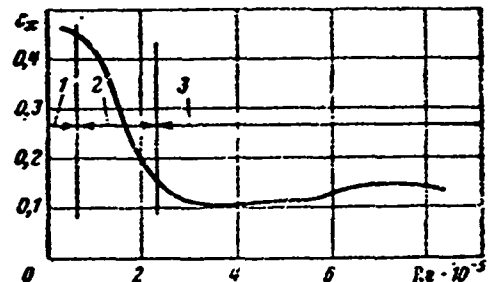
Figure 11.11. Sphere drag coefficient versus Re :
