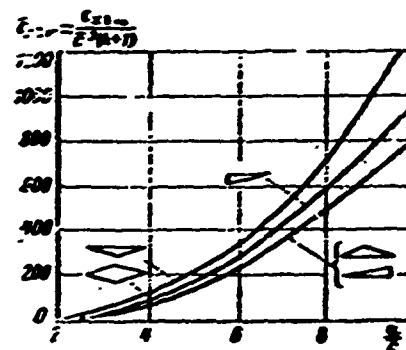
Figure 24.3. Coefficient \bar{c}_x w^\infty versus corrected angle of attack \alpha/\bar{c} for different profiles.
