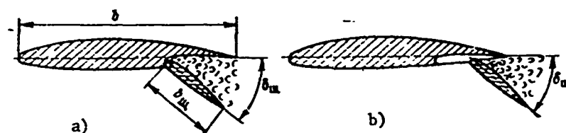
Figure 18.9. Split flaps: a - simple; b - extending
