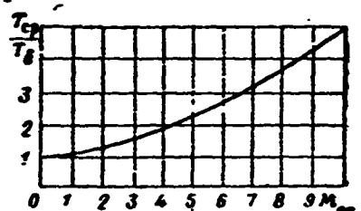
Figure 13.4. Temperature in turbulent boundary layer versus M_\infty
