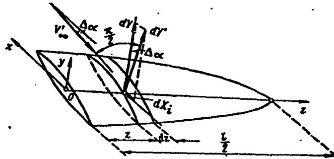
Figure 6.11. Calculation of forces acting on wing
