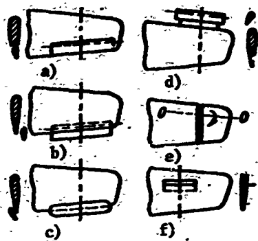
Figure 22.4. Ailerons:
