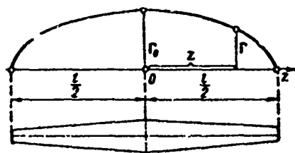
Figure 16.14. Elliptic circulation distribution along wing span
