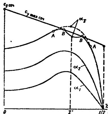
Figure 18.5. Change of spanwise c_{y \text{ sec}} distribution for swept wing with increase of \alpha
