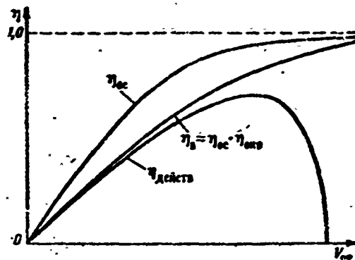
Figure 25.5. Variation of axial efficiency and efficiency of ideal and real propellers with flight speed.
