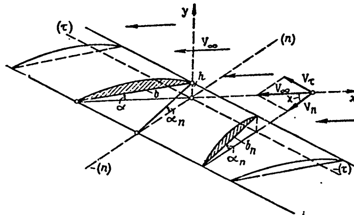
Figure 17.6. Yawed wing of infinite span.
