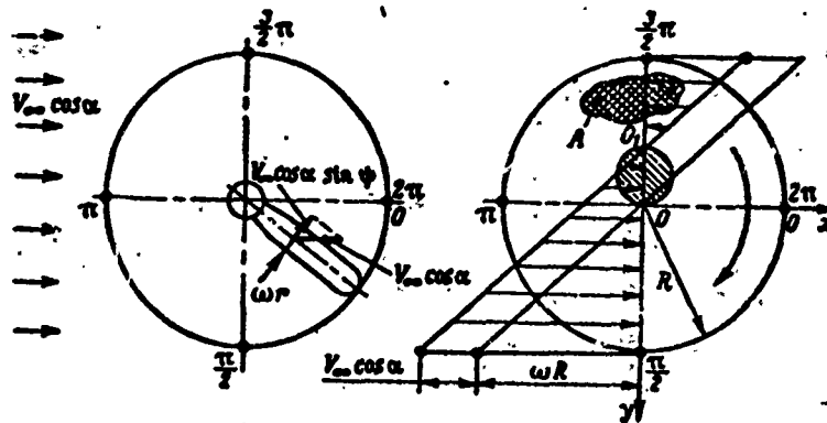
Figure 26.7. Tangential velocities on main rotor blades.
