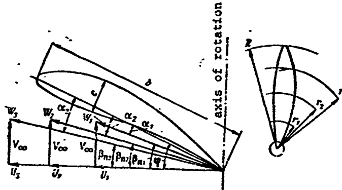
Figure 25.1. Geometric and kinematic characteristics of blade profile.
