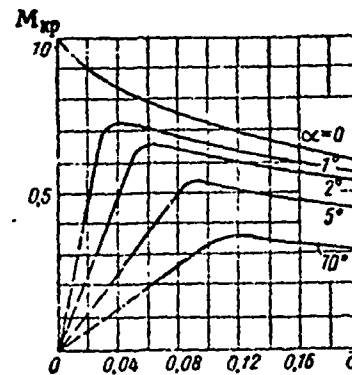
Figure 14.4. Effect of profile relative thickness and angle of attack on M_{cr}
