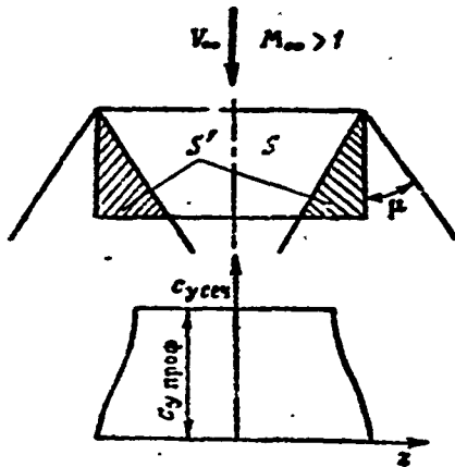
Figure 20.1. Influence of wing tips for supersonic flow around wing.
