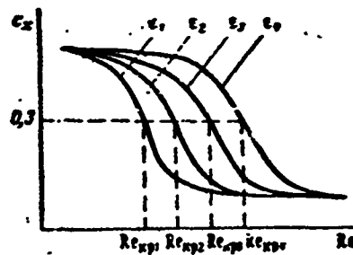
Figure 11.10. Effect of flow turbulence on sphere drag coefficient ( \epsilon_1 > \epsilon_2 > \epsilon_3 > \epsilon_4 )
