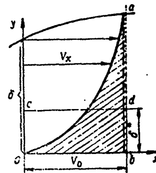
Figure 11.8. Geometric determination of displacement thickness
