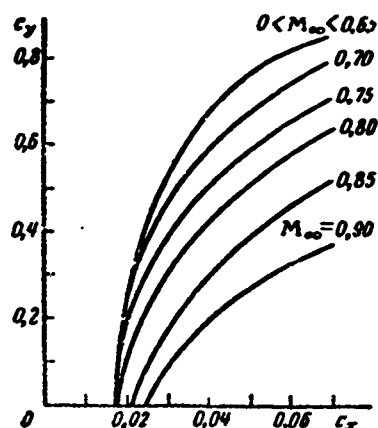
Figure 19.7. Wing polars for different M_\infty ( \lambda = 7 ; \bar{c} = 0.09 ; \chi_c = 0.52 rad).
