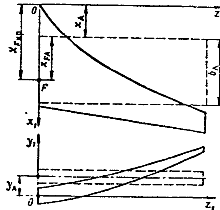
Figure 16.17. Mean aerodynamic chord ( b_A )
