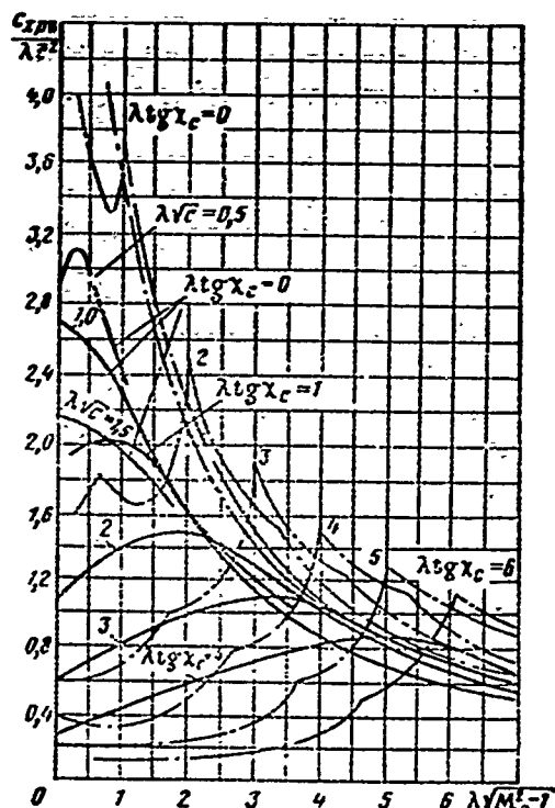
Figure 20.8. Graph for calculating wave drag of trapezoidal wing with rhombic profile ( \bar{x}_c = 0.5 ; \eta = 5 ).
