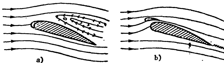
Figure 18.16. Flow around wing at high angle of attack with undeflected (a) and deflected (b) slats
