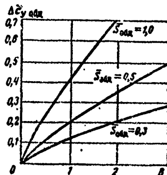
Figure 25.11. Effect of propeller slipstream over wing on lift force.
