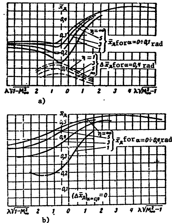
Figure 19.8. Plot for determining center of pressure coordinates of isolated wings with symmetric profile: a - straight ( \lambda \tan \chi_c = 0 ); b - swept ( \lambda \tan \chi_c = 3.0 ).
