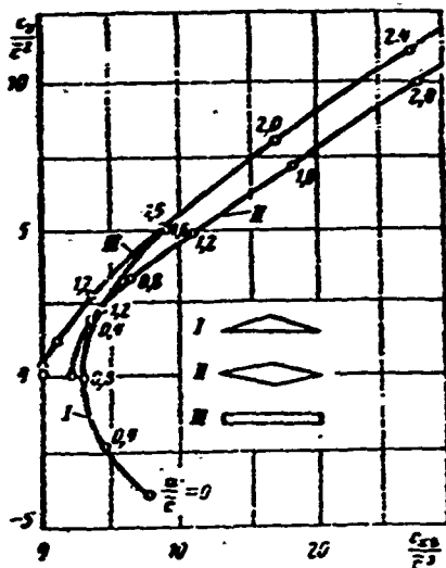
Figure 24.2. Polars of triangular and rhombic profiles and flat plate calculated using hypersonic gas flow theory.
