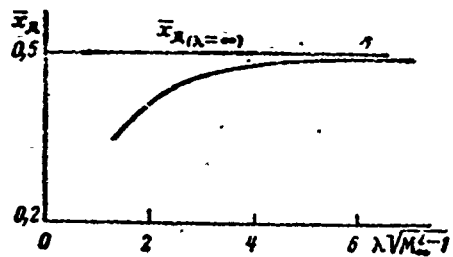
Figure 20.10. Influence of M_\infty and aspect ratio \lambda on center-of-pressure location.
