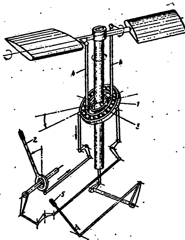
Figure 26.5. Tilt control: 1 - outer bearing ring; 2 - control stick; 3 - inner bearing ring; 4 - rods; 5 - collective pitch lever.
