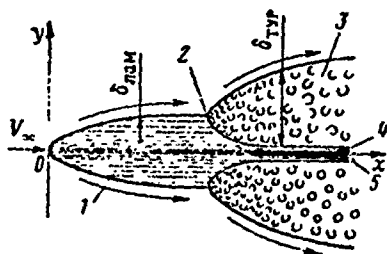
Figure 11.2. Boundary layer structure with transition from laminar to turbulent regime: 1 — laminar layer; 2 — transition point; 3 — turbulent layer; 4 — viscous sublayer; 5 — plate
