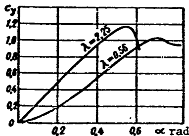
Figure 17.9. Curves c_y = f(\alpha) for wings of large and small aspect ratio.
