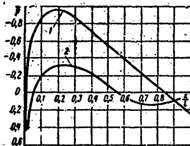
Figure 21.2. Pressure distribution along wing profile (1) and meridional section of body of revolution (2) for low M_\infty .
