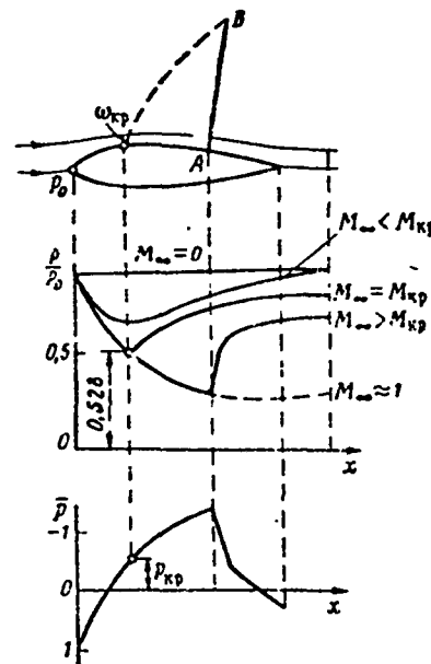
Figure 14.9. Pressure distribution over profile for different values of M_\infty
