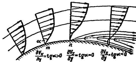
Figure 11.9. Schematic of flow with boundary layer separation
