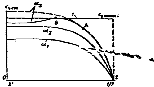
Figure 18.2. Change of spanwise c_y \sec distribution for rectangular planform wing with increase \alpha
