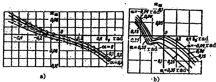
Figure 22.7. Curves of m_h = f(\delta_c, \alpha) and m_h = f(\delta_a, \alpha) : a - elevator and rudder; b - ailerons.
