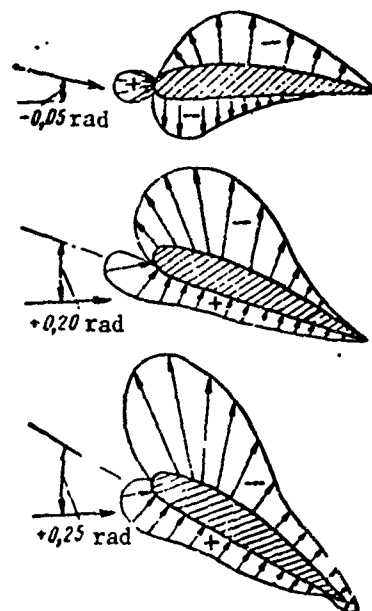
Figure 12.15. Vector diagrams of differential pressure distribution
