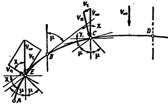
Figure 20.2. Supersonic flow past wing of arbitrary planform.
