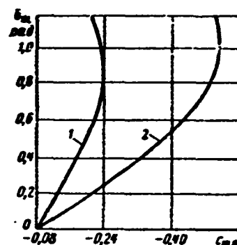
Figure 18.12. Effect of split flap deflection angle on wing moment characteristics:
