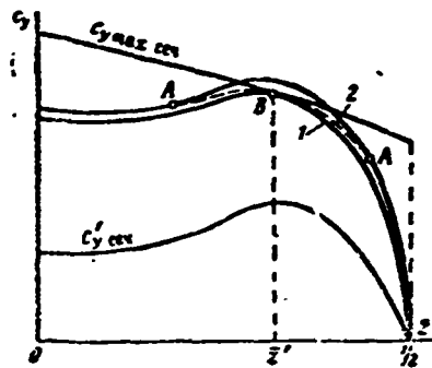
Figure 18.7. Illustration for calculation of wing c_{y \max} : 1 - variation of c_{y \sec} used in calculation under assumption that c_{y \sec} = c_{y \max \sec} at the section \bar{z}' ; 2 - actual variation of c_{y \sec} at the angle of attack for which c_{y \sec} = c_{y \max \sec} at section \bar{z}'
