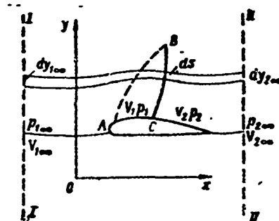
Figure 14.10. Scheme for calculating flow past wing profile in presence of normal shock
