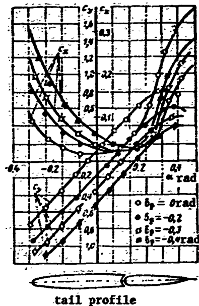
Figure 22.3. Aerodynamic characteristics of isolated tail.
