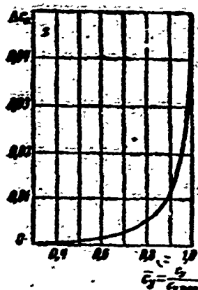
Figure 23.8. Curve for determining additional separation drag.
