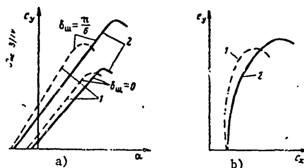
Figure 18.21. Change of wing aerodynamic characteristics under influence of ground effect:
