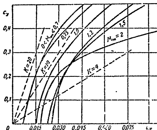
Figure 20.9. Wing polars for transonic and supersonic M_\infty range.
