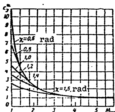
Figure 20.4. c_y^\alpha = f(M_\infty, \chi) for triangular wing calculated by the method of conical sections.
