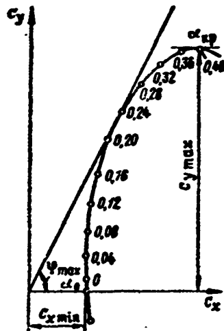
Figure 12.8. Type I polar
