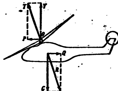
Figure 26.4. Forces acting on helicopter in flight.
