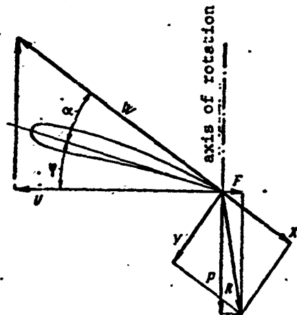
Figure 25.13. Prop blade operation in negative thrust regime.
