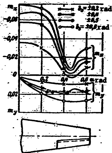
Figure 22.5. Curves of m_x = f(\delta_a, \alpha) and m_y = f(\delta_a, \alpha) for trapezoidal wing with conventional aileron.
