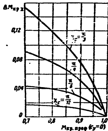
Figure 19.2. \Delta M_{cr\lambda} versus M_{cr, prof} (c_y = 0) and wing sweep angle along maximal thickness line.
