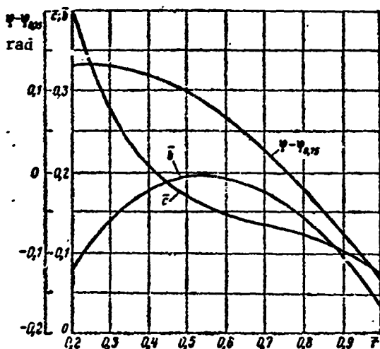
Figure 25.3. Variation of geometric characteristics along blade length.
