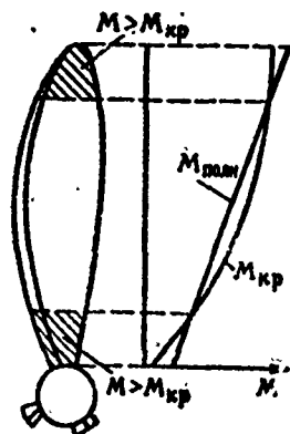
Figure 25.12. Regions of shock stall on blade.
