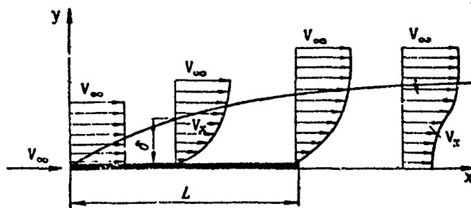
Figure 11.1. Schematic representation of boundary layer on a flat plate
