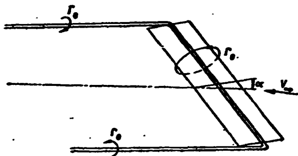
Figure 16.6. Simplest vortex scheme of finite-span wing
