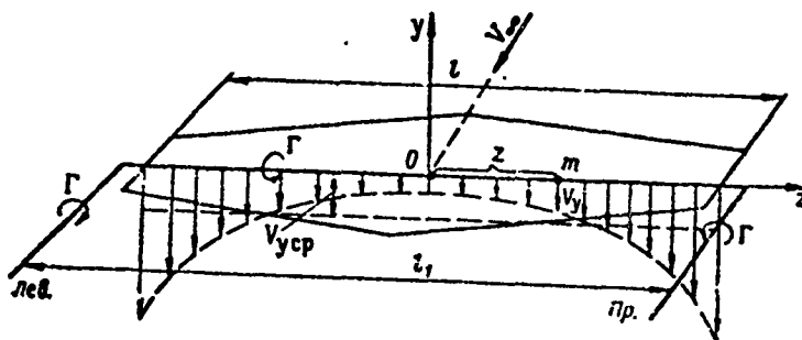
Figure 16.8. Illustration for calculating average downwash velocity
