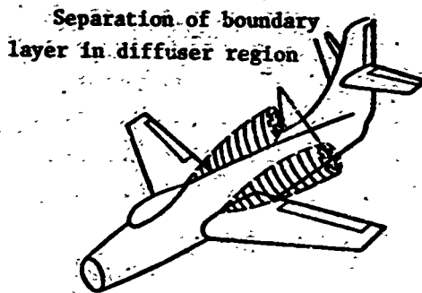
Figure 23.1. Increase of boundary layer thickness and premature flow separation at wing-fuselage junction.
