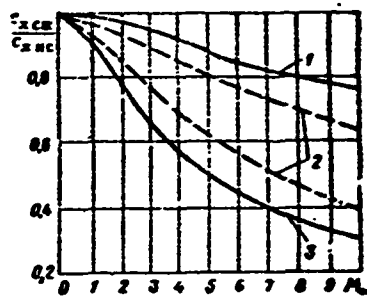
Figure 13.6. Flat plate drag coefficient versus M_\infty : 1 — \bar{x}_t = 1 ; 2 — 0 < \bar{x}_t < 1 ; 3 — \bar{x}_t = 0
