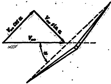
Figure 26.6. Main rotor angle of attack. Axial and transverse flow through rotor.
