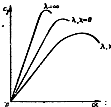
Figure 17.2. Relation c_y = f(\alpha) for wing of infinite span (profile) and also for straight and swept wings of finite span having different aspect ratio.
