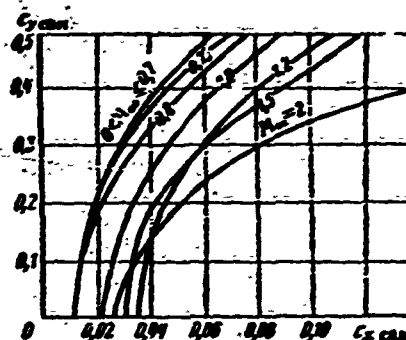
Figure 23.9. Supersonic airplane polars for different M_\infty .
