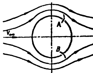
Figure 11.13. Separation-free flow past cylinder obtained by sucking boundary layer through slots A and B
