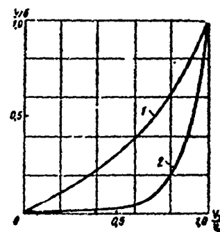
Figure 11.3. Comparison of velocity profiles in laminar and turbulent boundary layers: 1 — laminar layer; 2 — turbulent layer
