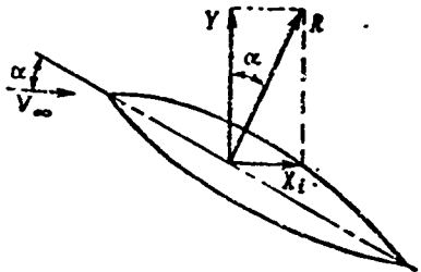
Figure 20.6. Illustration for determining induced drag of thin-profile wing in supersonic flow.
