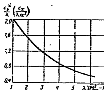
Figure 20.5. \frac{c_y^\alpha}{\lambda} \left( \frac{c_x}{\lambda^2} \right) as a function of \lambda \sqrt{M_\infty^2 - 1} for straight wing.
