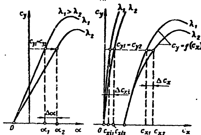
Figure 16.15. Conversion of wing aerodynamic characteristics to different aspect ratio
