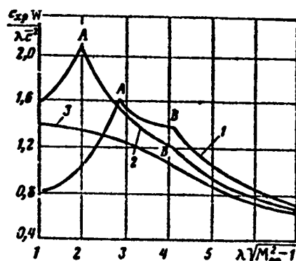
Figure 20.7. Influence of maximal profile thickness location on wave-profile drag: 1 - theoretical curve ( \bar{x}_c = 0.5 ); 2 - theoretical curve ( \bar{x}_c = 0.3 ); 3 - experimental curve ( \bar{x}_c = 0.5 ).
