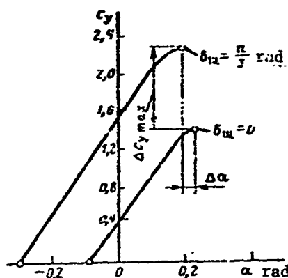
Figure 18.10. Wing lift coefficient c_y versus angle of attack \alpha for split flap deflections \delta_f = 0 and \delta_f = \pi/3 rad
