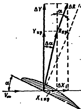
Figure 19.6. Illustration for constructing wing polar for M_{\infty} > M_{cr} .
