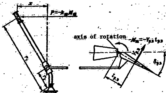
Figure 22.6. Hinge moment on control surface when stick is deflected.
