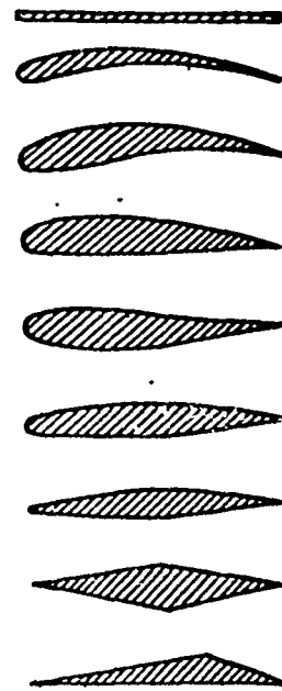
Figure 12.2. Aircraft profile forms (three lower profiles are supersonic)
