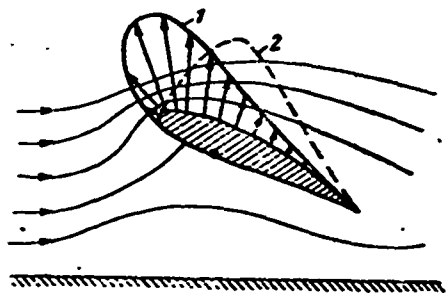
Figure 18.20. Influence of ground effect on pressure distribution over profile:
