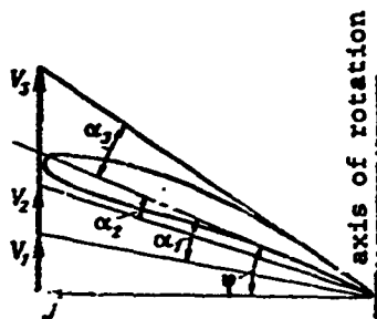
Figure 25.2. Effect of flight speed on blade section angle of attack.
