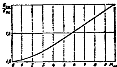
Figure 13.5. Turbulent boundary layer thickness versus M_\infty
