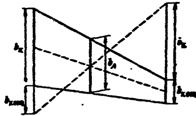
Figure 16.18. Geometric technique for finding MAC
