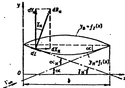
Figure 15.6. Supersonic flow past thin profile
