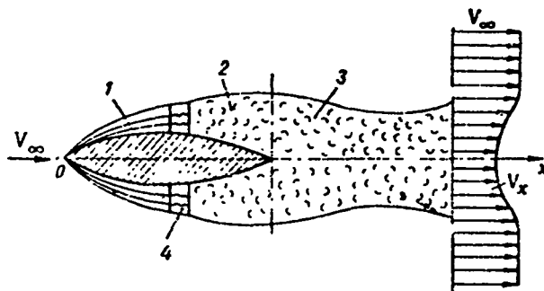
Figure 11.4. Schematic of viscous fluid flow past a body:
