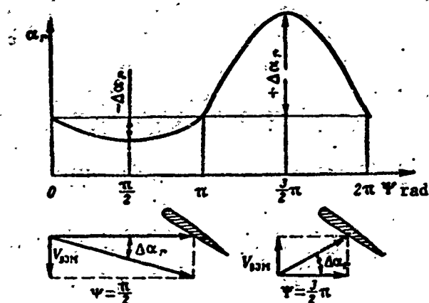
Figure 26.8. Azimuthal variation of blade section angle of attack because of blade flapping motion.
