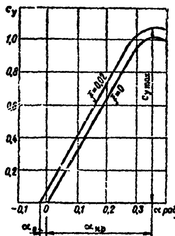
Figure 12.5. Aerodynamic coefficient c_y versus angle of attack \alpha
