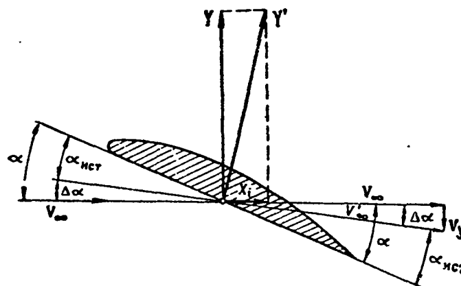
Figure 16.7. Velocity and force triangles for finite-span wing
