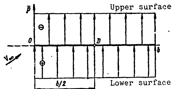
Figure 15.2. Pressure coefficient distribution over flat plate in supersonic flow
