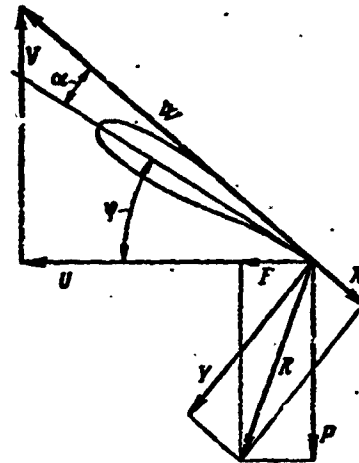
Figure 25.14. Prop blade operation in autorotation regime.
