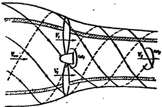
Figure 25.4. Illustrating ideal propeller analysis.
