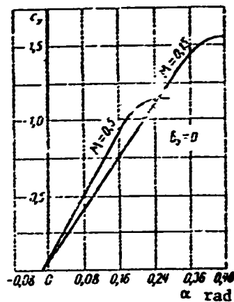
Figure 19.1. Wing lift coefficient c_y of An-24 airplane versus \alpha .
