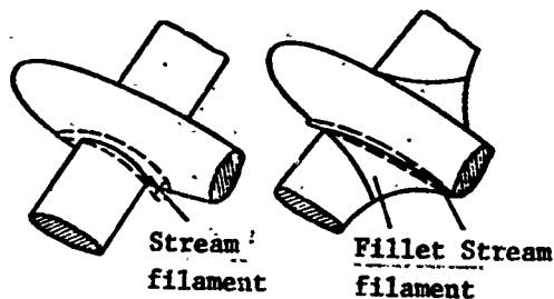
Figure 23.3. Diffuser effect at wing-fuselage junction.
