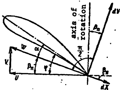
Figure 25.7. Forces acting on blade element.
