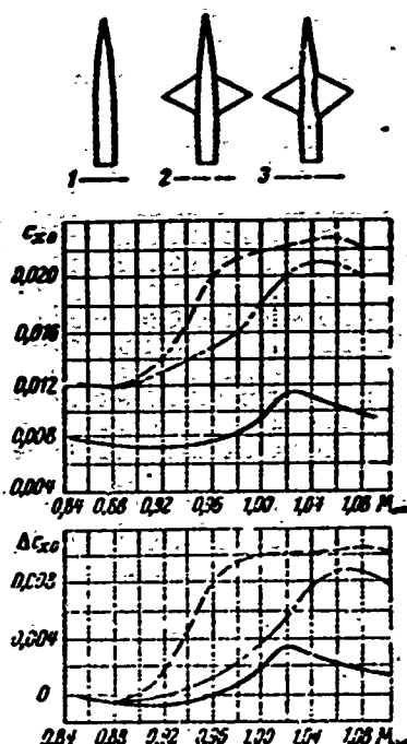
Figure 23.5. Effect of area rule application: 1 - fuselage alone; 2 - cylindrical fuselage plus wing; 3 - fuselage plus wing with use of "area rule".
