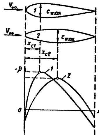
Figure 14.5. Effect of profile maximal thickness location on pressure distribution
