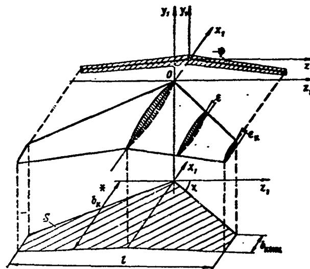
Figure 16.2. Wing geometric characteristics
