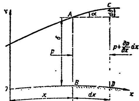
Figure 11.5. Derivation of integral relation for boundary layer in incompressible fluid
