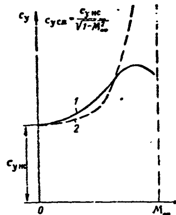
Figure 13.2. Comparison of actual values of c_y and those calculated using linear theory in the subsonic region: 1 — experimental values; 2 — theoretical values
