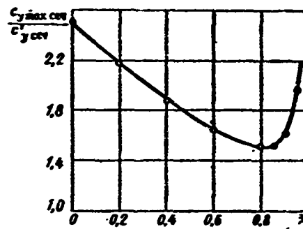
Figure 18.8. Curve of c_{y \max \sec} / c_{y \sec} = f(\bar{z})
