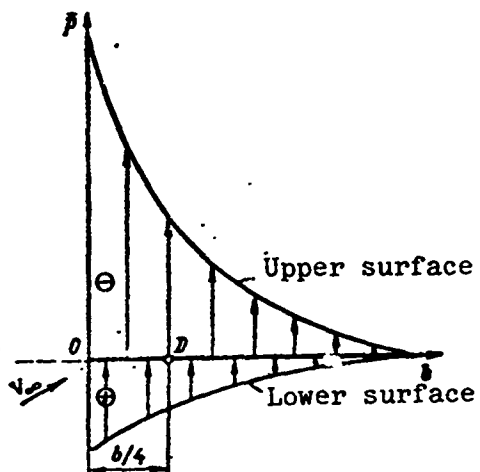
Figure 15.3. Pressure coefficient distribution over flat plate in subsonic flow
