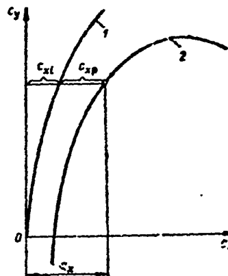
Figure 16.9. Induced drag parabola (1) and wing polar (2)
