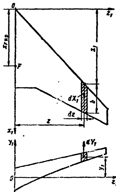
Figure 16.16. Determining wing longitudinal moment
