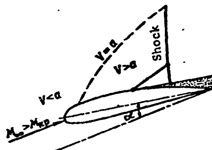
Figure 14.7. Flow past profile for M_{\infty} > M_{cr} with transition of laminar boundary layer into turbulent
