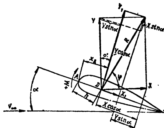
Figure 12.3. Components of total aerodynamic force in wing and body coordinate systems
