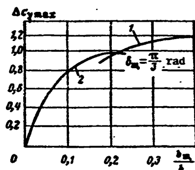
Figure 18.11. \Delta c_{y \max} versus relative split flap chord:
