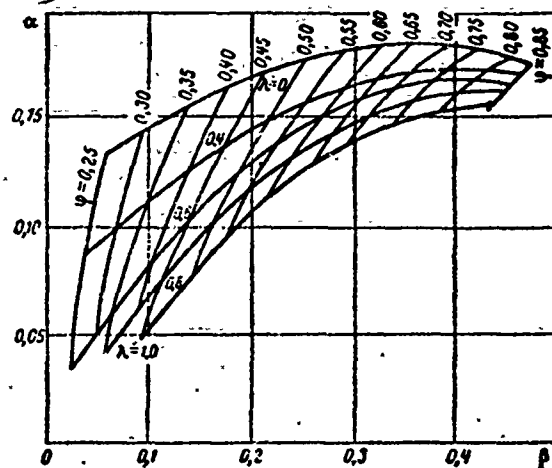
Figure 25.10. Propeller thrust characteristics.
