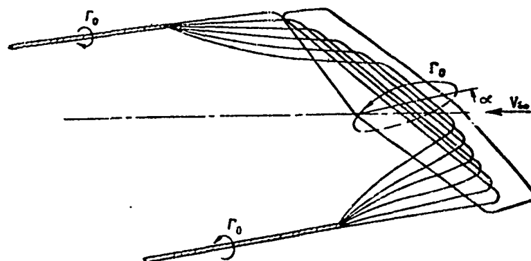
Figure 16.5. Transformation of vortex sheet into two trailing vortices
