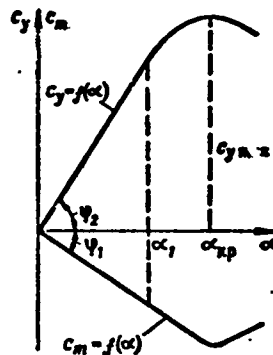
Figure 12.12. Aerodynamic coefficients c_y and c_m versus angle of attack \alpha for symmetric profile
