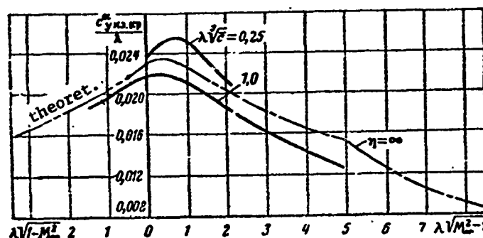
Figure 19.4. Curves for calculating lift coefficients of isolated wings ( \lambda \lg \chi_c = 3 )
