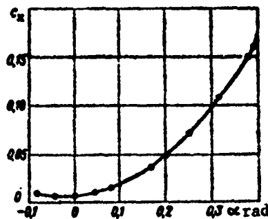
Figure 12.6. Aerodynamic coefficient c_x versus angle of attack \alpha
