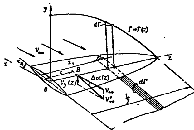
Figure 16.10. Definition of induced velocity at arbitrary wing section
