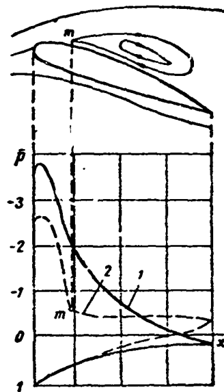
Figure 12.14. Flow over profile at stalling angle of attack: 1 — flow without separation; 2 — flow with separation (point m is point of boundary layer separation)
