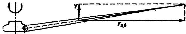
Figure 26.2. Blade equilibrium position.
