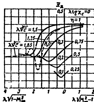
Figure 19.9. Effect of parameter \lambda\sqrt{1-M_\infty^2} on straight wing center of pressure location.
