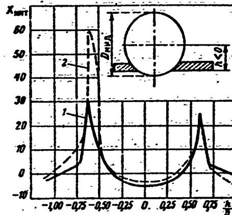
Figure 23.2. Effect of relative location of wing and fuselage on interference drag: 1 - for c_y = 0 ( c_{x \text{ air}} = c_{x \text{ min}} ); 2 - for c_y = 0.115 .
