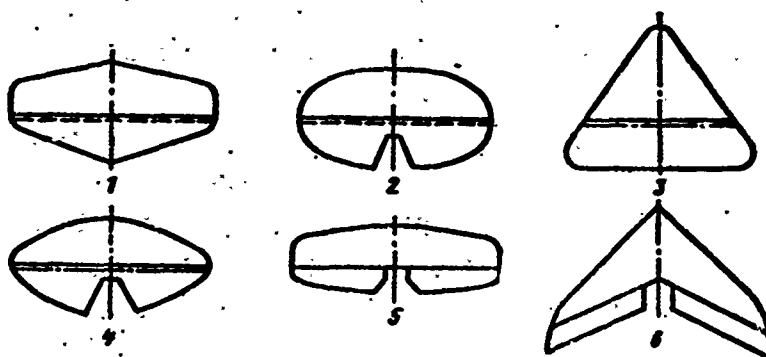
Figure 22.2. Characteristic horizontal tail planforms:
