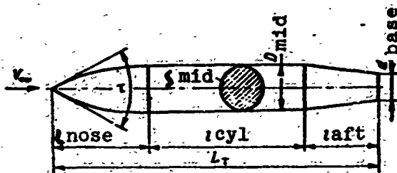
Figure 21.1. Basic geometric dimensions of body of revolution.
