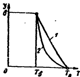
Figure 13.3. Temperature variation in boundary layer: 1 — laminar flow; 2 — turbulent flow
