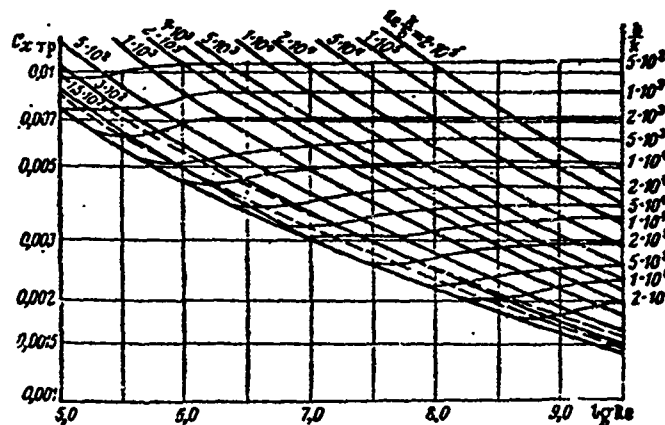
Figure 11.7. Frictional drag coefficient of rough plate as function of Re and surface roughness
