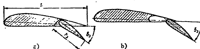
Figure 18.13. Trailing edge flaps: a - simple; b - extending
