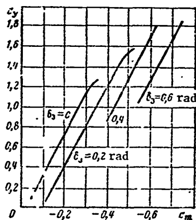
Figure 18.14. c_y versus c_m for wing with different trailing- edge flap deflections
