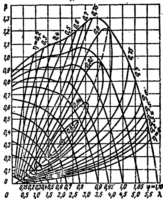
Figure 25.9. Propeller aerodynamic characteristics.
