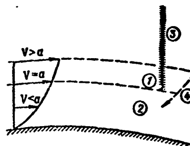
Figure 14.7. Flow past profile for M_{\infty} > M_{cr} with transition of laminar boundary layer into turbulent
