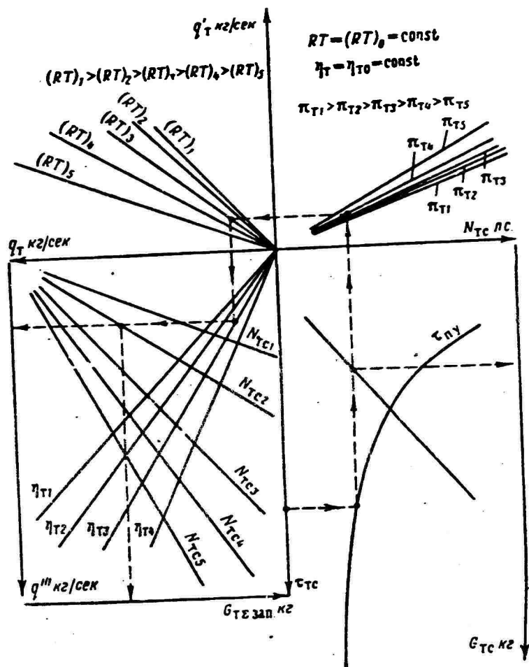
Figure 24. Nomogram for calculation of powder turbostarter. [Subscripts: TC = ts; 3an = st; ny = ss].
