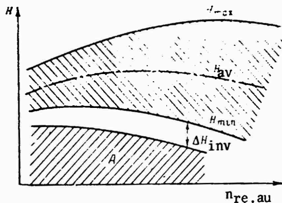
Figure 138. Limits of high-altitude starting for a series of engines: A -- region of reliable starting with confidence level \gamma = 0.99 .
