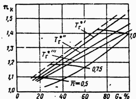
Figure 50. Air flow rate through compressor as function of change of gas temperature in front of turbine: T_g^{*'} > T_g^{*''} > T_g^{*'''} .
