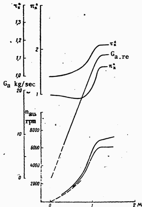
Figure 101. TJEА parameters as functions of Mach number in autorotation mode (top curve -- n_{phys.au} , bottom -- n_{re.au} ).
