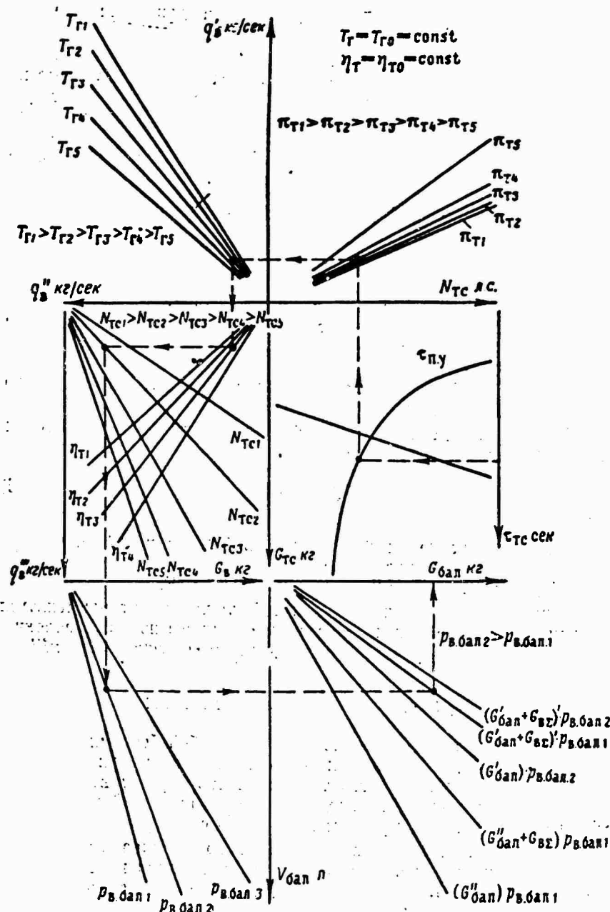
Figure 20. Nomogram for calculation of fuel-air starter. [Subscripts: Г = g; Б = a; Тс = ts; п.у = s.s; Б.бал = = a.cy; бал = cy].
