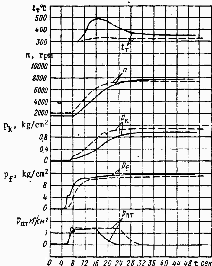
Figure 133. Change of parameters of VK-1A engine during starting process (continuous curves indicate changes of parameters at H = 6,000 \text{ m} and V_{\text{re}} = 320 \text{ km/hr} , and the broken curves -- H = 6,000 \text{ m} and V_{\text{re}} = 420 \text{ km/hr} ).
