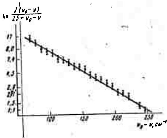
Fig. 30. Dependence of \log_e [J(v)/(25 + \nu_0 - v)] on frequency for the same mixture as Fig. 29 and \tau = 2 \text{ msec} .
