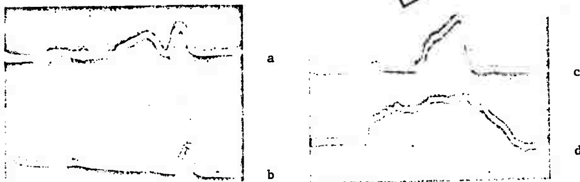
Fig. 4 Oscillograms of individual v-r transitions ( \tau_{\text{pump}} \approx 8 \mu\text{sec} ): a -- unresolved transitions P_{3-2}(8) and P_{2-1}(11) ; b -- P_{2-1}(11) ; c -- P_{3-2}(8) ; d -- total laser pulse. Total scan time 60 \mu sec.
