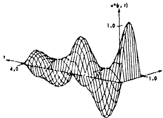
(c) THE OPTIMAL TRAJECTORY
