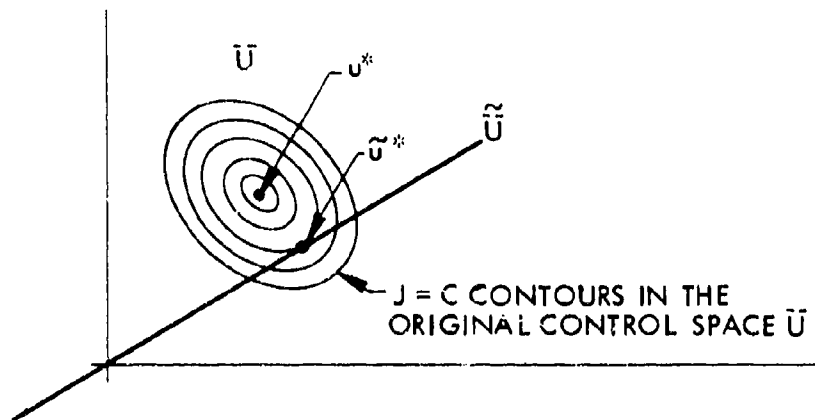
Figure 4.6. Minimization on a subspace
