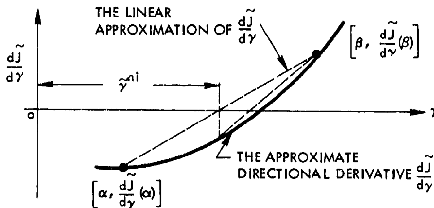
Figure 4.3. The regula falsi iterator
