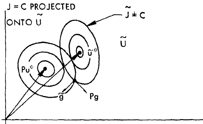
Figure 4.5. Constant cost contours
