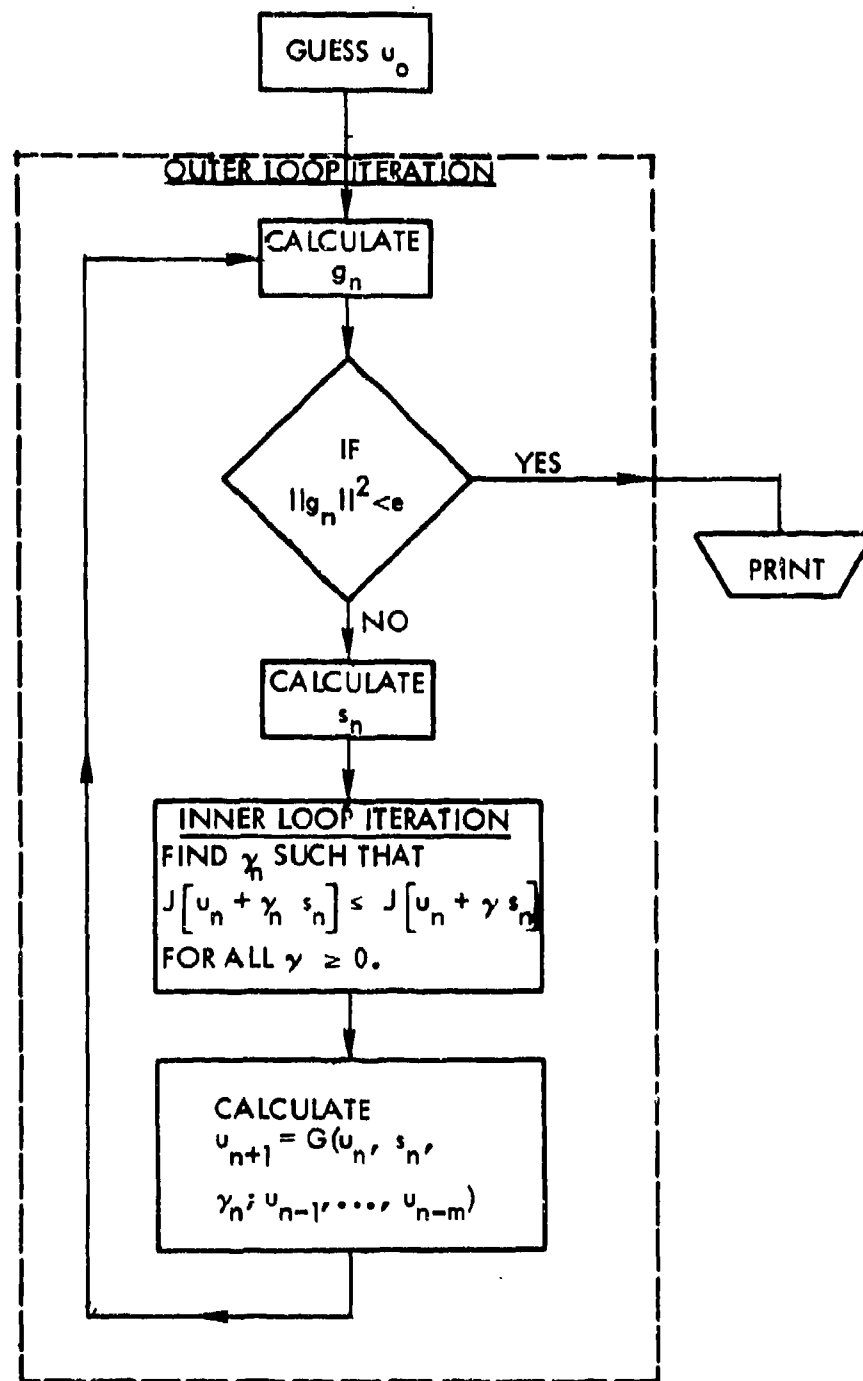
Figure 3.1. The gradient method algorithm
