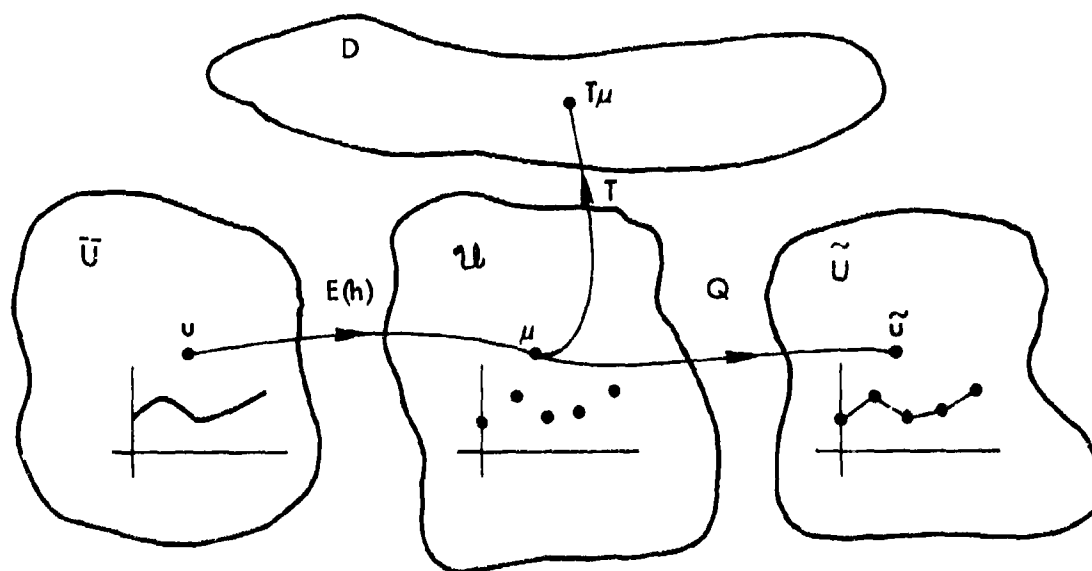
Figure 4.1. The discretization process
