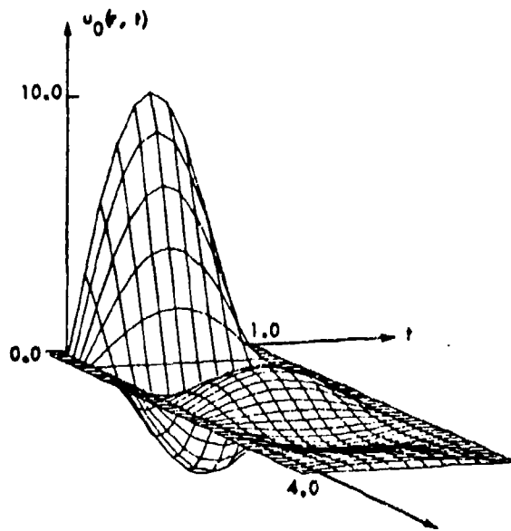
(a) THE GUESSED INITIAL CONTROL
