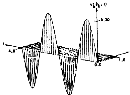
(b) THE APPROXIMATE OPTIMAL BOUNDARY CONTROL
