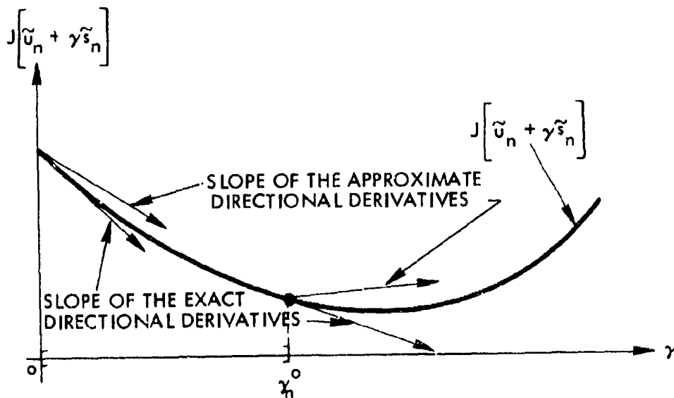
Figure 4.2. Cubic interpolation
