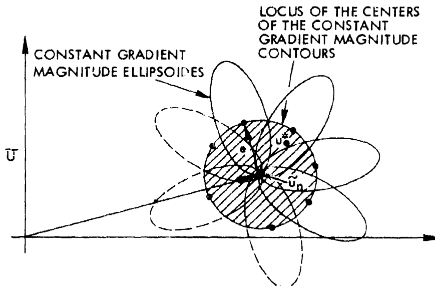
Figure 4.4. Geometrical interpretation of the optimal control error
