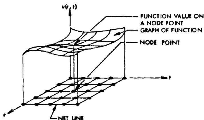
Figure A-1. The node N of the net \mathcal{N}
