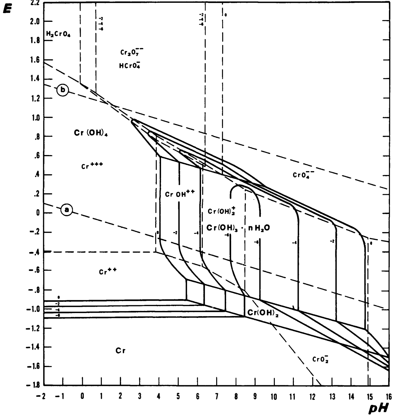
FIGURE 47. Pourbaix diagram for Chromium. Adapted from Pourbaix, 1974.
