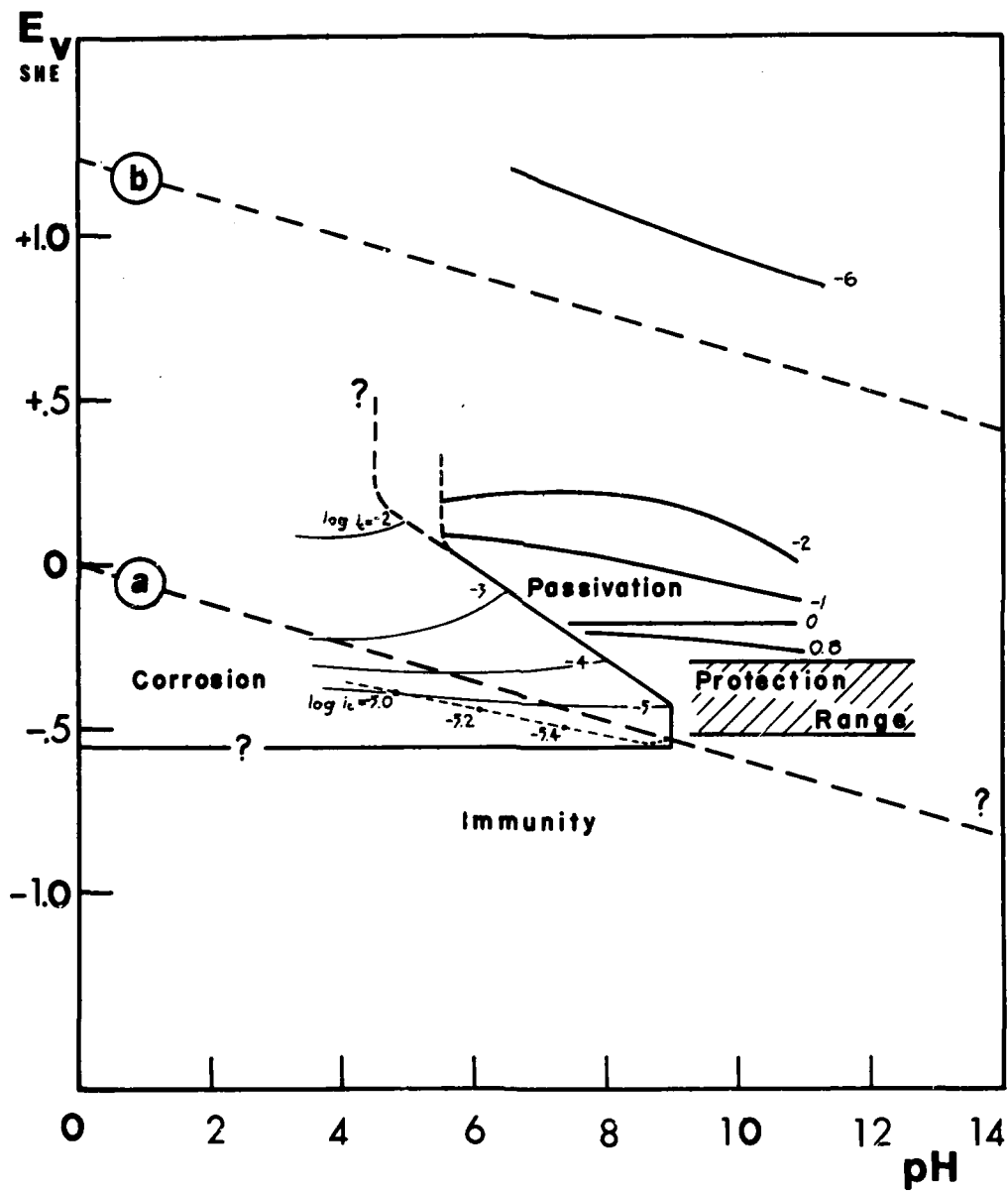
FIGURE 40: Experimental Pourbaix Diagram for Binary Fe-Cr Alloy Containing 2.0% Chromium. Rupture Potential and Protection Potential Range are Superimposed.
