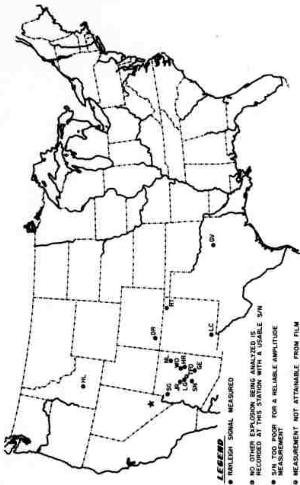
Figure 6. Location of stations recording long period seismic energy from the nuclear explosion AUK.
