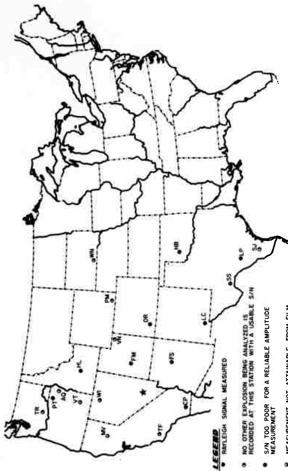
Figure 31. Location of stations recording long period seismic energy from the nuclear explosion AARDVARK.
