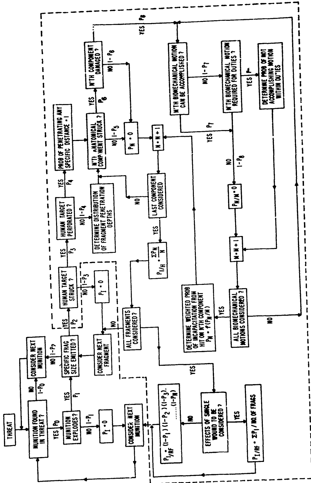
Figure 8. Logic diagram for probabilistic model of incapacitation by kinetic energy missiles.
