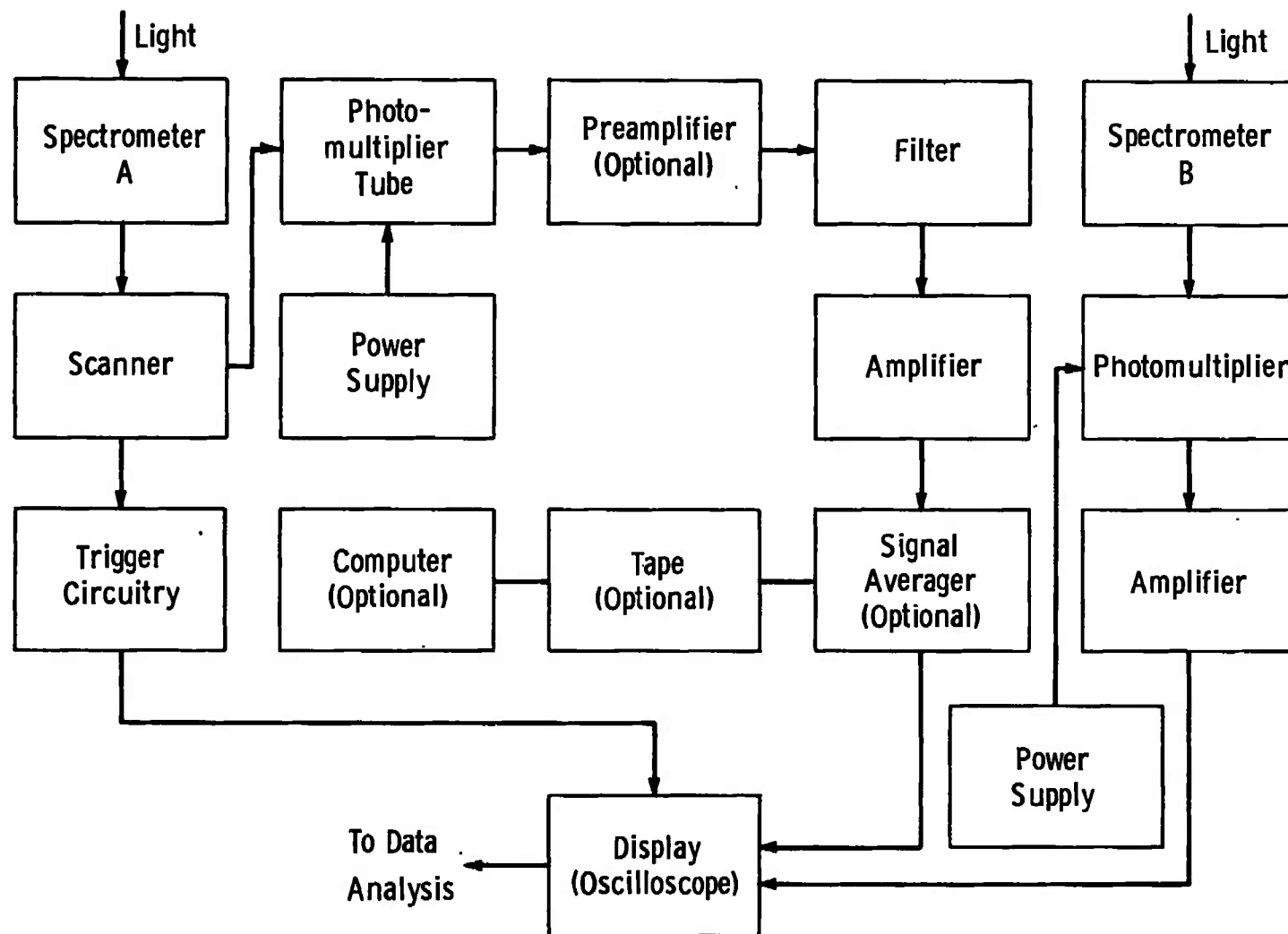
Fig. 13 Photoelectric Scanning
