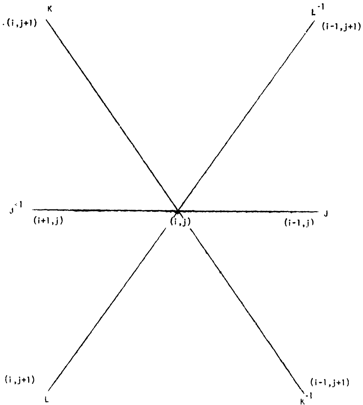
Figure 9. Representation of the State Component System.
