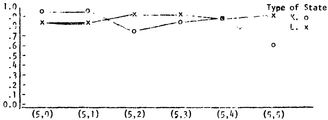
Figure 7. The Estimates of P for the Second Power Position for Each Type of State as a Function of Initial State.
