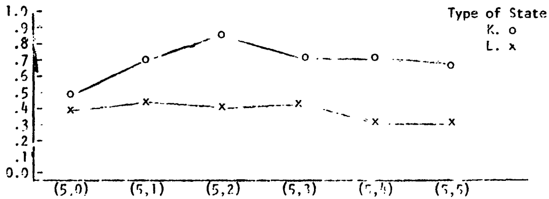
Figure 6. The Estimates of P for the First Power Position for Each Type of State as a Function of Initial State.
