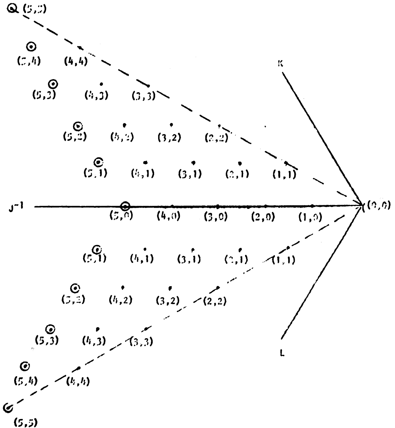
Figure 10. Reduced Co-ordinate System for the Representation of State Vectors.
