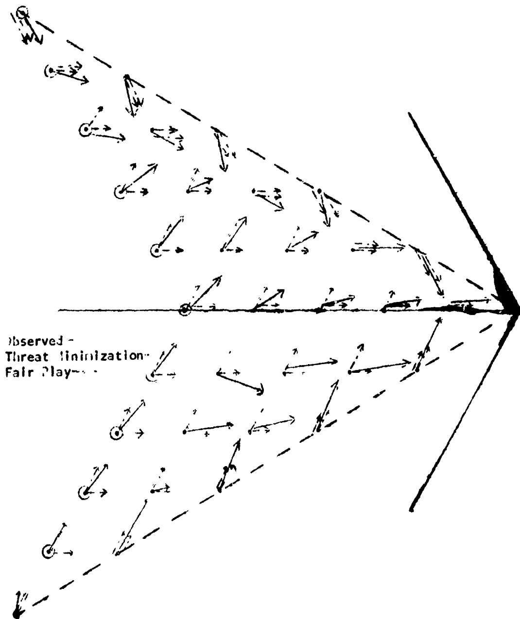
Figure 11. The Mean Observed Directional Vectors and the Directional Vectors for the Fair Play and Threat Minimization Strategies.
