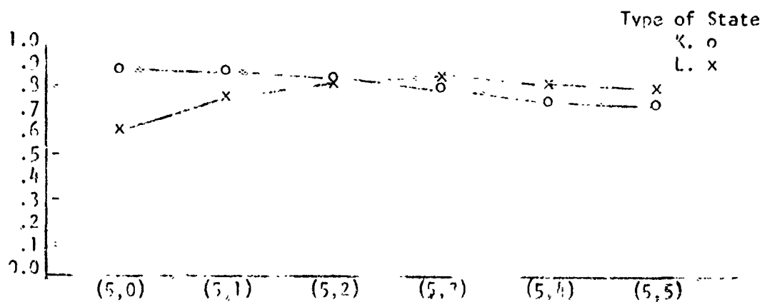
Figure 8. The Estimates of P for the Third Power Position for Each Type of State as a Function of Initial State.
