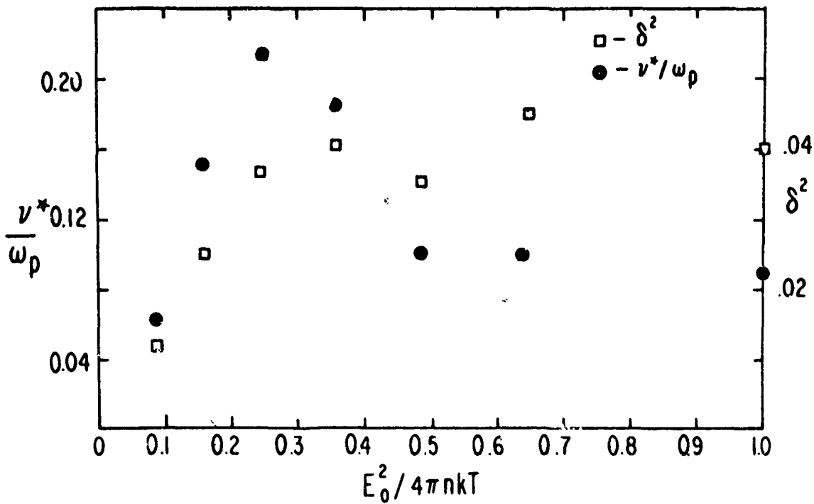
Fig. 4. Variation of the normalized anomalous collision frequency (v^*/\omega_p) with the electric field parameter (E_0^2/4\pi n k T) in the computer simulation experiment.
