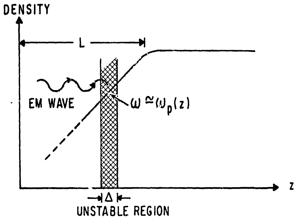
Fig. 5. Schematic of the Gekker-Sizukhin experiment.
