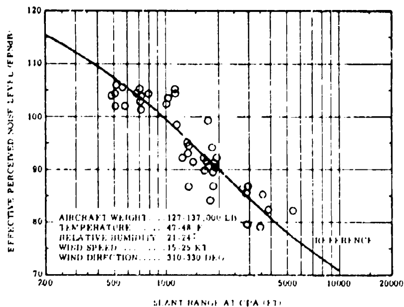
Figure A-58. Noise Levels as a Function of Slant Range for Profile A51, 727 Aircraft
