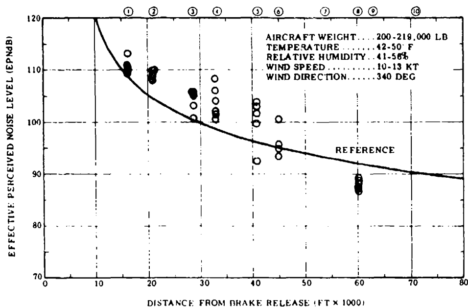
Figure C-1. Takeoff Noise Levels for Profile T1, 707-320B Aircraft
