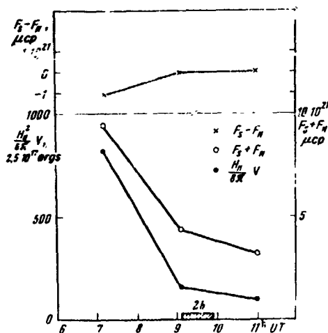
Figure 16. Behavior of the Magnetic Energy of the Longitudinal Field H_{\parallel}^2/8\pi of the Total Flux F_S + F_N and the Resulting Flux F_S - F_N with Time for the 22 June 1962 Flare
