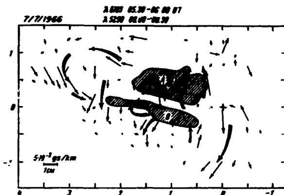
Figure 28. Map of Transversal Fields j_{\perp} for July 7 and Location on It of Clouds of the A and B Proton Flares (hatched)
