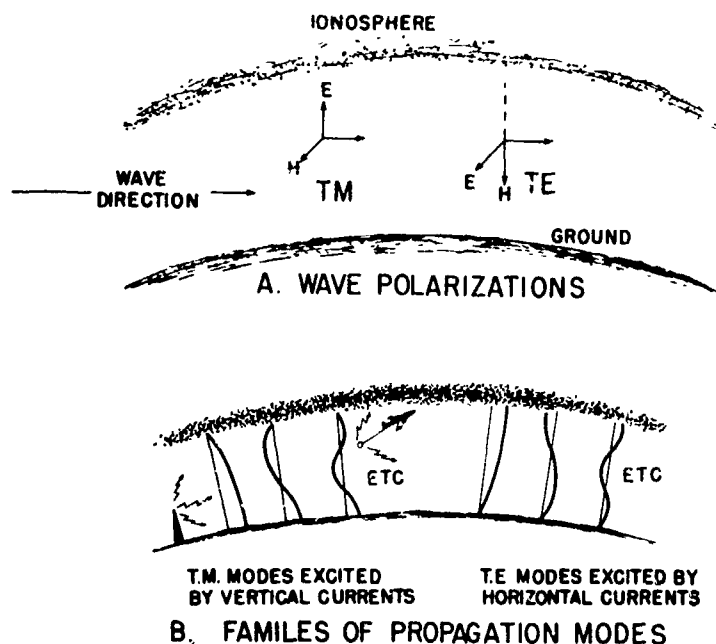
Figure 1. Characteristics of TM and TE Waves
