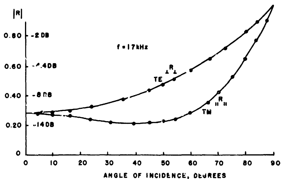
Figure 5. Ionospheric Reflection Coefficients— Severely Disturbed Daytime Ionosphere
