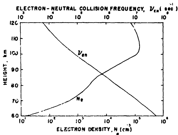
Figure 2. Model of a Normal Daytime Ionosphere
