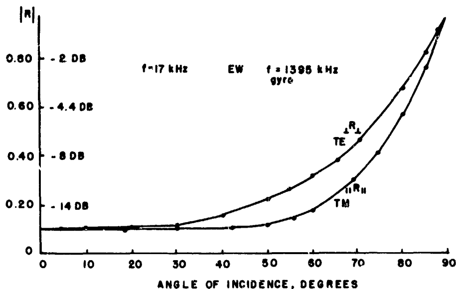
Figure 3. Ionospheric reflection Coefficients—Normal Distorted Ionosphere
