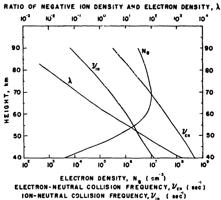
Figure 4. Model of a Severely Disturbed Daytime Ionosphere
