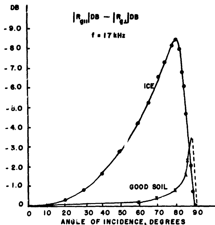
Figure 6. Relative Attenuation of TM and TE Waves Upon Reflection From the Earth
