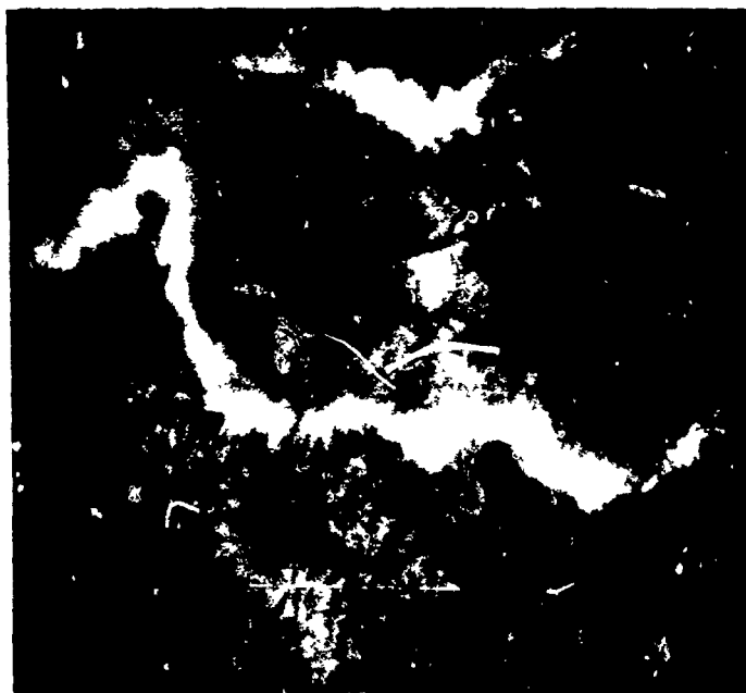
Figure 13. A Vacuum Tower Telescope Photograph of the Class 2 Flare of 14 May 1971. Notice the thin, dark loops connecting the two bright flare ribbons. Photo courtesy of R. B. Dunn
