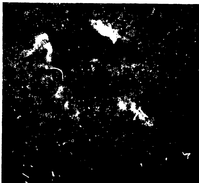
Figure 14. Photograph Showing the Same Loops as the Previous Figure Except That This Image in the Red Wing of H\alpha Shows the Downward-Moving Material in the Loops. The bright flare ribbons may be caused by the energy released when the falling material strikes the chromosphere. Photo courtesy of R. B. Dunn
