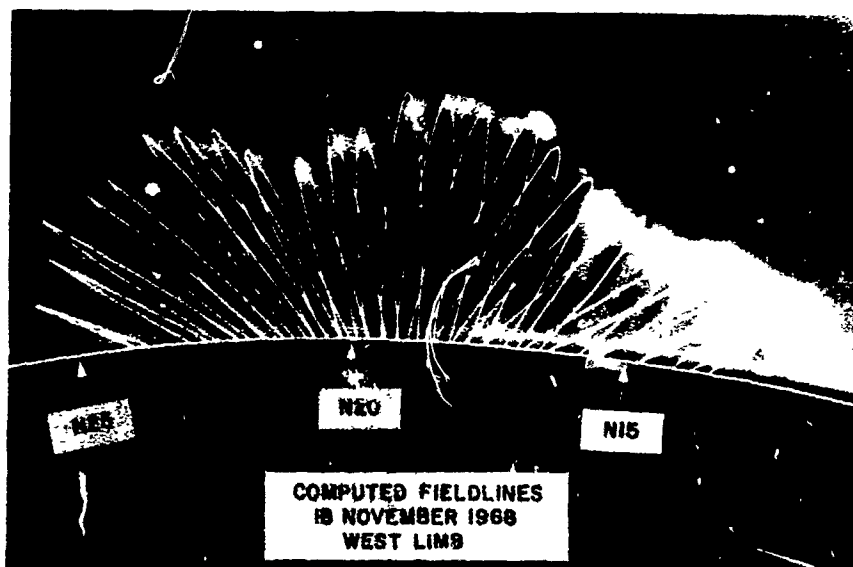
Figure 11. Comparison Between the Computed Fieldlines for the 18 November 1968, X-Ray Flare and Loops and the Green-Line Corona as Photographed by H. L. DeMastus at Sacramento Peak
