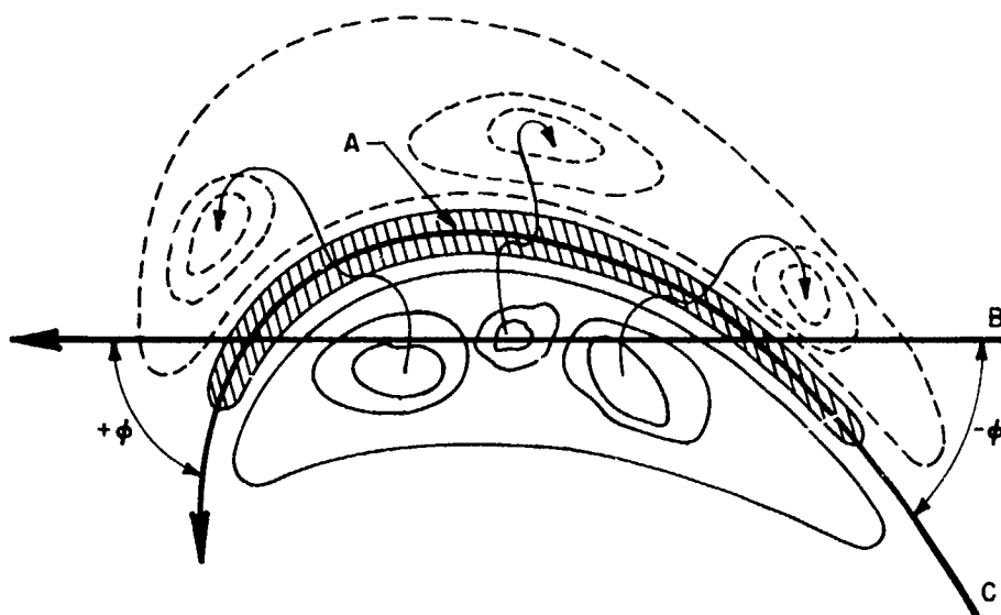
Figure 1. Lines of Force (with dips) Passing Through a Quiescent Filament. The straight arrow is a hypothetical line-of-sight for magnetic observations made on the limb
