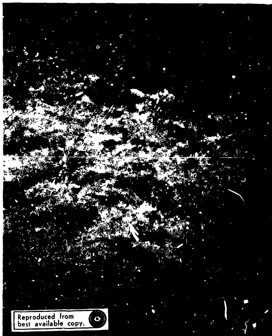
Figure 9. An Unusual Surge, or Veil of Surges, as Photographed in H\alpha . This photograph was taken on 25 July 1971 at Sacramento Peak by J. -R. Roy
