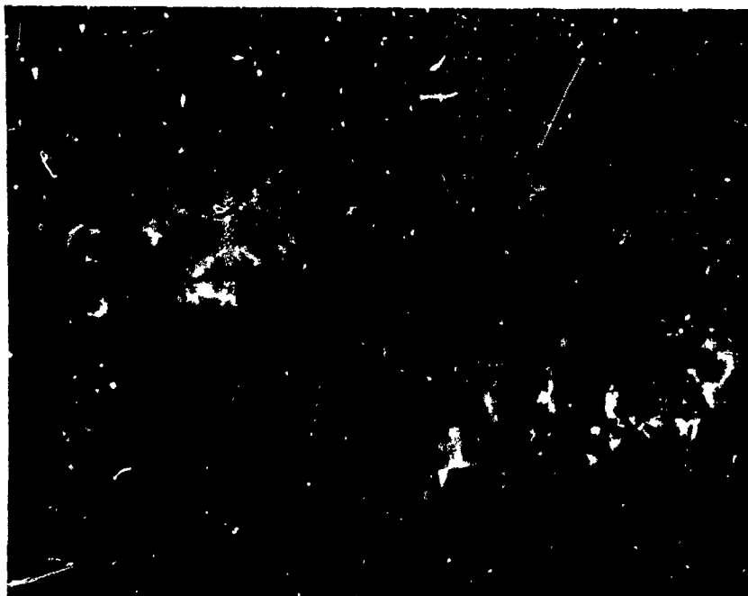
Figure 4. A Peculiar Filament Photographed on the Disk on 1967 July 29. Spectroheliogram in H\alpha from the Mount Wilson Observatory
