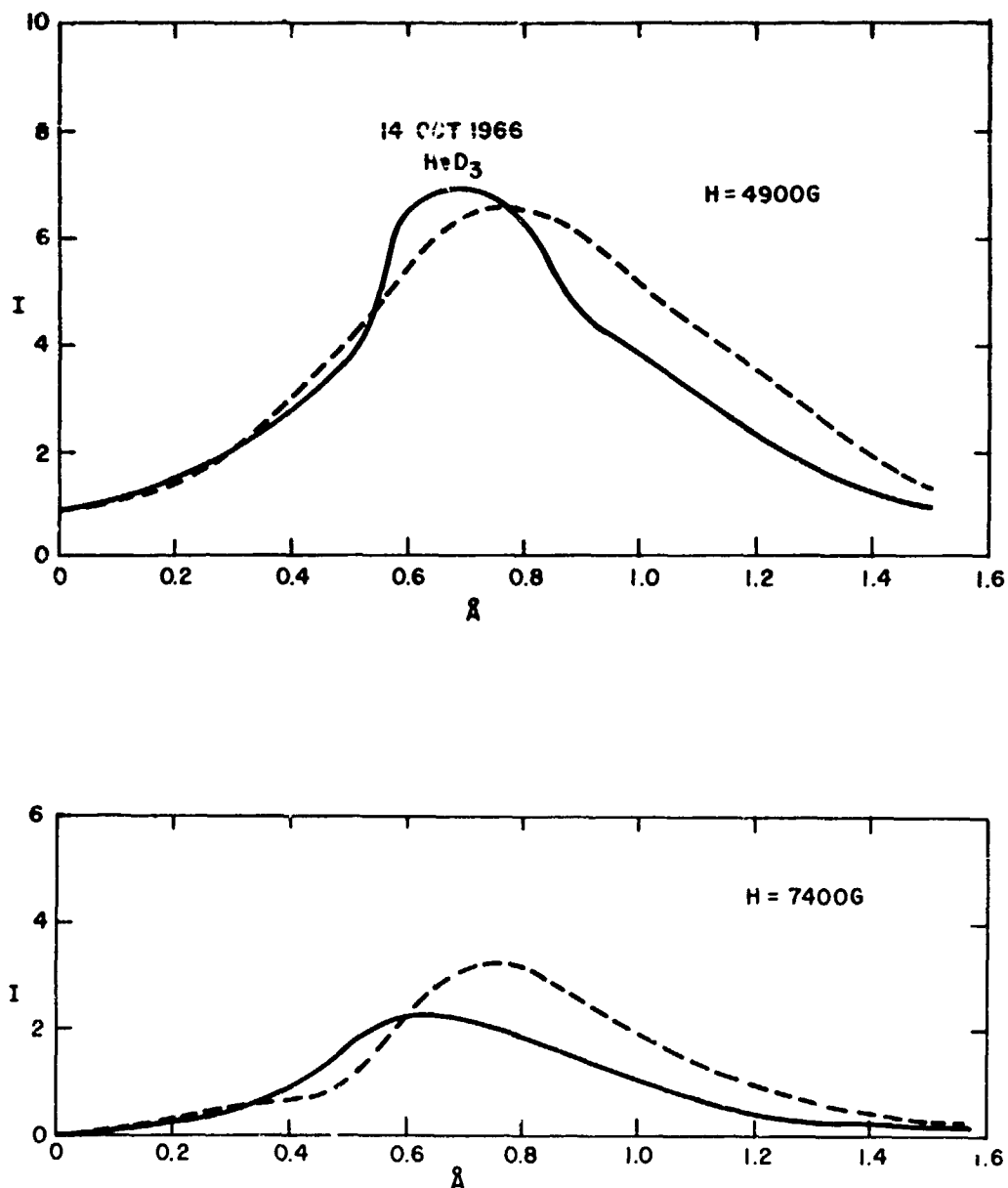
Figure 7. Microphotometer Tracings of Dash Profiles Made at the Pulkovo Observatory. (Top) Profiles from top 12 arcsec of a dash. (Bottom) Profiles from bottom 12 arcsec of the same dash. Dashed lines denote profiles corresponding to the lower image. Solid lines denote profiles corresponding to the upper image
