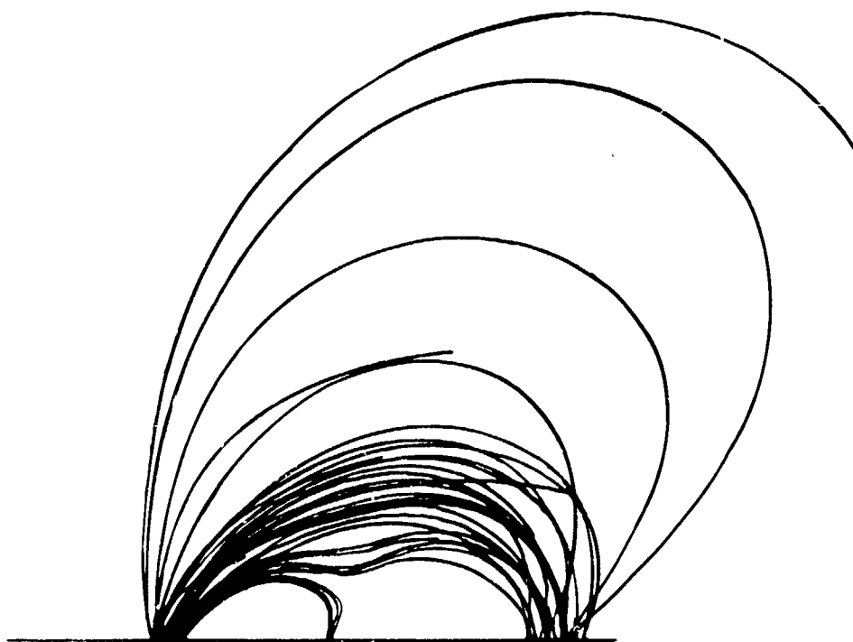
Figure 2. Computed Current-Free Fieldlines Capable of Supporting a Prominence
