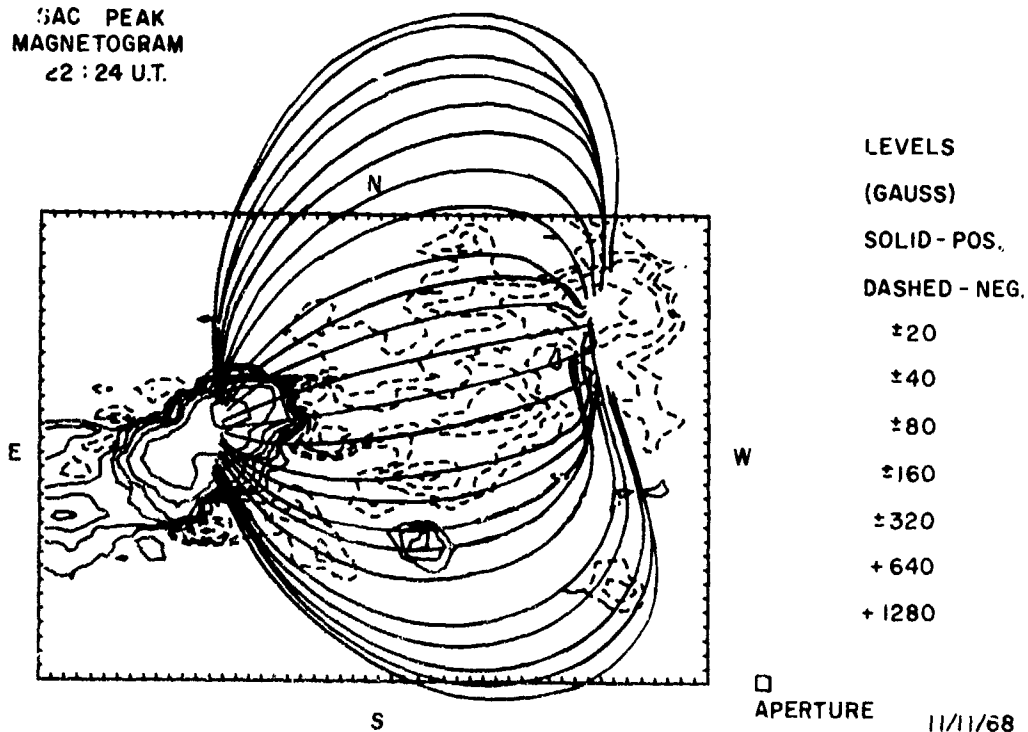
Figure 12. The Computed Fieldlines of the Previous Figure as Seen in Projection on the Disk
