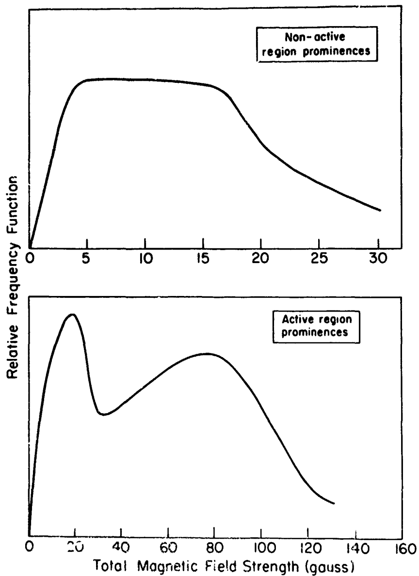
Figure 3. Frequency of Occurrence of Prominence Magnetic Field Intensities After Transformation of the Observations by the Assumption That the Field in the Prominences has No Preferred Direction
