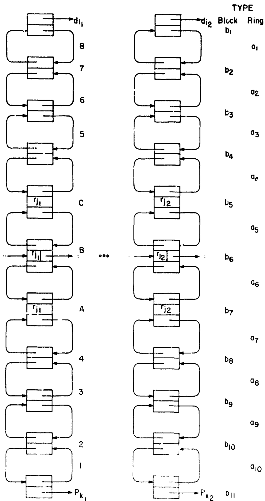
Figure 3-11. Storage Structure Model for all k_1^0 = 1
