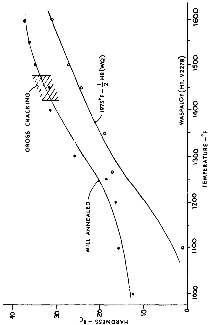
FIGURE 24 - ON-HEATING HARDENING RESPONSE OF WASPALOY (HT. V2278) FOR THE MILL ANNEALED AND SOLUTIONED (1975 ^{\circ}F -1/2 HR, WQ) CONDITIONS.
