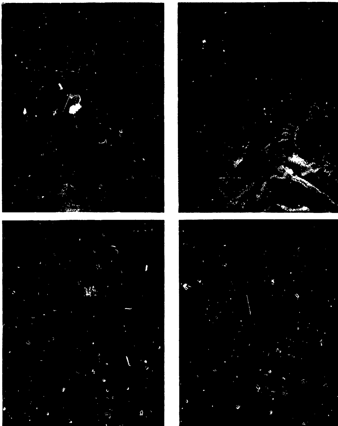
FIGURE 15 - SCANNING ELECTRON MICROGRAPHS SHOWING DIFFERENCES IN FRACTURE FACE FEATURES DUE TO HEAT TREATING IN AN AIR ATMOSPHERE (LEFT) AND A VACUUM ENVIRONMENT (RIGHT). X1000
