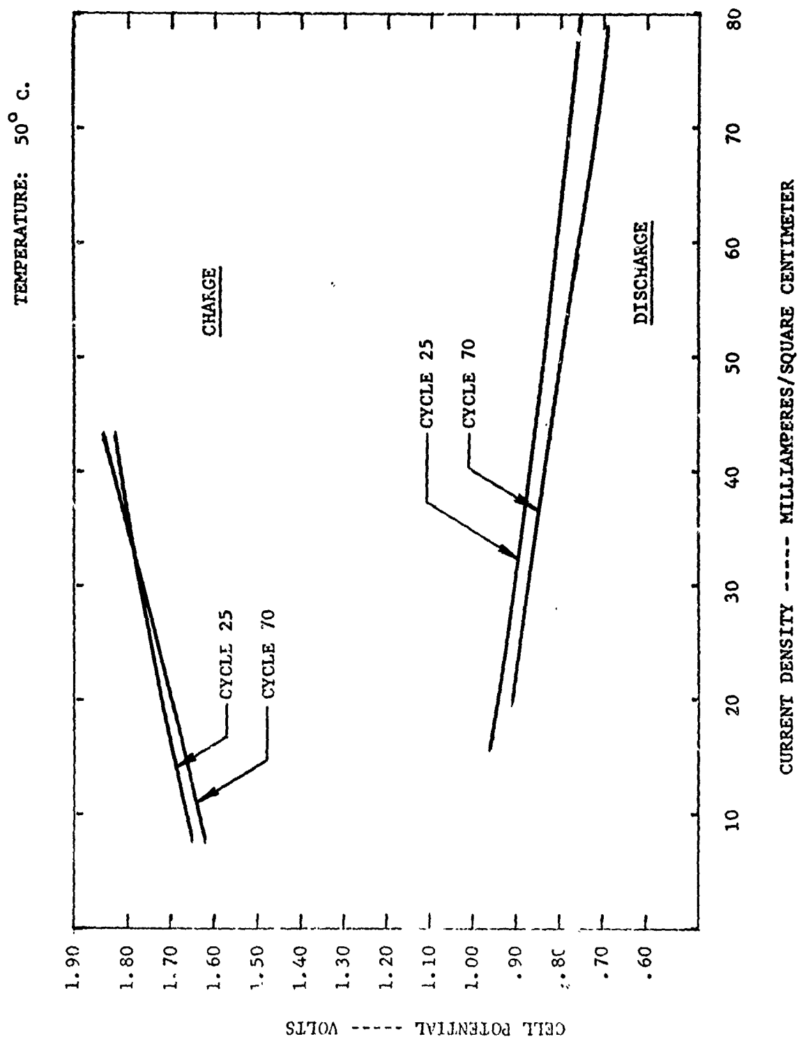
FIGURE 32. CELL NO. 4058-18 POLARIZATION SCANS
