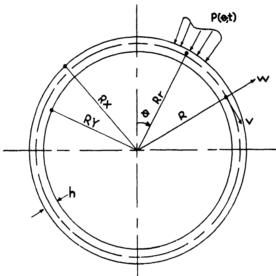
FIGURE 1-A. SHELL GEOMETRY
