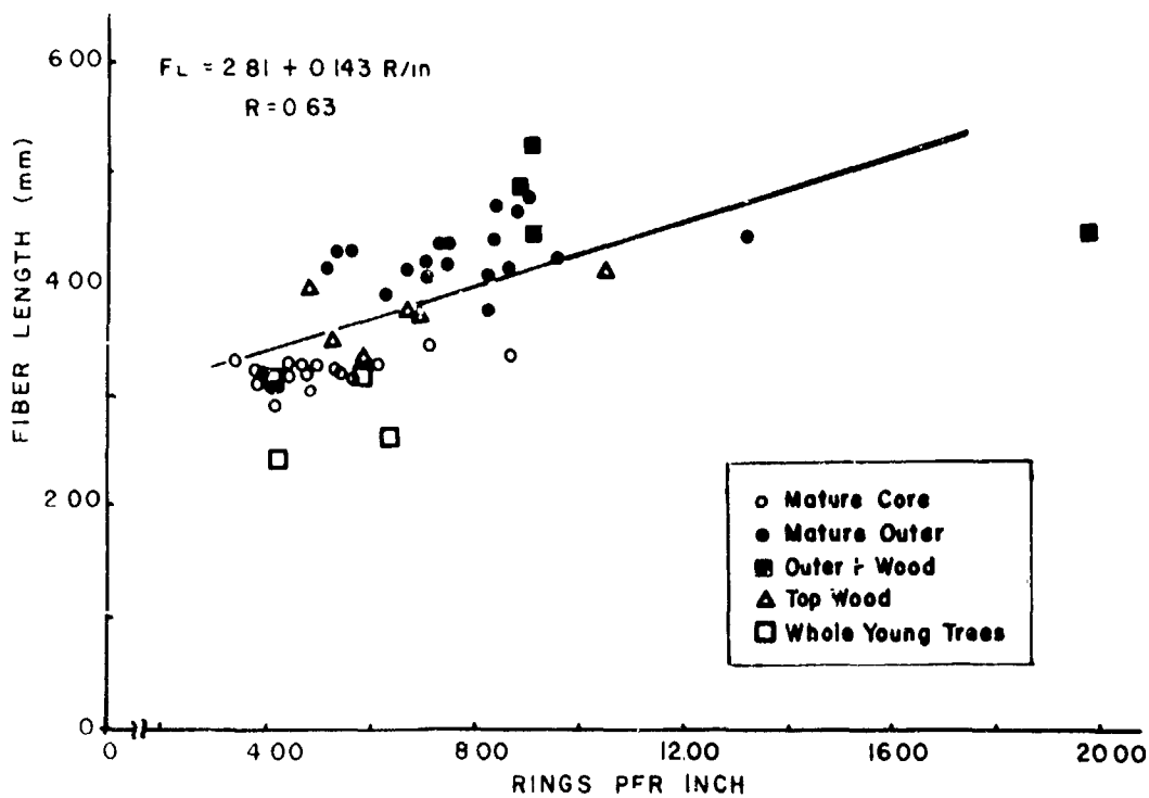
Figure 18.--The relationship of average rings per inch and fiber length for 52 samples of wood from 23 loblolly pine trees.
