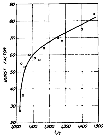
Figure 4.--Influence of L/T ratio on bursting strength for handsheets made from unbeaten, unbleached kraft pulps from 12 western U.S. softwood species.
