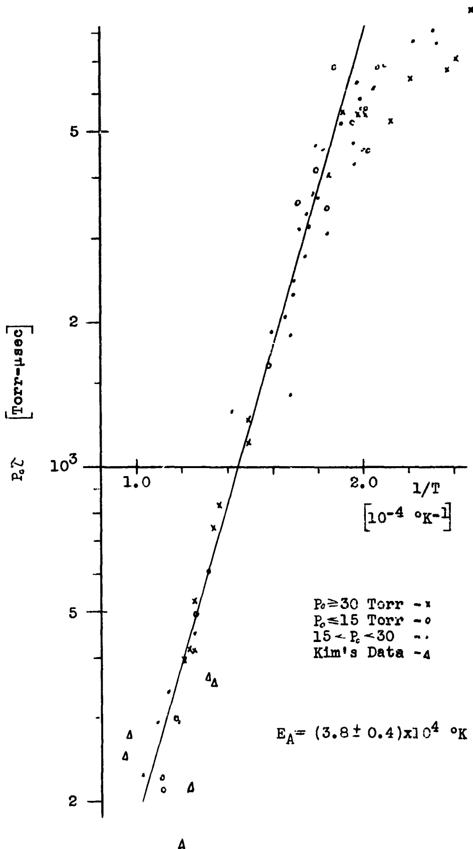
Figure 13. Plot of \log P_0 \tau against 1/T for Mercury.
