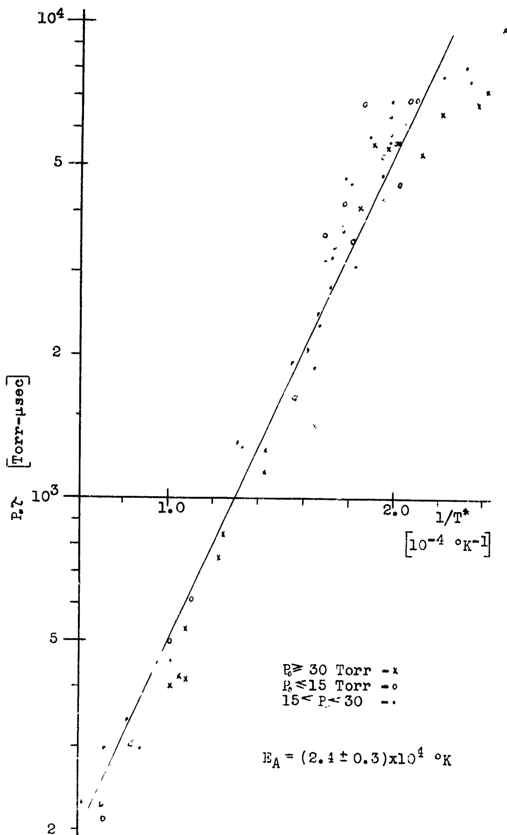
Figure 11. Plot of \log P_0 \tau against 1/T^* for Mercury.
