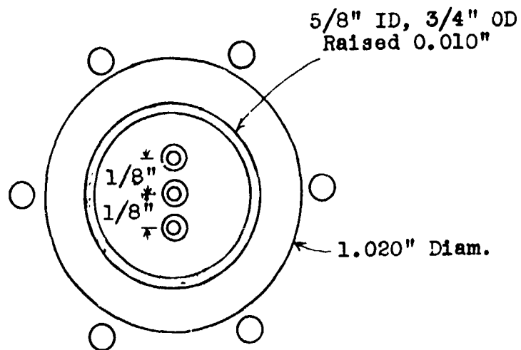
B. Front View of Tube Wall (Double Actual Size)
