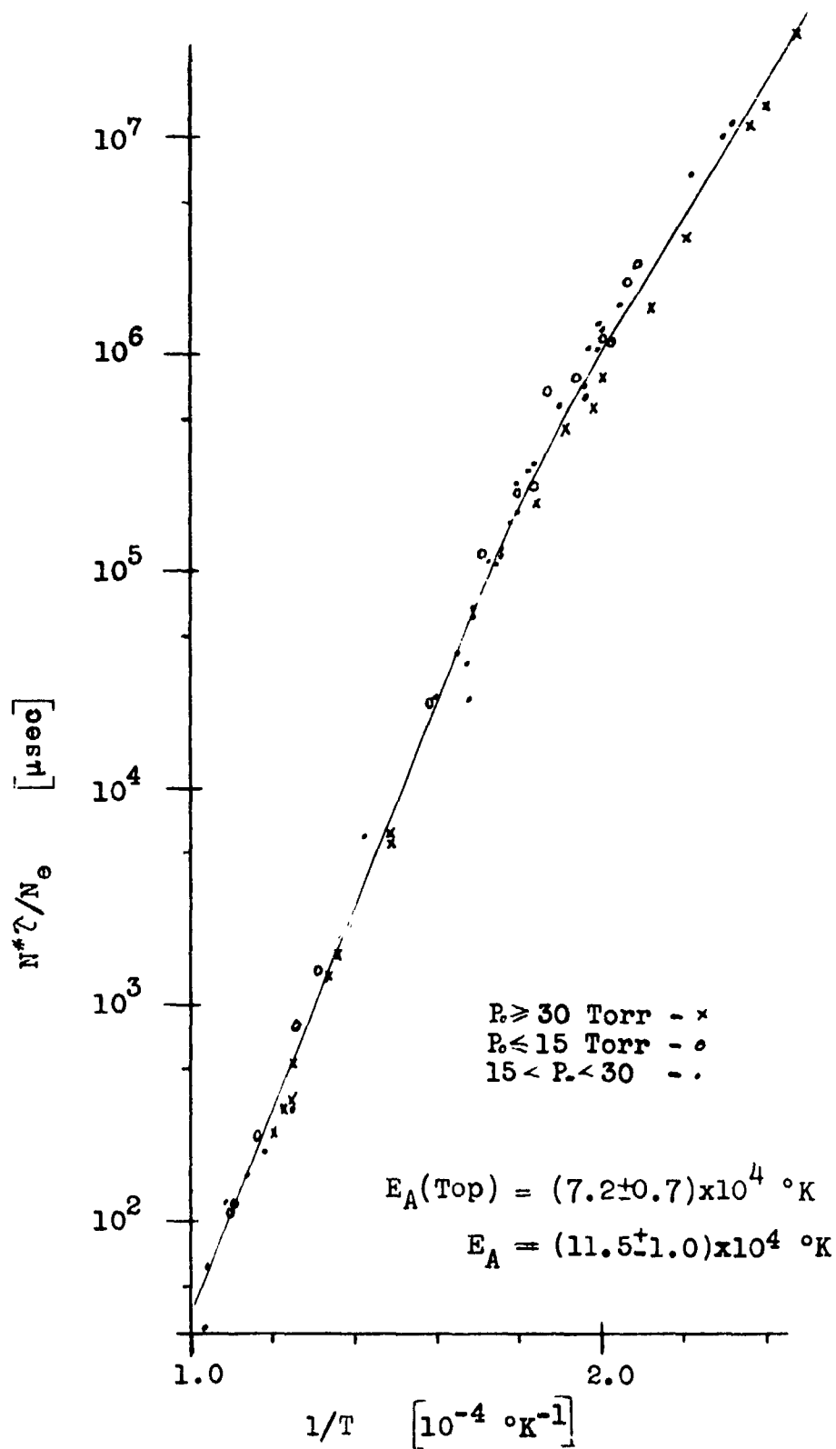
Figure 16. Plot of \log(N^*\lambda/N_e) against 1/T for Mercury.
