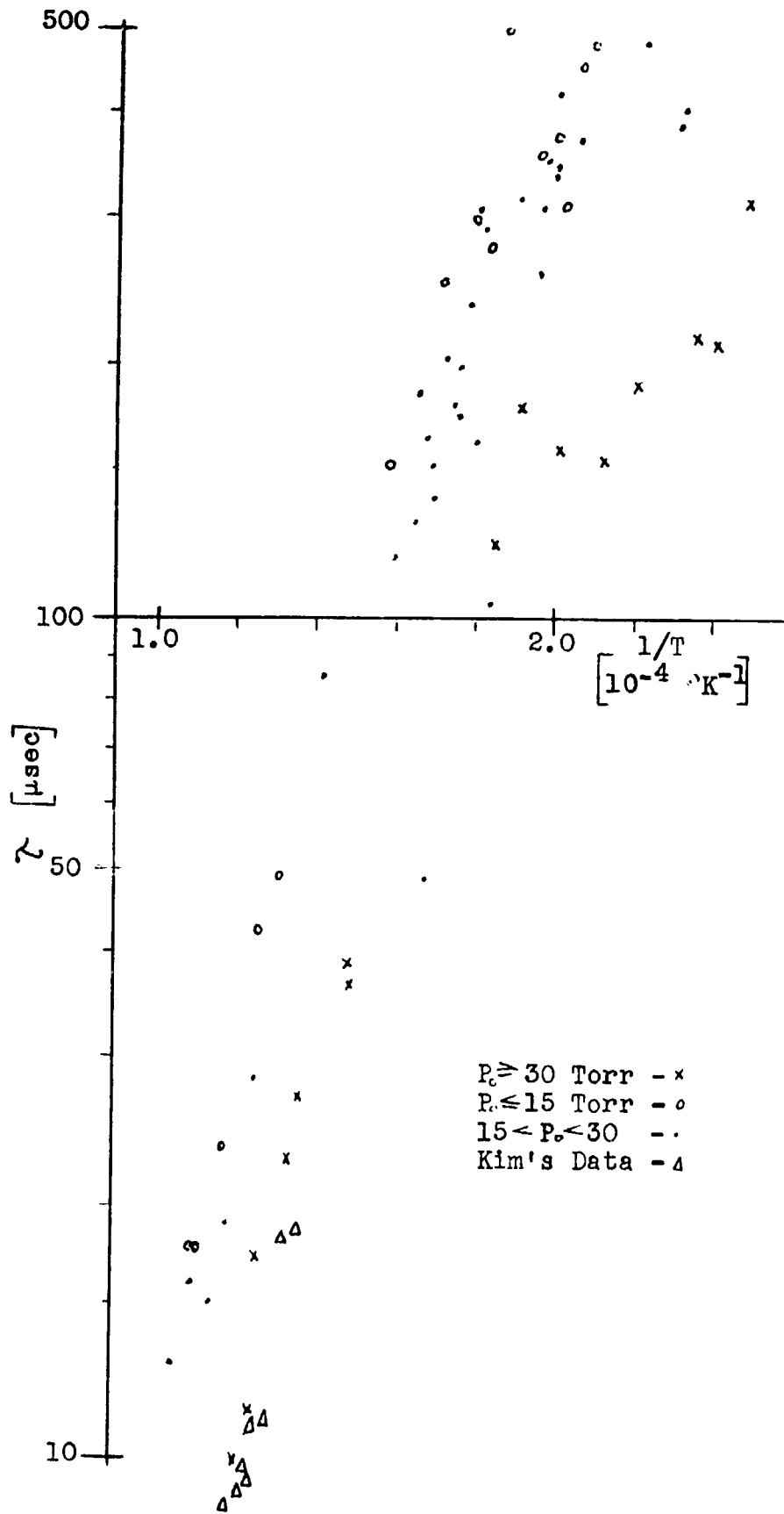
Figure 12. Plot of \log \tau against 1/T for Mercury.
