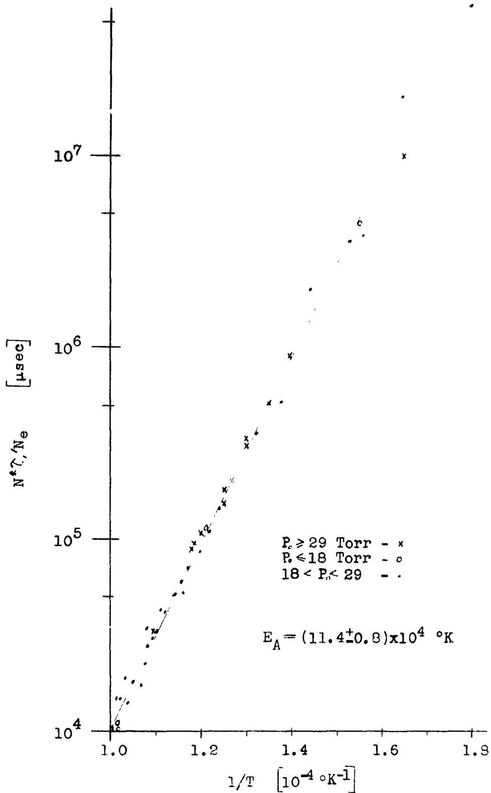
Figure 19. Plot of \log(N^* \tau / N_e) against 1/T for Argon.
