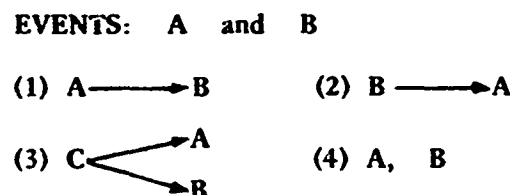
Fig. 1. NATURE OF ASSOCIATION with respect to causation. (1) A caused B, (2) B caused A, (3) C caused both A and B, or (4) A and B occurred, totally unrelated with respect to causation (i.e. "coincidentally").
