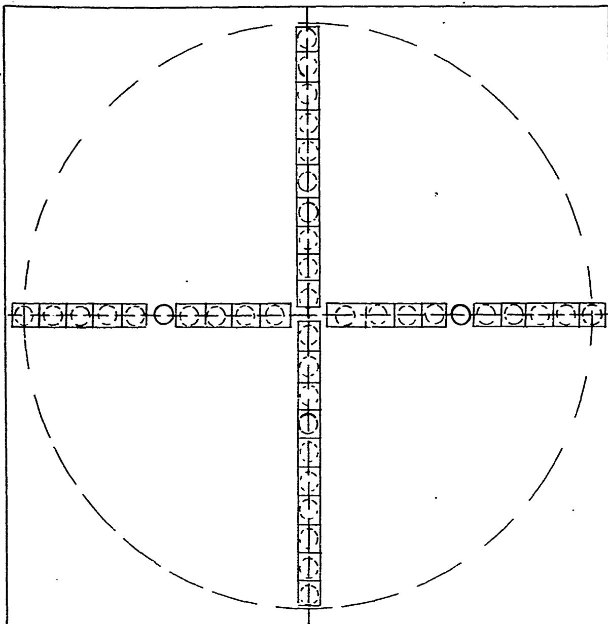
Diaphragm for Zonal Testing of 31" diameter Obsidian Mirror
