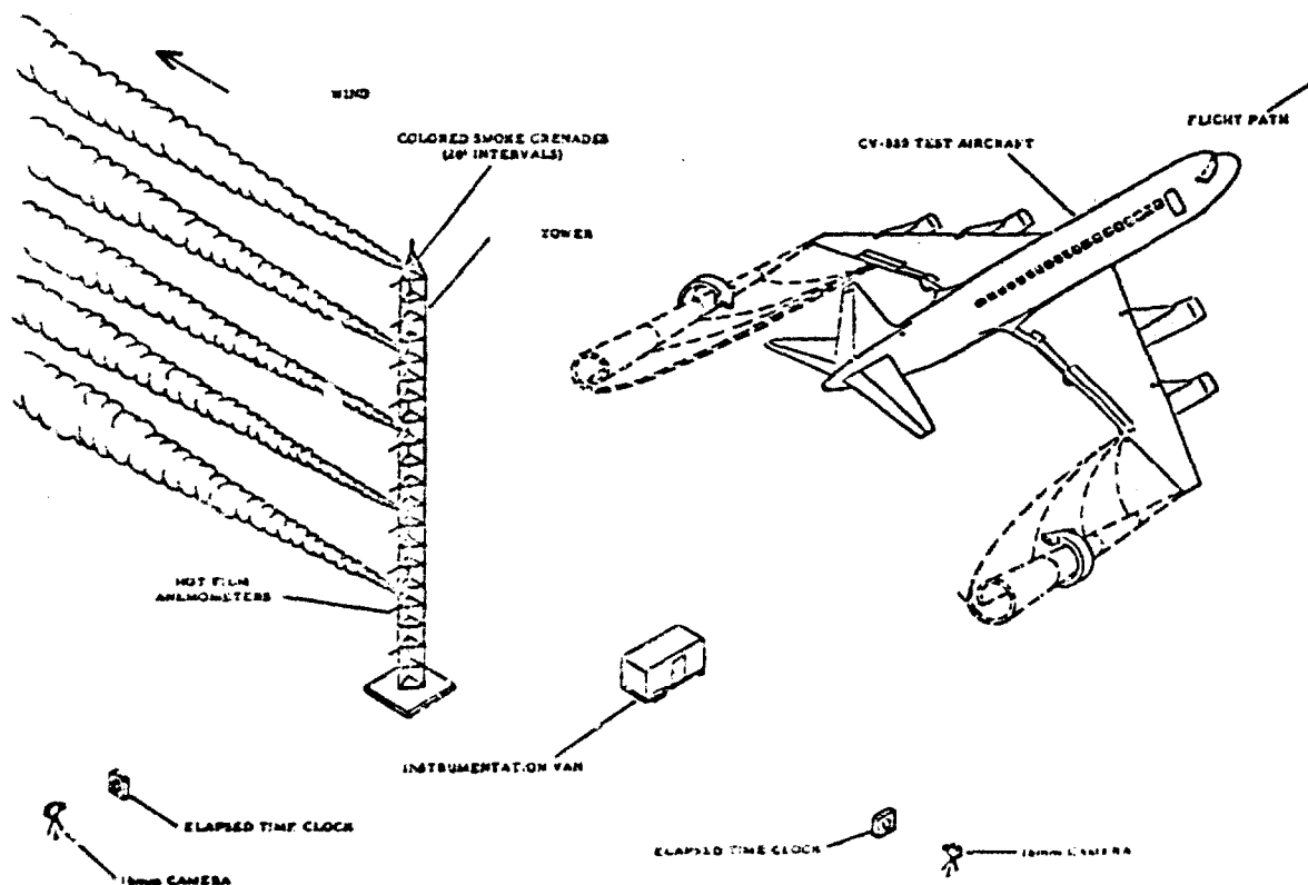
Figure 76. Tower Fly-By Schematic.
