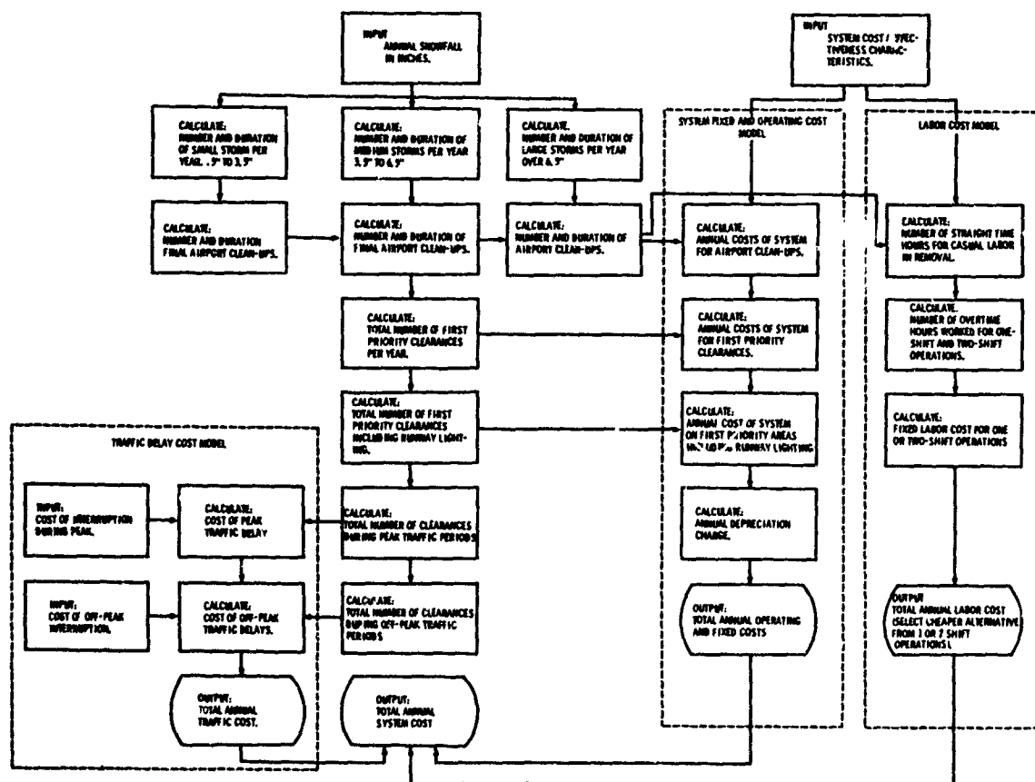
Figure 24. Planning Process Airport Snow Removal and Ice Control.
