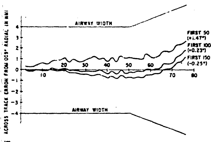
Figure 72. Effect of Sample Size on Track Data.
