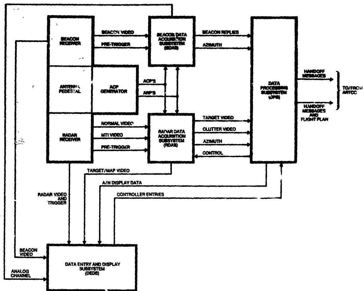
Figure 47. Radar/Beacon Tracking Level (Level B).
