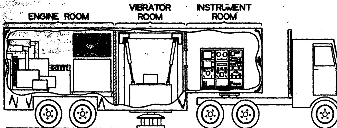
Figure 25. Nondestructive Pavement Testing System.
