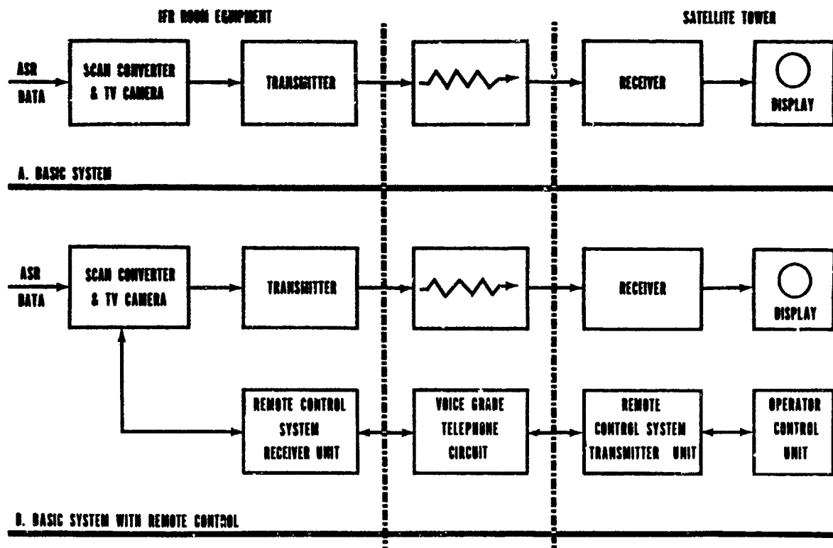
Figure 12. Remoting System Block Diagram.
