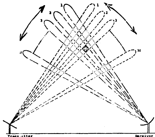
Figure 75. Acoustic Swept-Beam Configuration.
