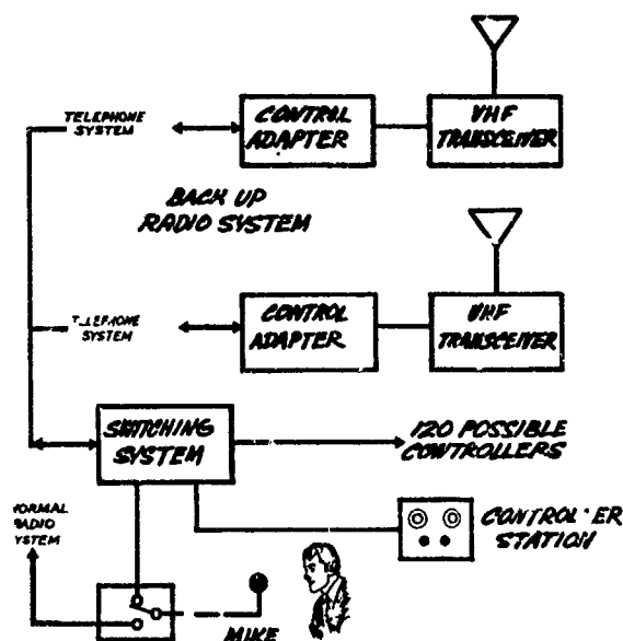
Figure 8. Backup Emergency Communications System.
