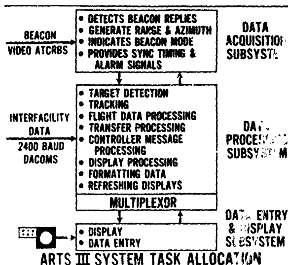
Figure 43. Functional Activities of each Subsystem.
