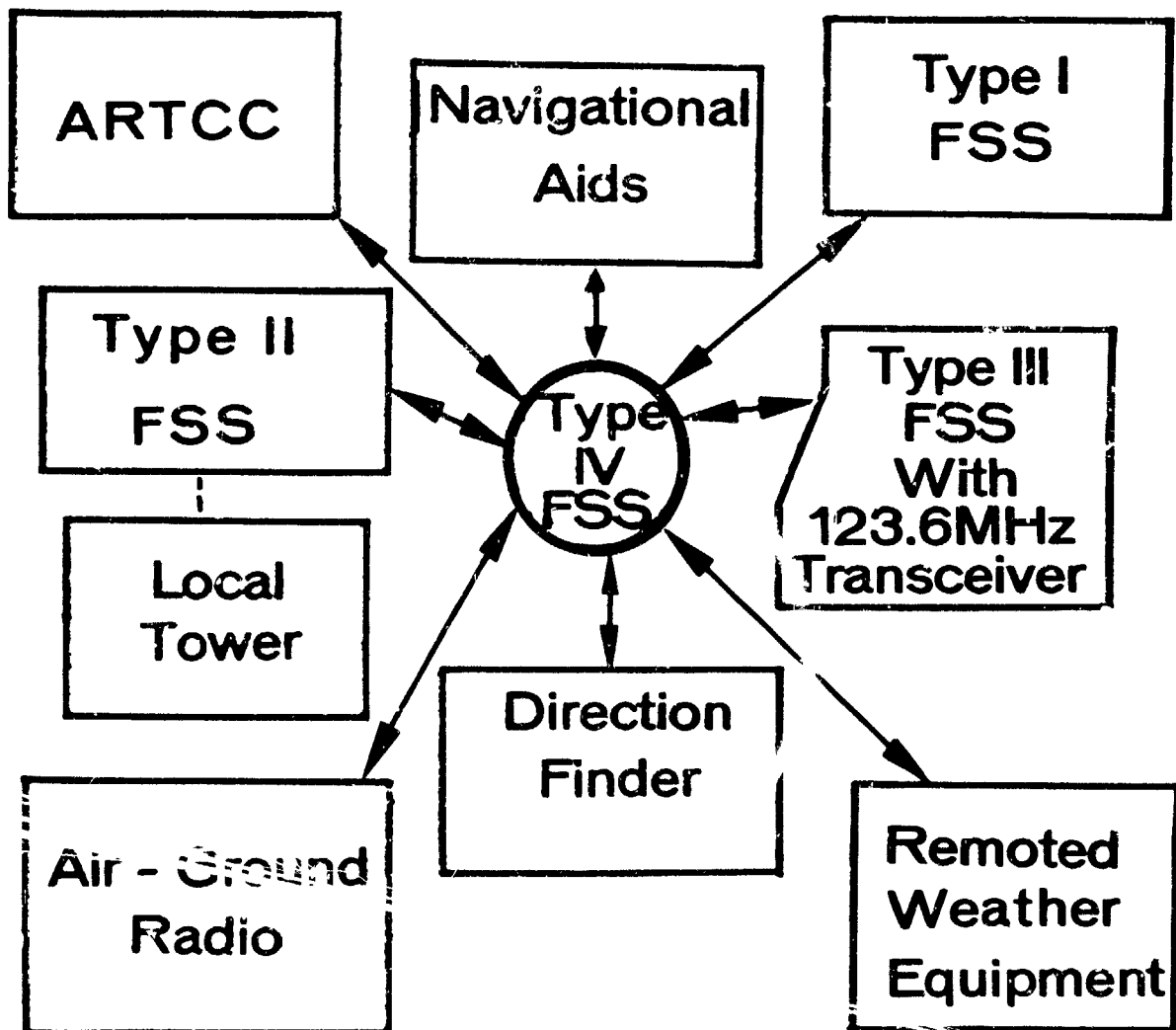
Figure 38. Reconfigured FSS Communications.
