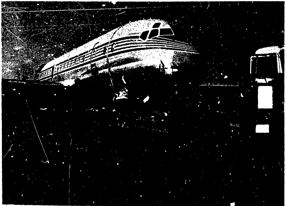
Figure 27. Disabled Aircraft Recovery Using Conventional Methods.
