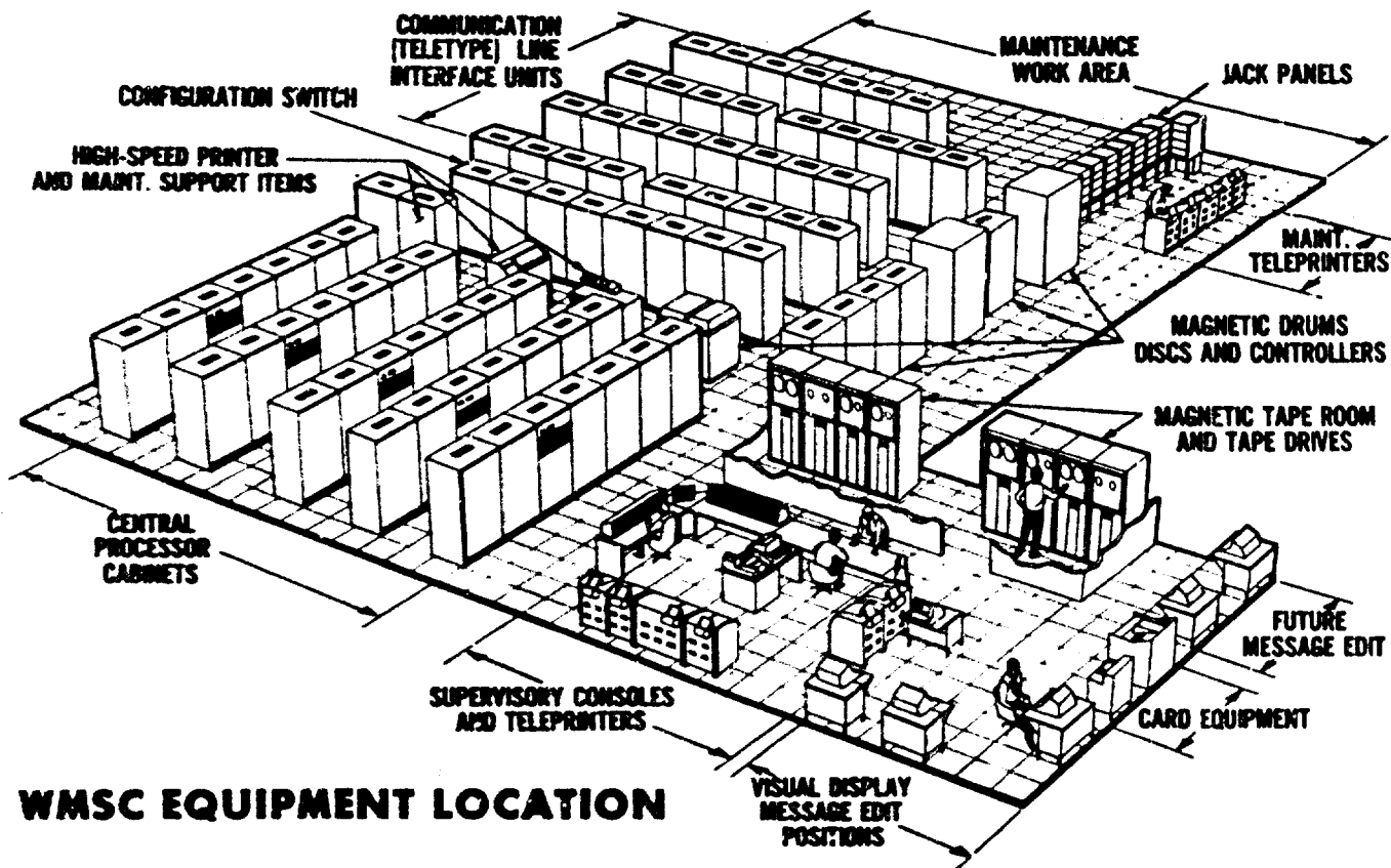
Figure 10. Equipment Layout.
