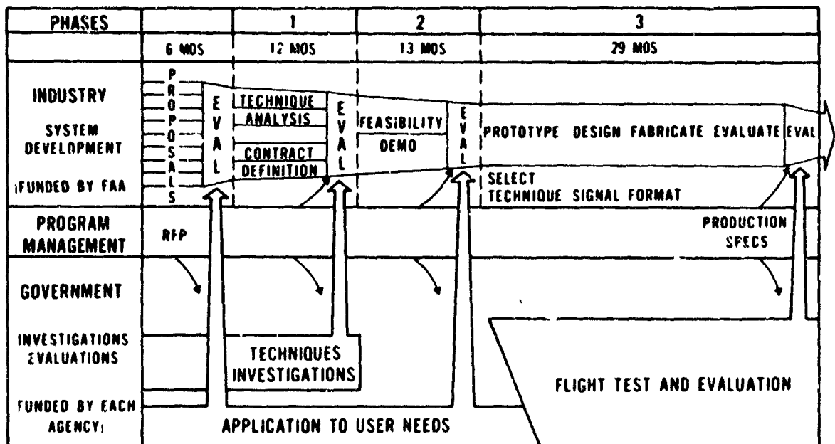
Figure 21. MLS Development Plan.
