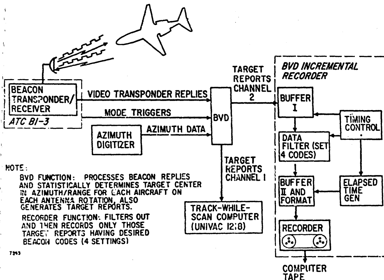
Figure 71. Typical BVD Recording Installation.
