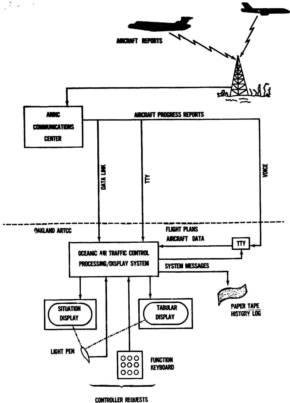
Figure 32. Schematic of System Terminals.
