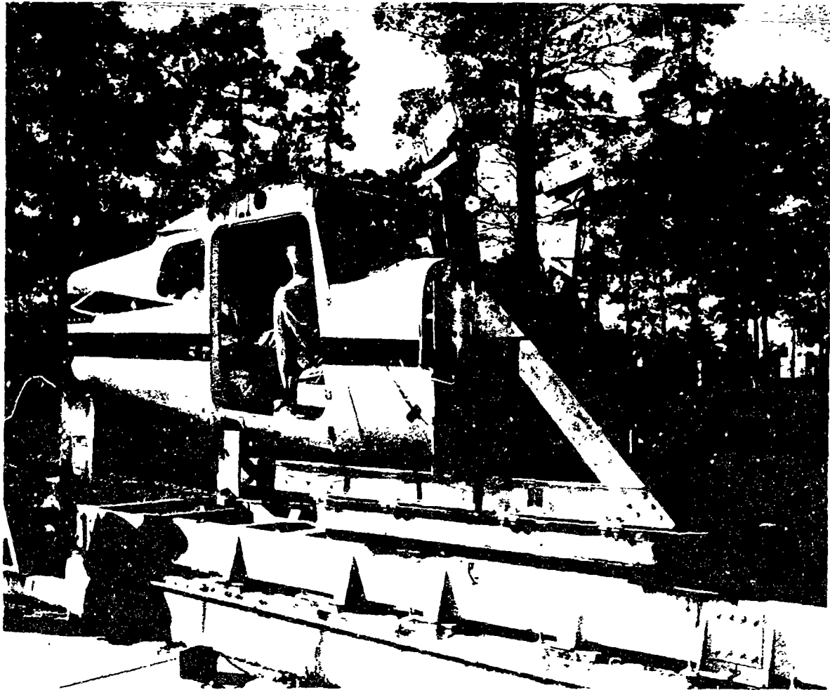
Figure 64. Shoulder Harness and Lap Belt Catapult Test Vehicle.
