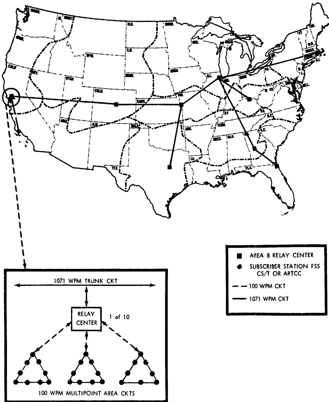
Figure 11. Area B System Circuit Network.
