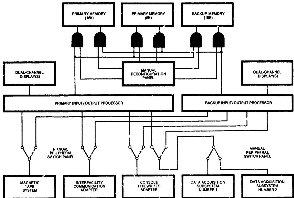
Figure 46. Redundant Basic Arts III System (Level A).
