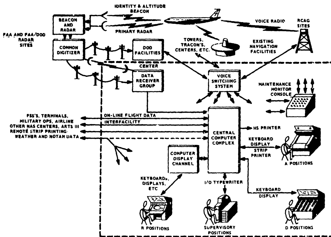
Figure 34. Enroute Stage a System Pictorial Diagram.
