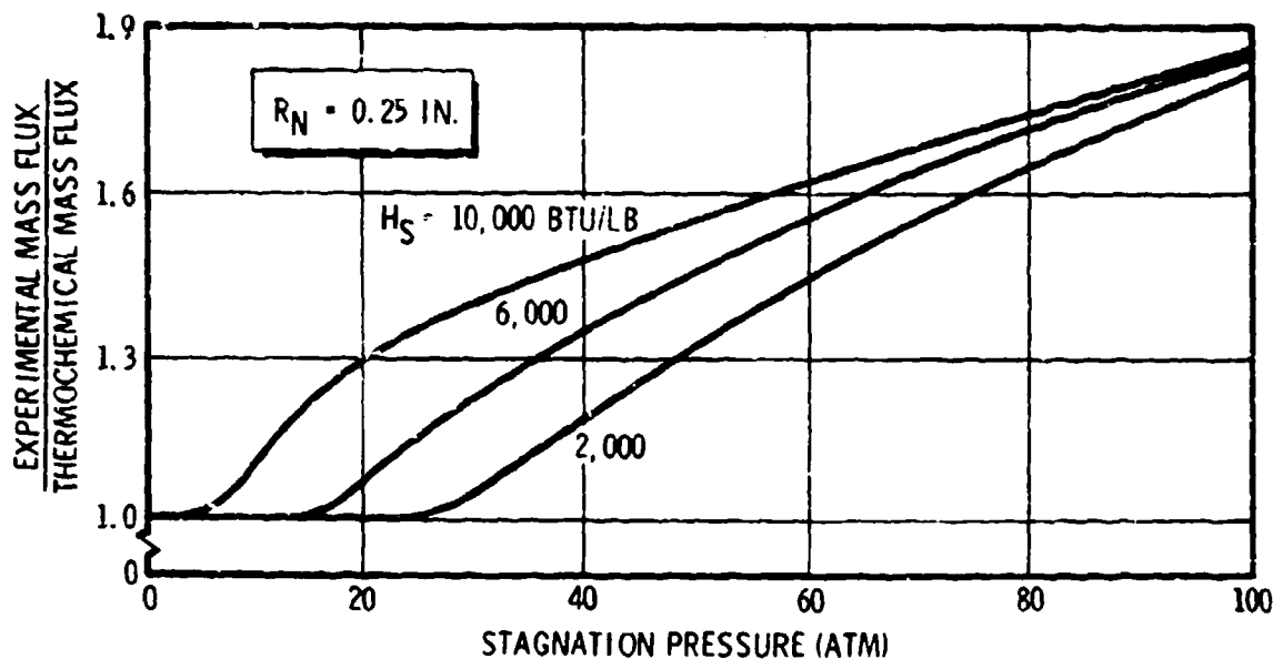
Figure 6. Ratio of Experimental and Thermochemical Mass Fluxes
