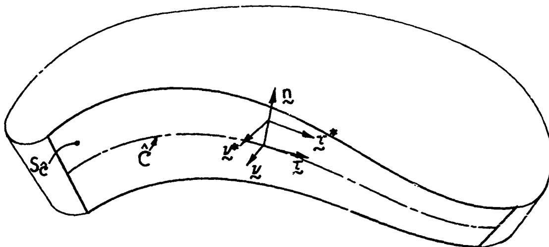
Figure 4.2 The surface S_C^{\wedge} generated by varying z between the limits \pm \frac{h}{2} over the arc \hat{C} . \tau is the unit tangent to \hat{C} and \tilde{\nu} the exterior unit normal to \hat{C} tangent to the middle surface. \tilde{\nu}^* is normal to S_C^{\wedge} and \tau^* is tangent to S_C^{\wedge} and the middle surface, but \tilde{\nu}^* and \tau^* need not be unit vectors.
