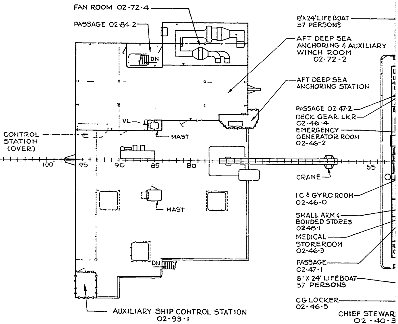
Fig. 3j — Plan view, 02 level
