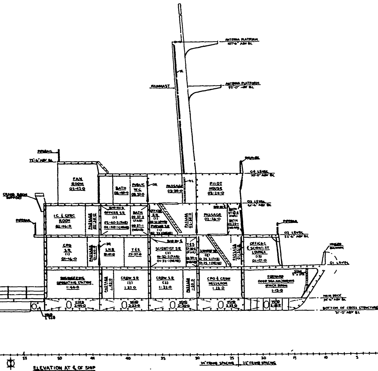
3b - Elevation, inboard
