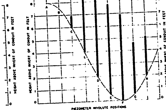
DISCHARGE - 1740 CFS
