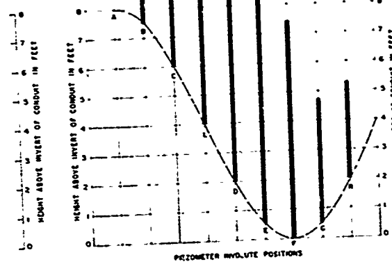
PRESSURE GRAPH
