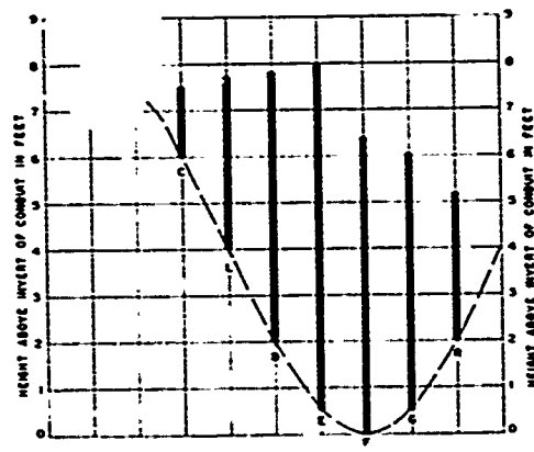
PRESSURE GRAPH
