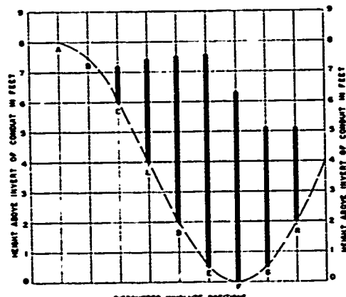
DISCHARGE - 1900 CFS
