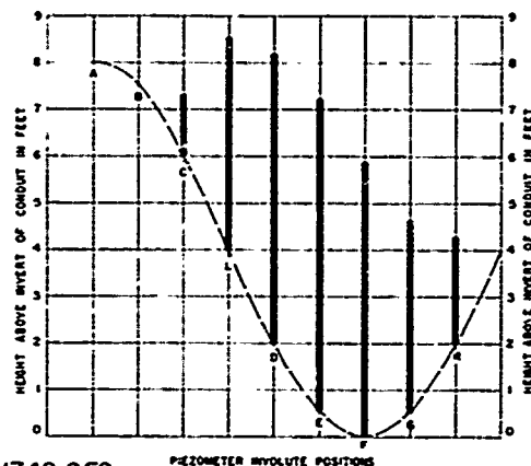
DISCHARGE-1740 CFS
