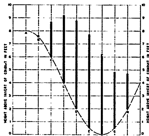
PIEZOMETER INVOLUTE POSITIONS
