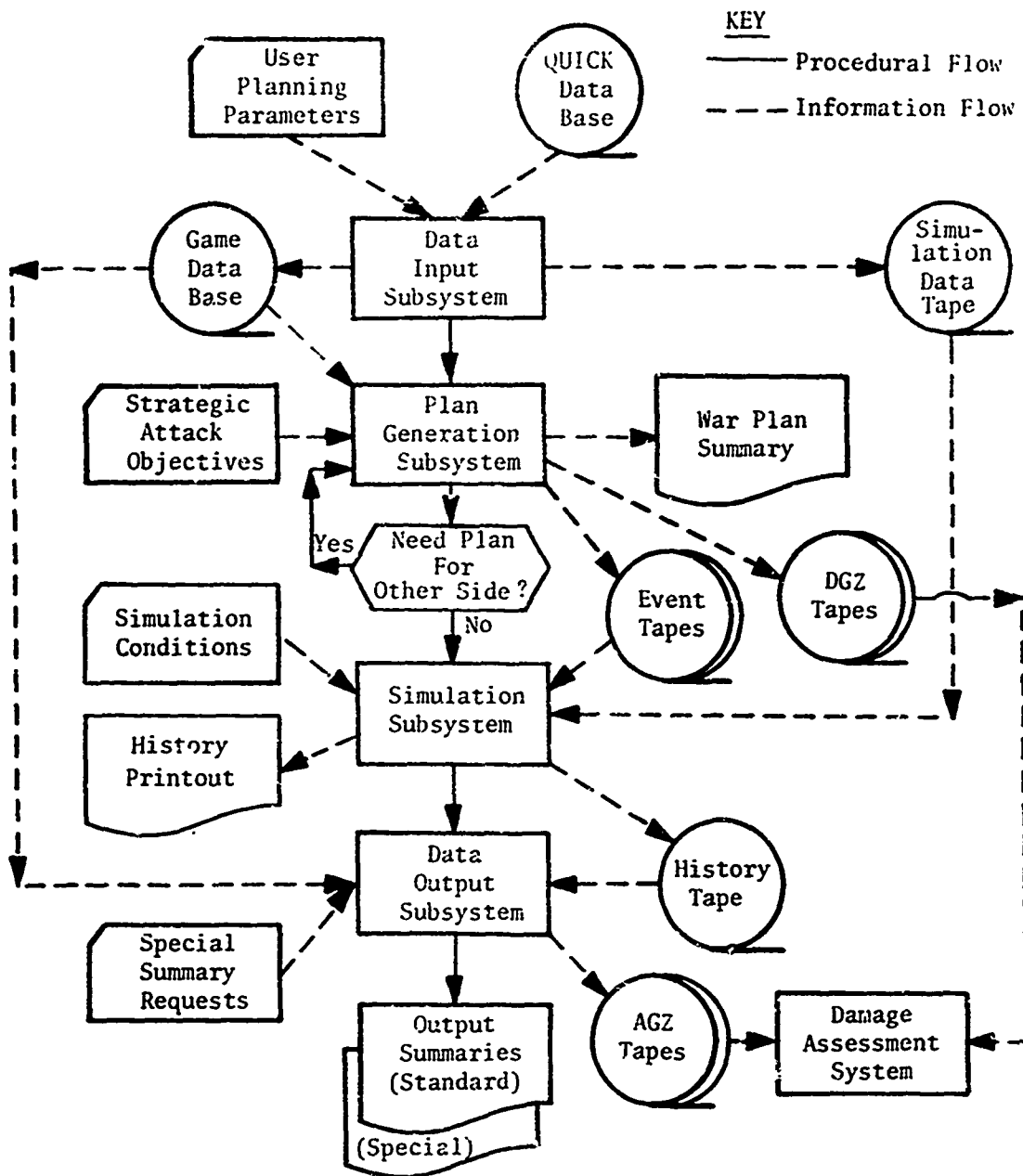
Fig. 1. Procedure and Information Flow in QUICK
