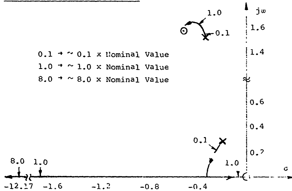
Figure 39. 60 Knots Lateral N_r and L_o Root Loci.
