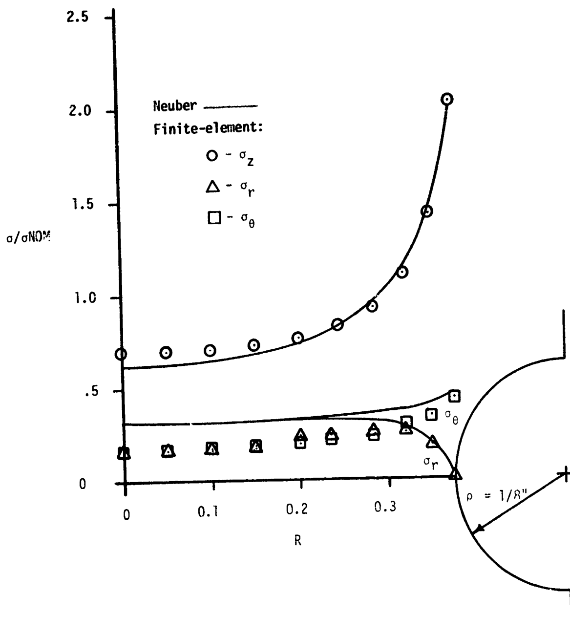
Figure 27. Comparison of Finite-element Results with Neuber Solution in Vicinity of 1/8 in. Radius Notch
