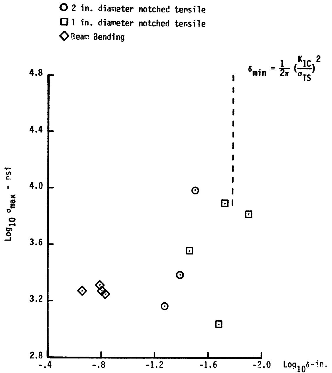
Figure 38. Critically stressed distance for non-uniform stresses in Nugget sandstone.
