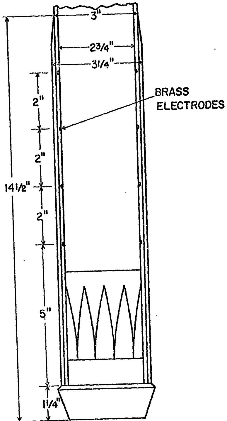
Figure B-4 Inner Corer Ring Electrode Array.
