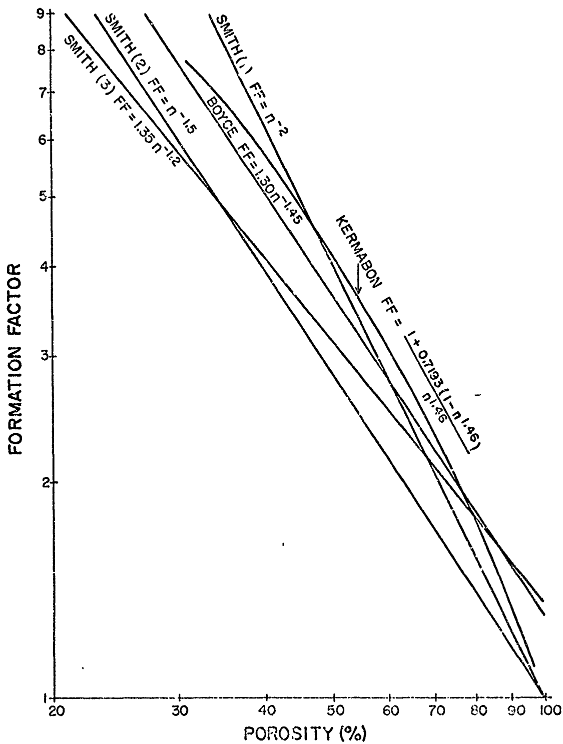
Figure 5. Formation Factor-Porosity Relationships Proposed by Boyce, Kermabon, et. al., and Smith.
