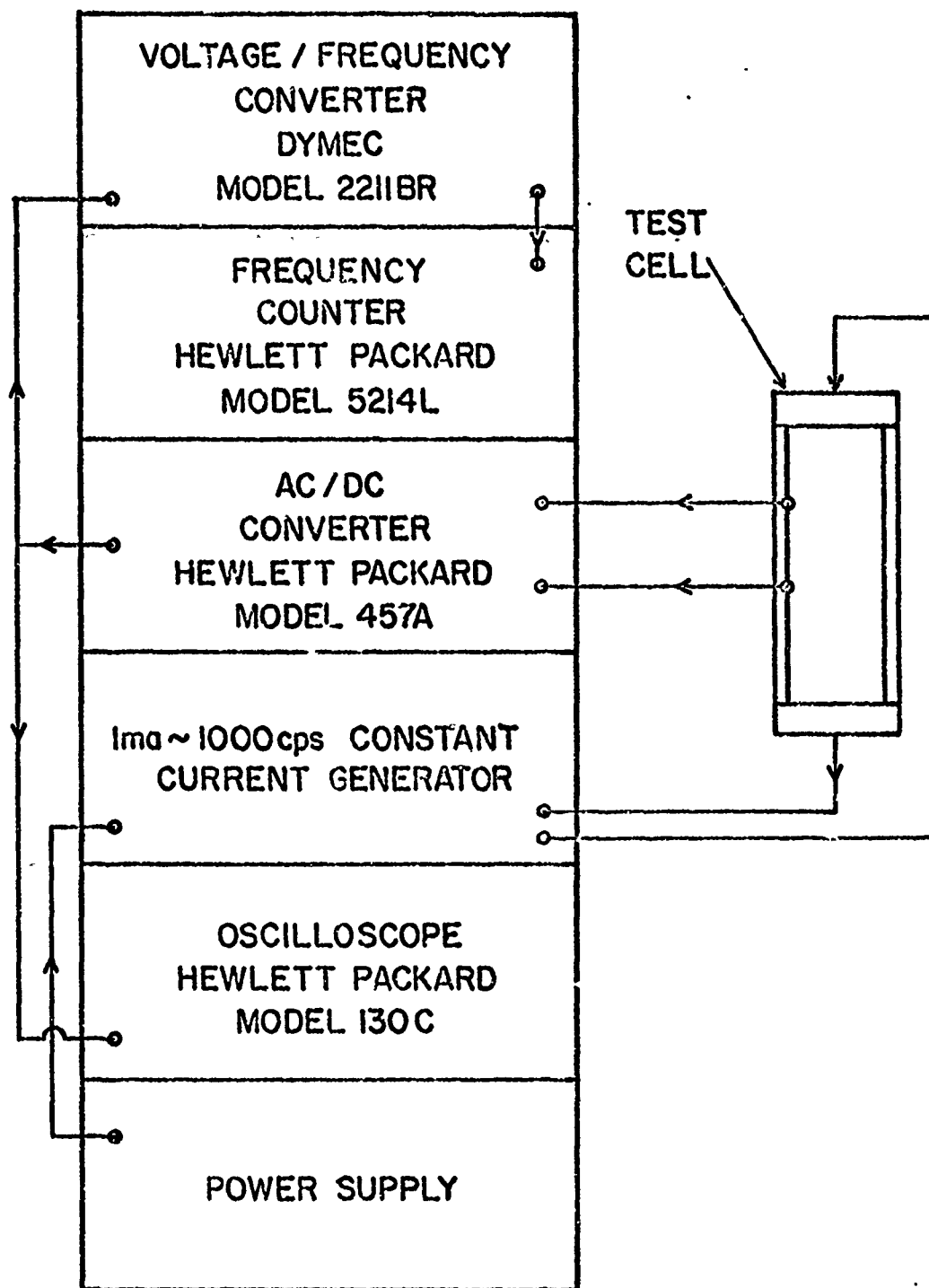
Figure B-5 Electronic Block Diagram of the Simple and Modified Apparatus.
