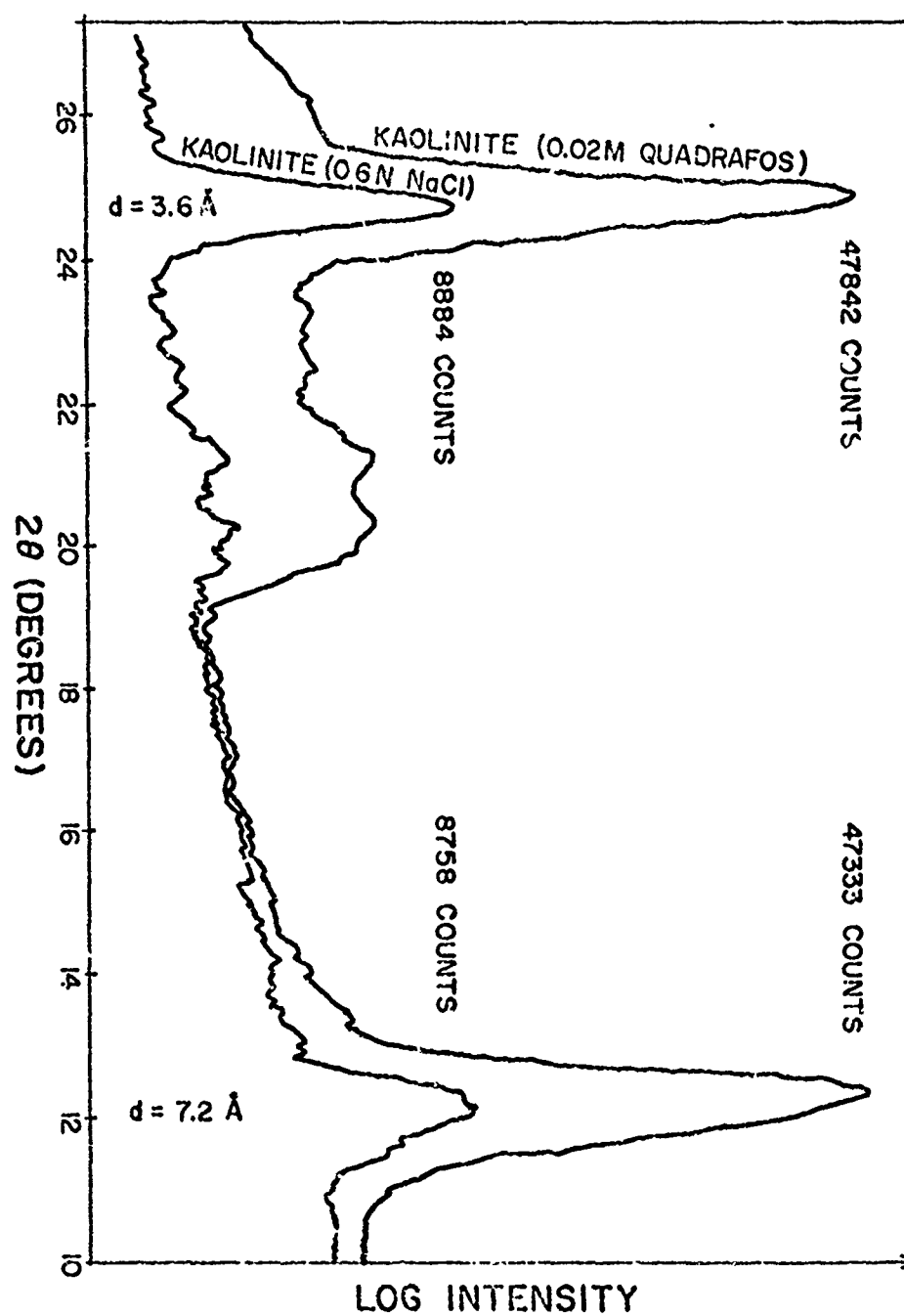
Figure 27. X-Ray Diffractograms of Two Structures of Kaolinite Clay.
