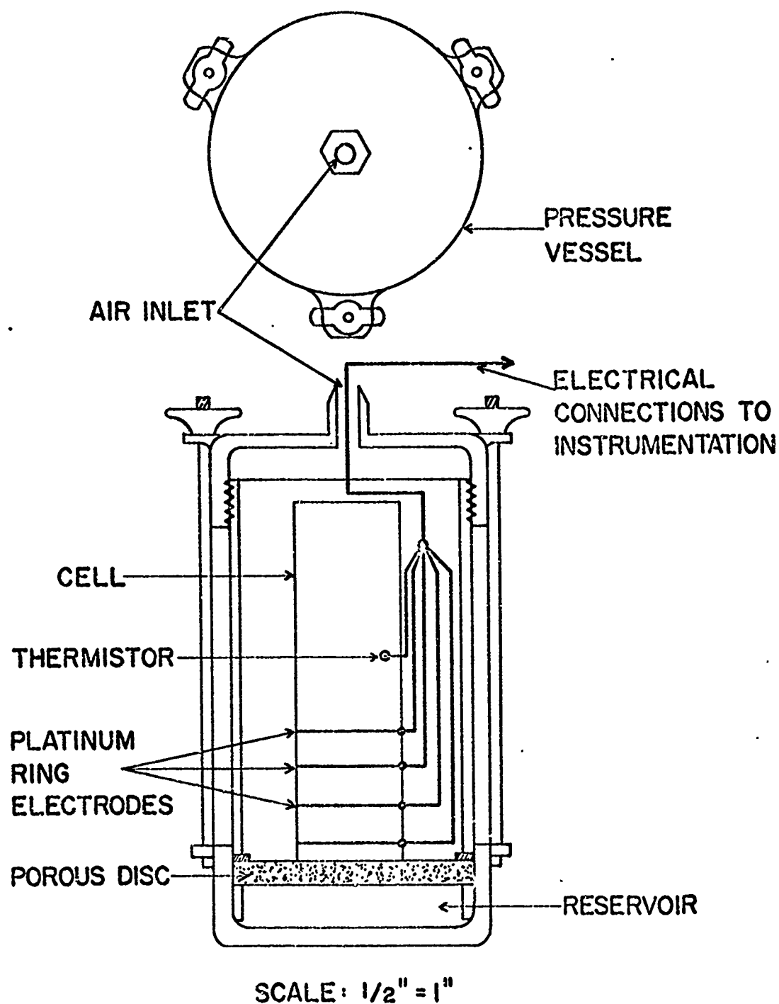
Figure B-3 Redesigned Apparatus Pressure Vessel and Test Cell.
