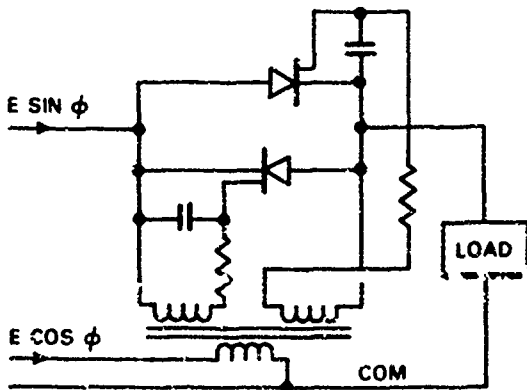
Fig. 11. Basic SCR power switch circuit.
