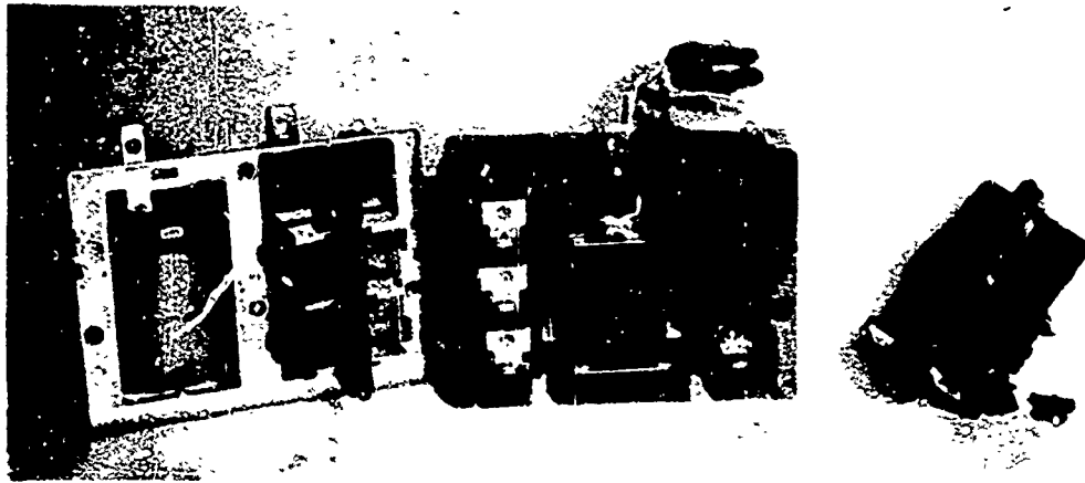
Fig. 7. Extensive carbon formation and severely burned contacts inside contactor.
