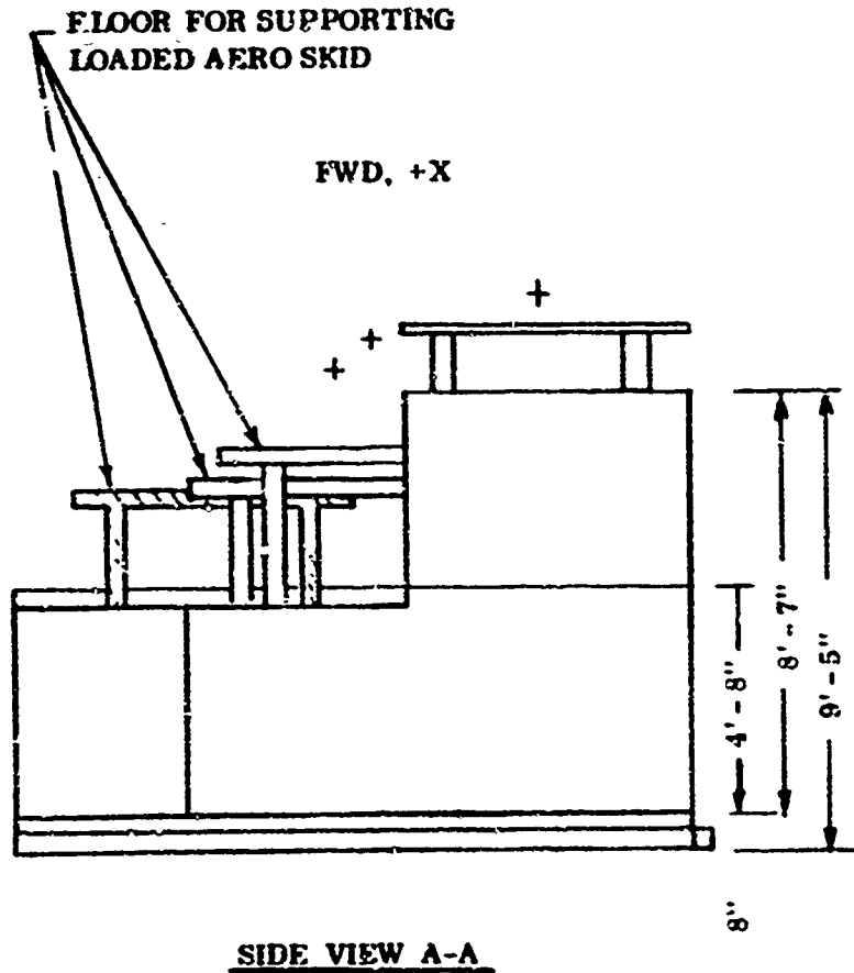
FIGURE 11. ORDNANCE PALLET FOR A-7 A/C ONLY
