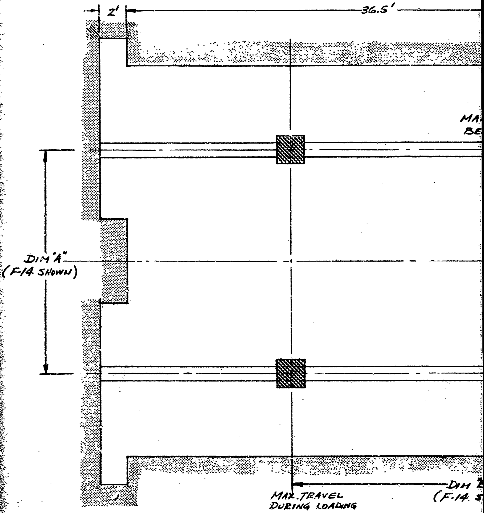
FIGURE A-3, CONCEPT 'B'. LAY SUPPORT POI
