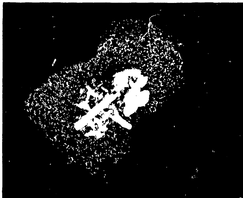
Figure 7. Exaggerated Grain Growth of \alpha -Al 2 O 3 in Billet Fabricated from Vendor I Lot 120 Powder.
