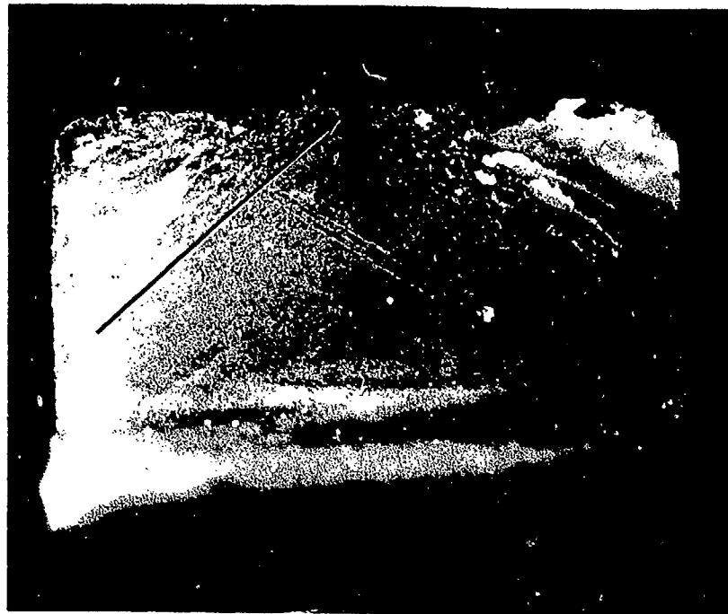
Figure 12. Flaw Origin Occurring at a Dark Inclusion in FLU 2-1a.
