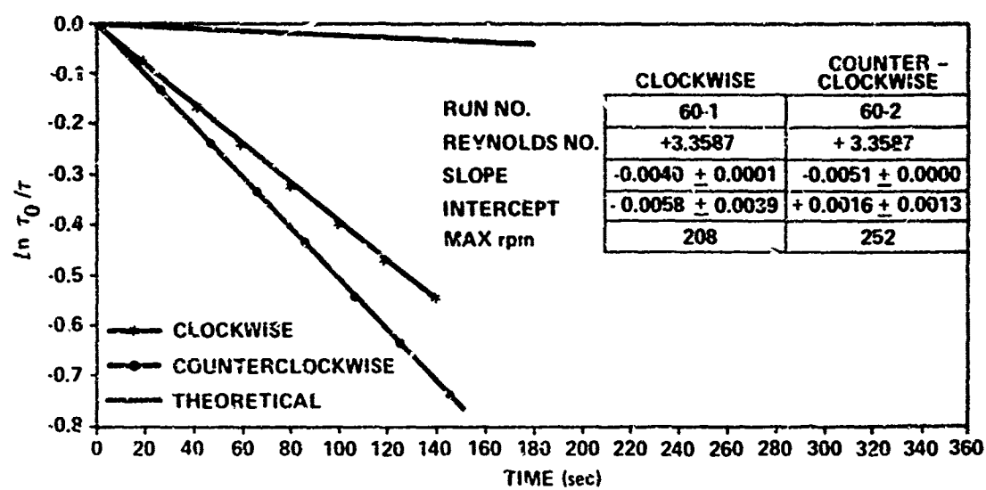
Figure 12. Shaft speed decay, R = +3.3587 .
