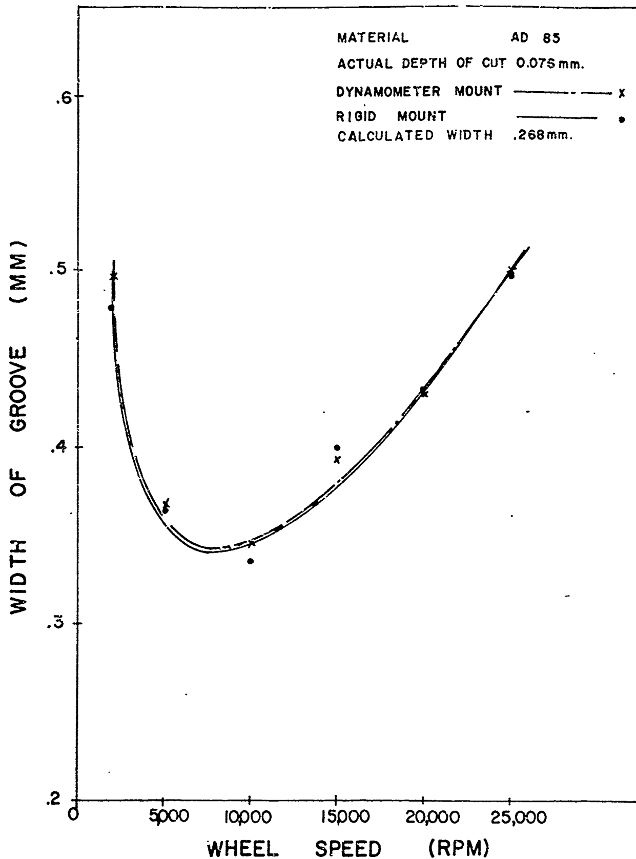
FIGURE 3, Measured Width-of Groove Versus Wheelspeed. AD 85, .003" Depth of Cut, 120° Diamond Cone.
