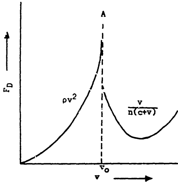
FIGURE 37. General Features of \bar{F}_D in a Brittle Material.
