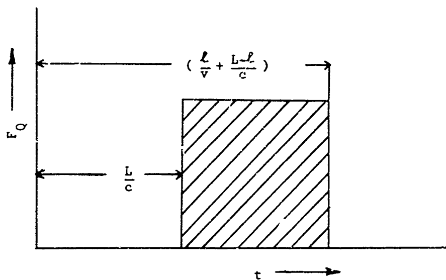
FIGURE 34. Force Measured by the Transducer as Modified by a Fracture.
