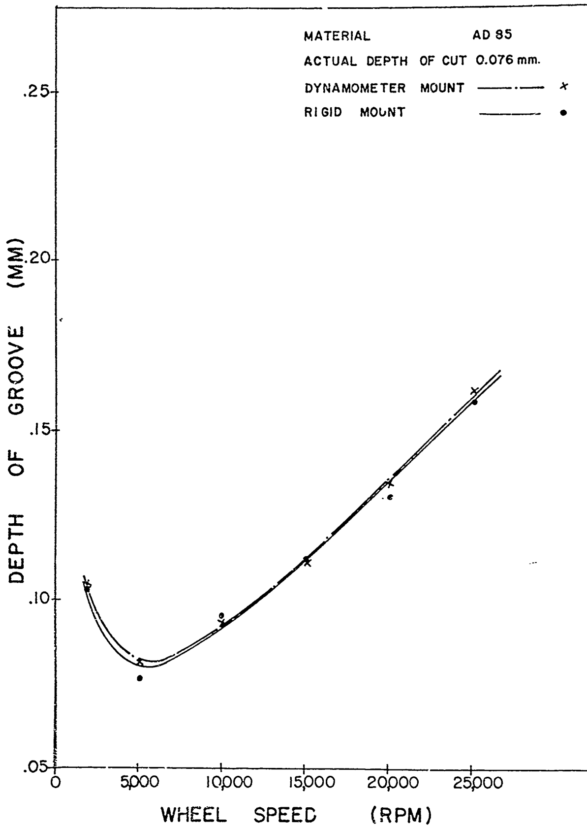
FIGURE 2. Measured Depth of Groove Versus Wheelspeed. AD 85, .003" Depth of Cut, 120° Diamond Cone.
