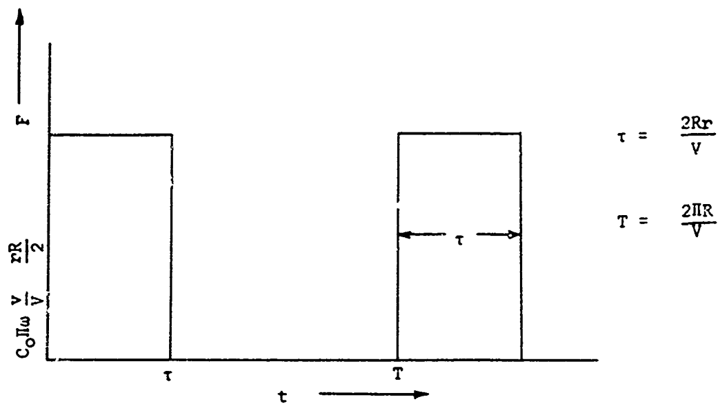
FIGURE 26. Force Experienced by the Cutting Point.
