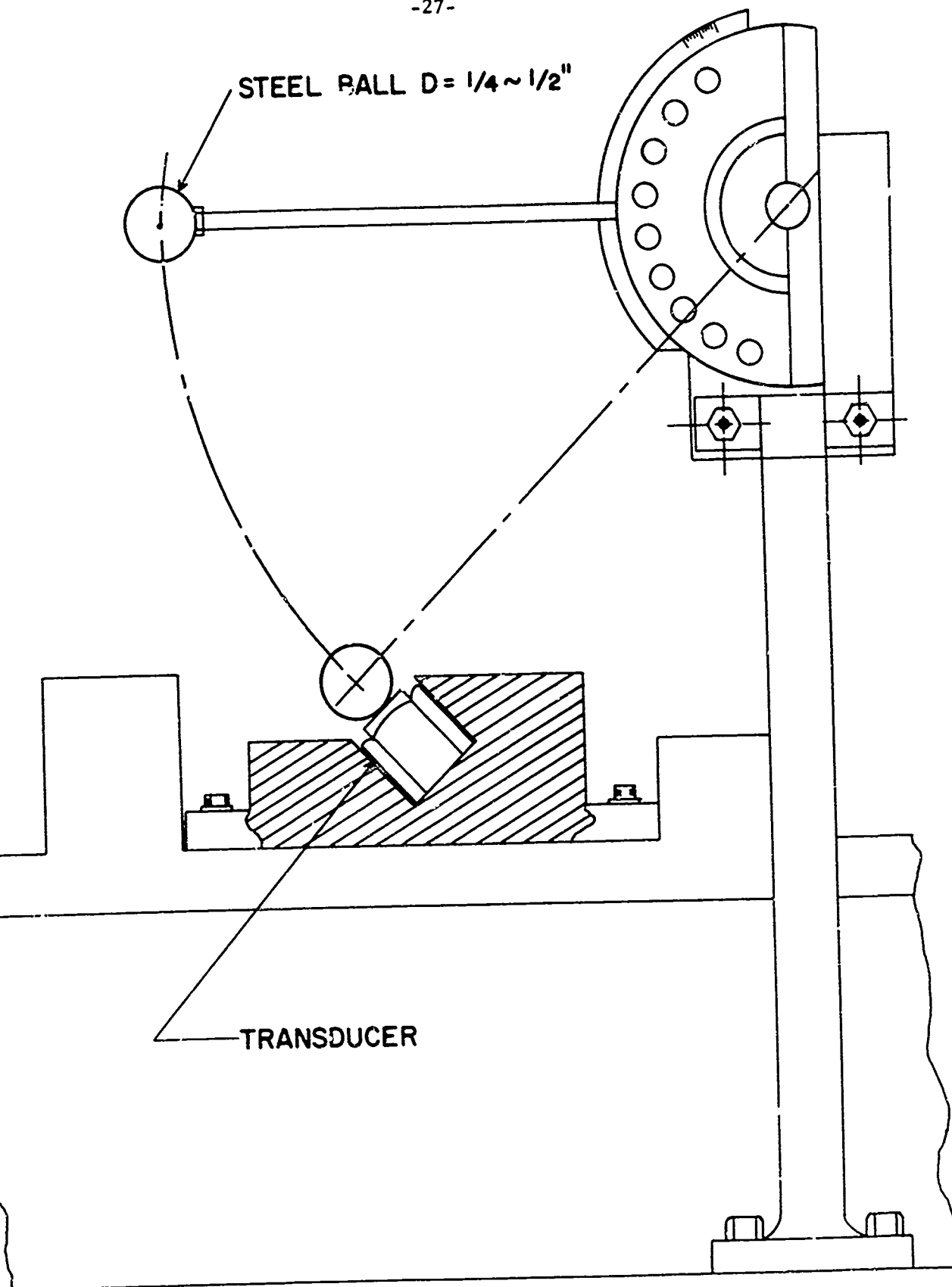
FIGURE 8. Calibration Device for Horizontal and Vertical Forces for Dynamometer of Figure 6.
