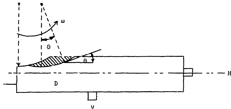
FIGURE 29. Geometrical Configuration of Force Measurement Experiment.
