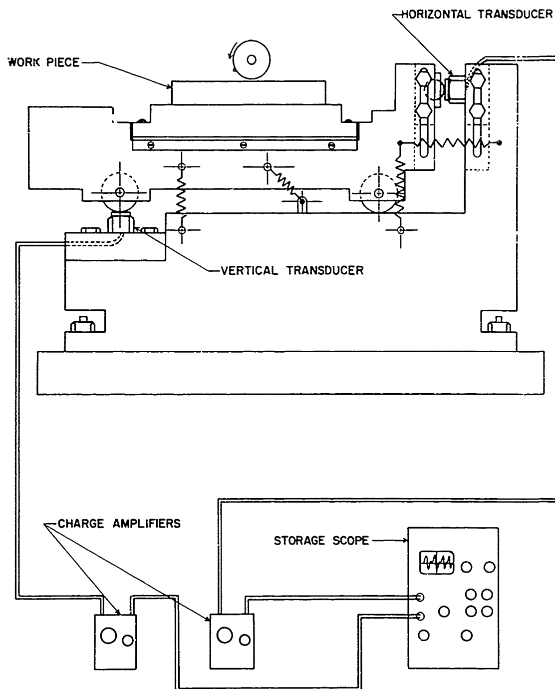
FIGURE 5. Piezoelectric Dynamometer (Schematic) with Readout Equipment.
