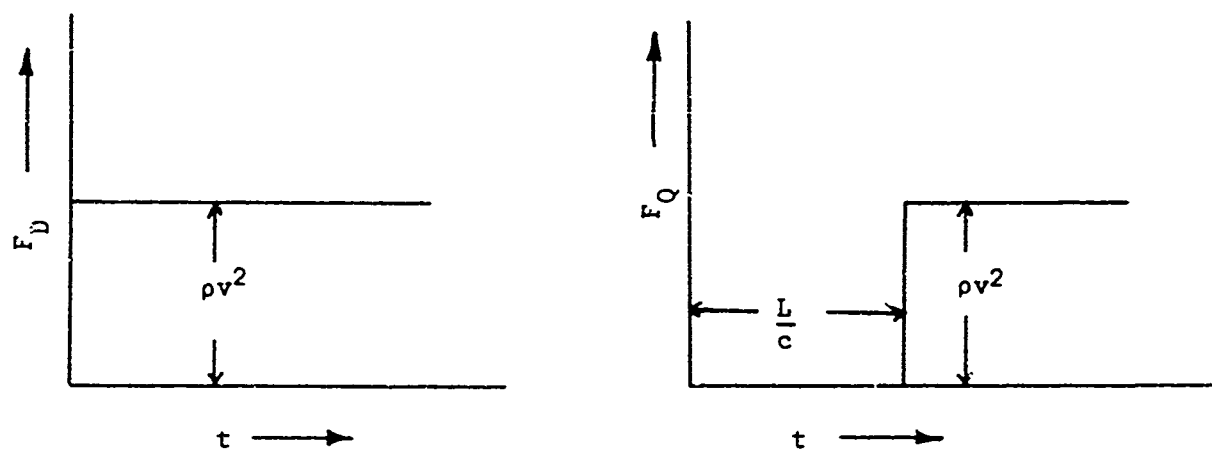
FIGURE 33. (a) Force Experienced by Cutting Point. (b) Force Measured by Transducer.
