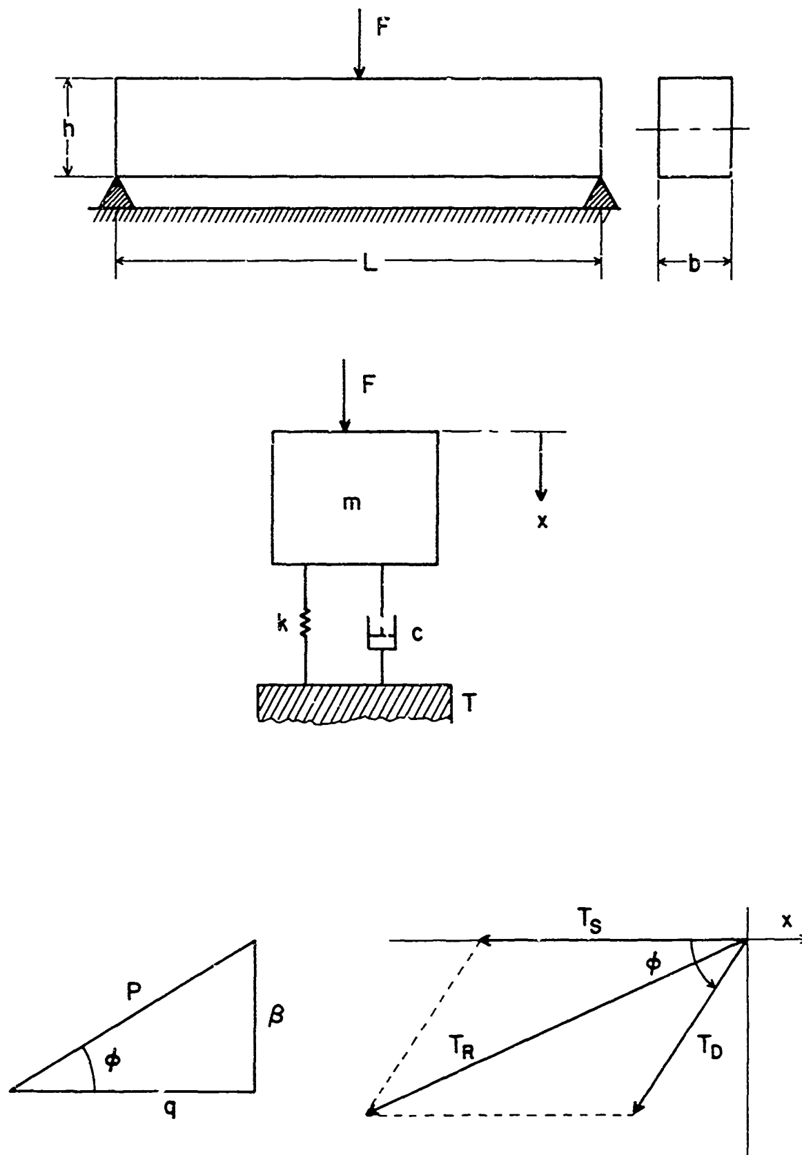
FIGURE 7. Idealized Model of Dynamometer (see text for explanation)
