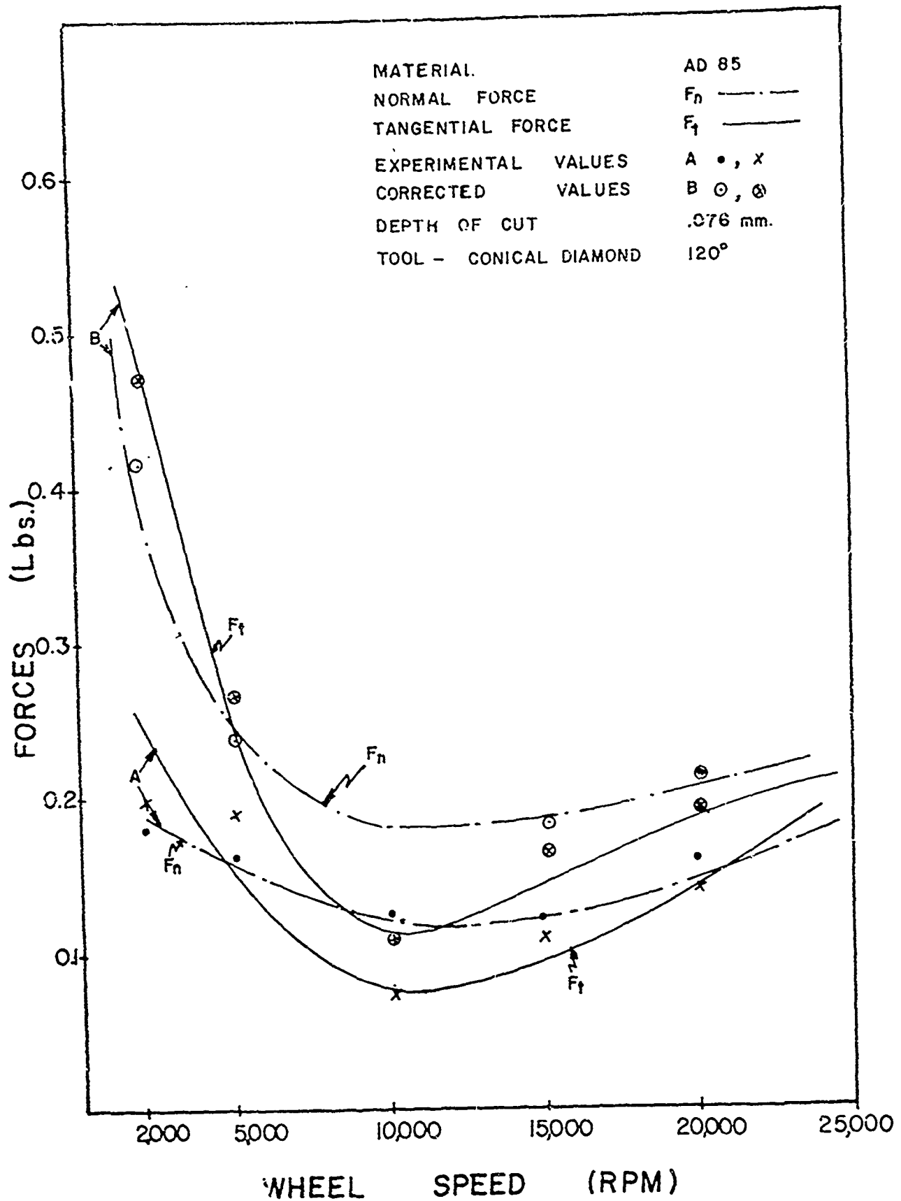
FIGURE 1. Peak Grinding Forces as a Function of Wheelspeed Before and After Adjustments for Dynamometer and Electronic Response. AD 85, .003" Depth of Cut, 120° Diamond Cone.
