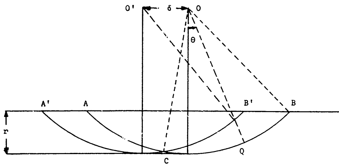
FIGURE 27. Trajectory of Cutting Point in Two Successive Cuts.
