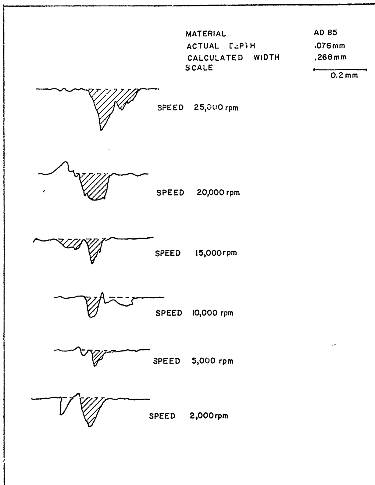
FIGURE 4. Profilometer Traces Recorded at One Point Across a Series of Grooves Cut at Various Wheelspeeds. AD 85, .003" Depth of Cut, 120° Diamond Cone.
