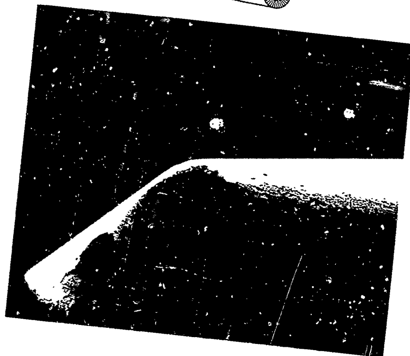
FIGURE 1A. Scanning Electron Micrograph of New Diamond Point. Top 200X, Bottom 500X.
