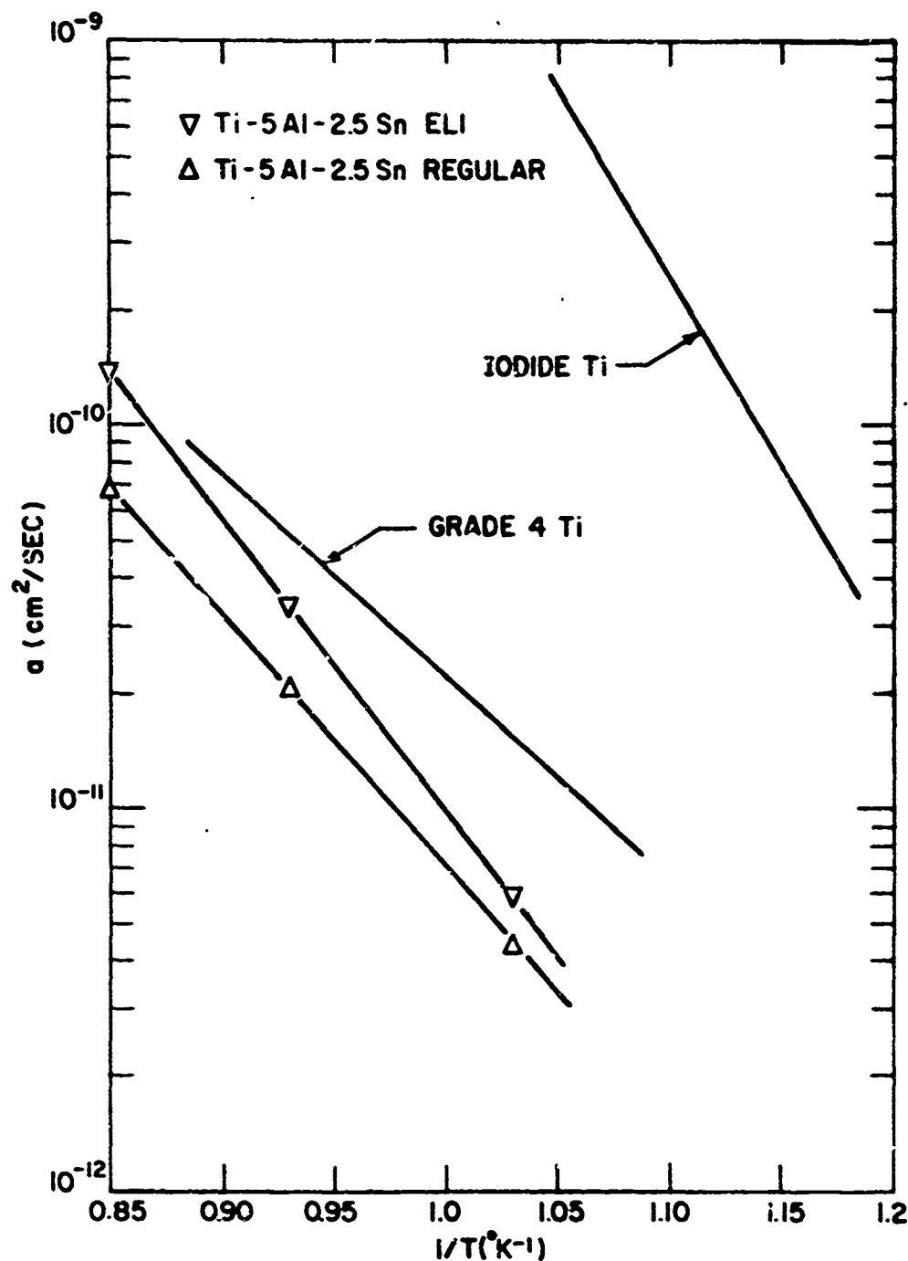
Fig. 4-1. Comparison of the Temperature Dependence of the Grain Growth Rate of Ti-5Al-2.5Sn of Two Purities with the Behavior Observed in Previous Work (4,14) for Unalloyed Titanium.
