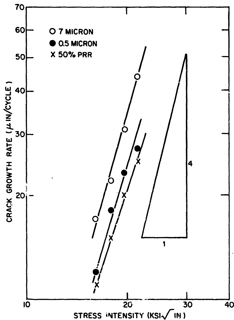
Fig. 5-3. Variation of Fatigue Crack Growth Rate with Stress Intensity Range for Grade 3 Unalloyed Titanium in Three Conditions at Room Temperature.
