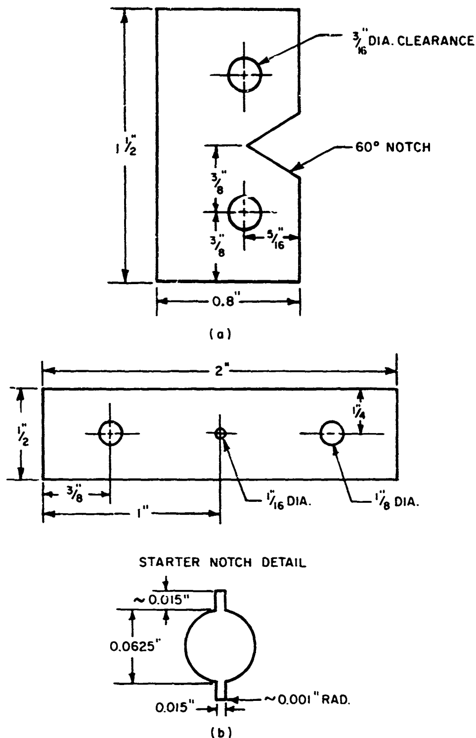
Fig. 3-3. Test Samples Used in Toughness Studies: (a) Tearing Test; (b) Fatigue Crack Propagation Test.
