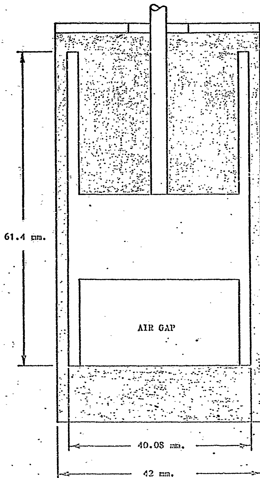
FIGURE 5: DOZ AND CUP ASSEMBLY
