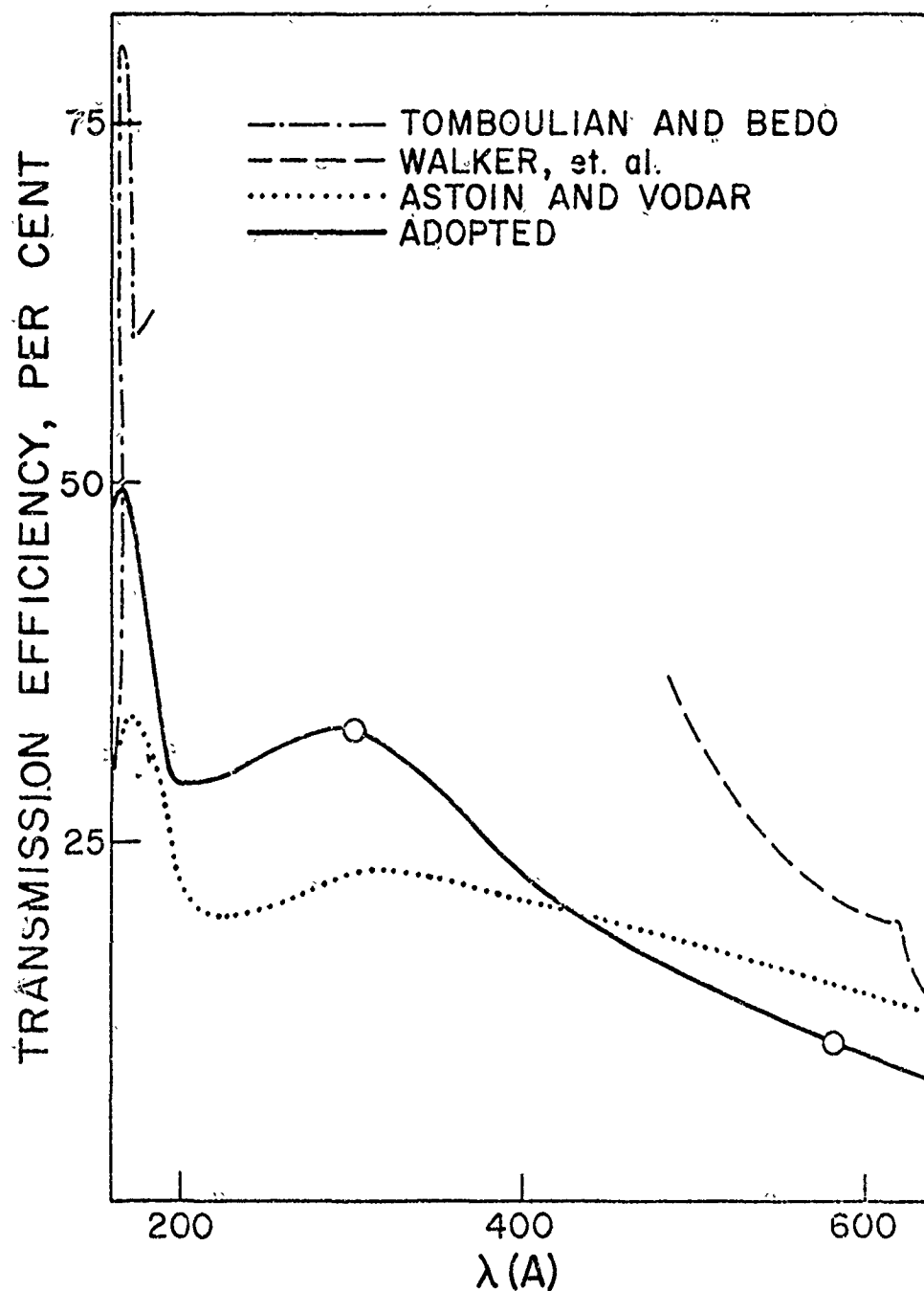
Figure II-2. The percentages of radiation transmitted by aluminum filters of thicknesses 1150Å for the case of Walker, Kustgi, and Weissler; 1000Å for the others. The two points obtained at 304Å and 584Å from laboratory measurements of the filter used in flight are circled. After Tousey (1963), except for the adopted curve.
