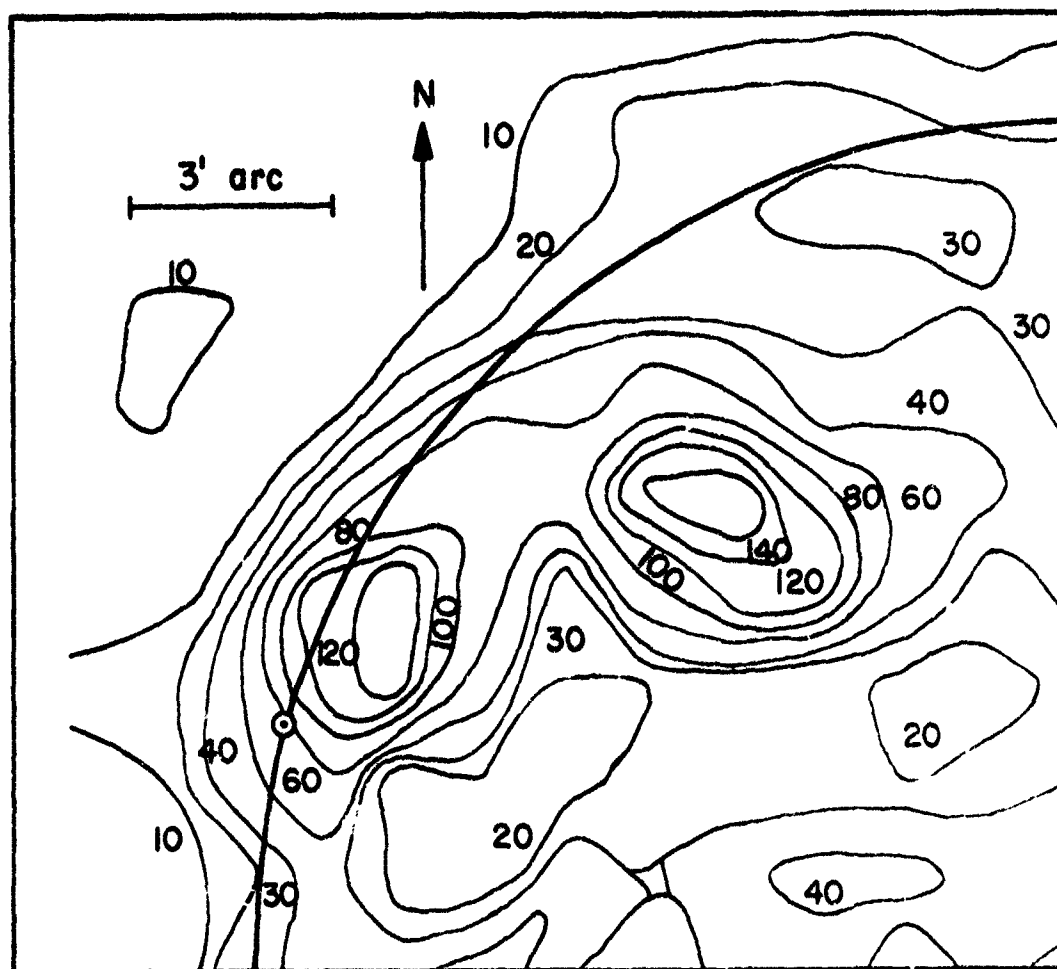
Figure VII-20. A radio brightness temperature map of a portion of the east limb of the sun on April 28, 1966. The map is drawn from Stanior .1 cm data. The position of Feature 4 is marked by a dotted circle.
