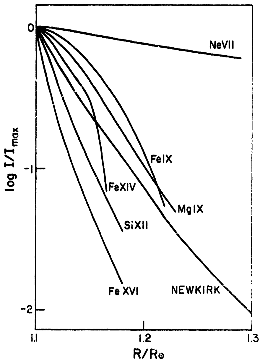
Figure VII-10. Brightness variations of Feature 4 with radial distance from the limb in solar radii. The curve labeled NEWKIRK is Newkirk's (1961) density model is given for comparison. All curves are normalized to equal Newkirk's at the limb.
