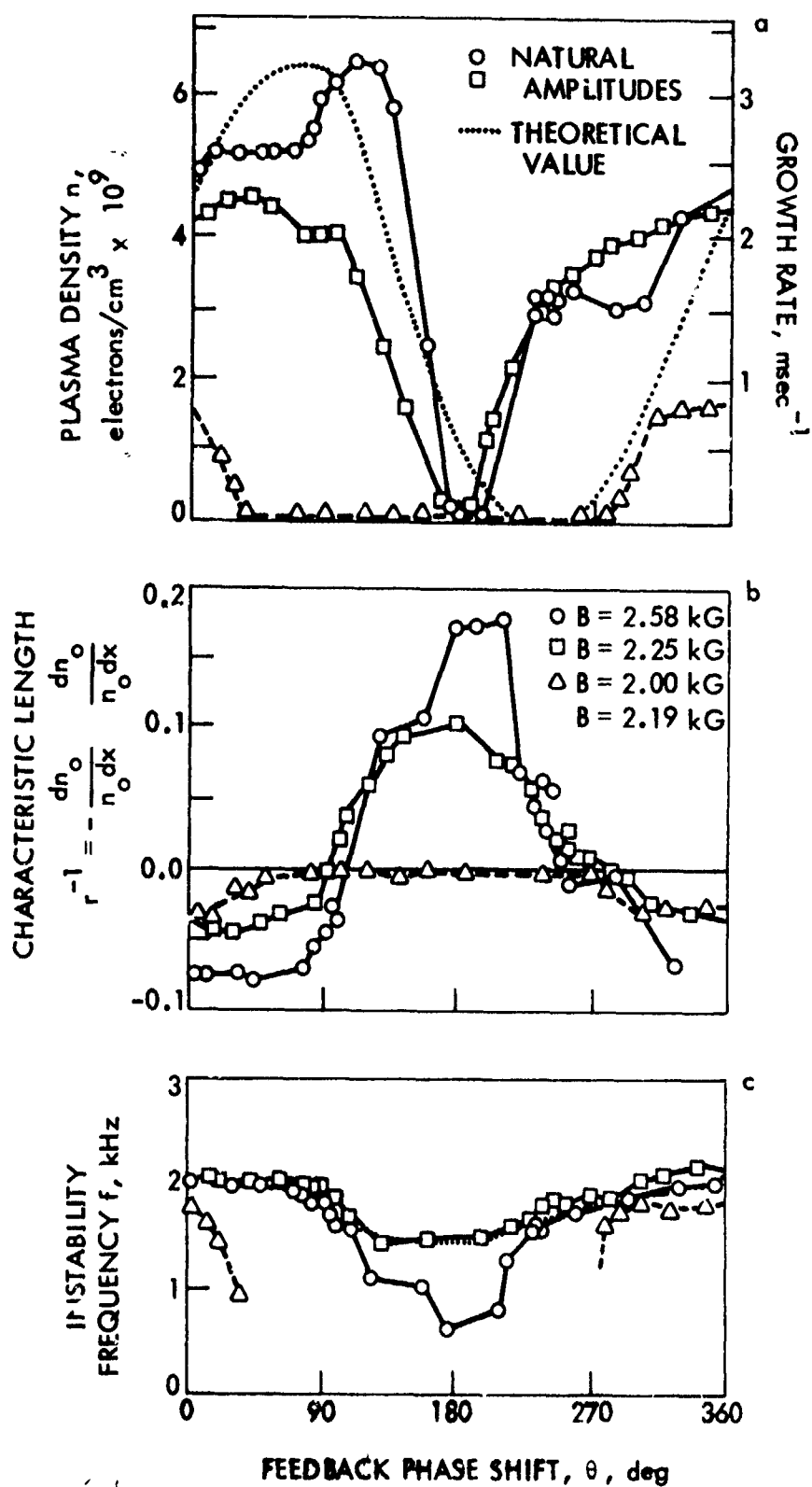
Fig. 7. Constant feedback gain v, phase shift of the applied probe (suppressor) voltage for various magnetic fields: (a) instability amplitude; (b) change of density at center of plasma column; and (c) instability frequency after subtraction of Doppler shift due to radial electric field.
