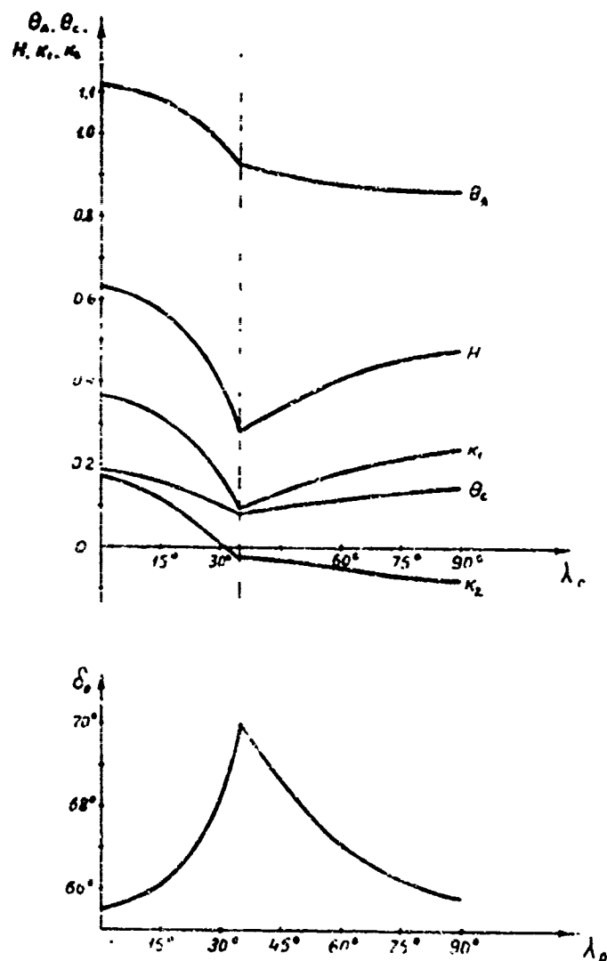
Fig. 15. Dependence of \theta_A , \theta_C , H , K_1 , K_2 , \delta_0 on \lambda_0 .
