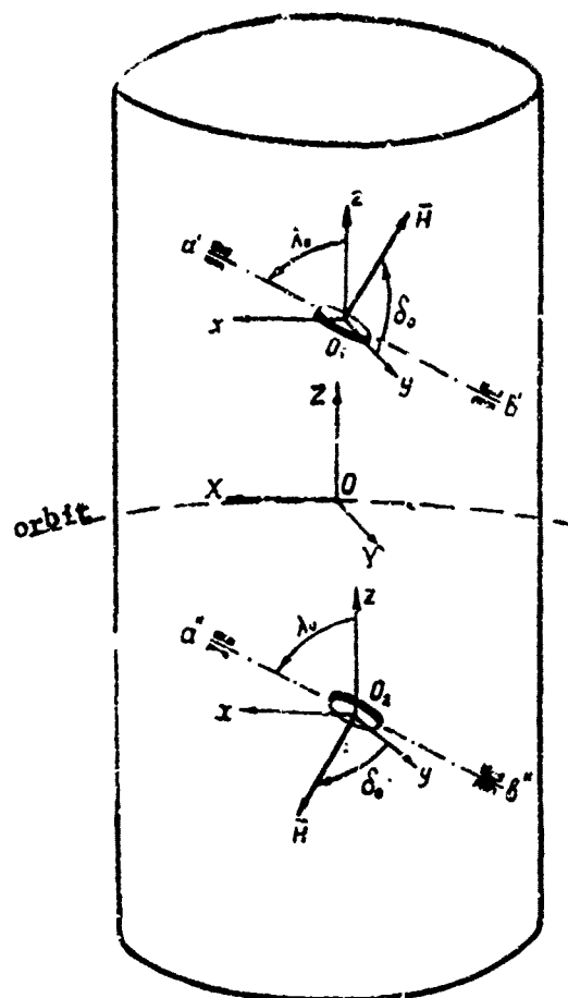
Fig. 1. Diagram of the satellite-gyroscope system.
