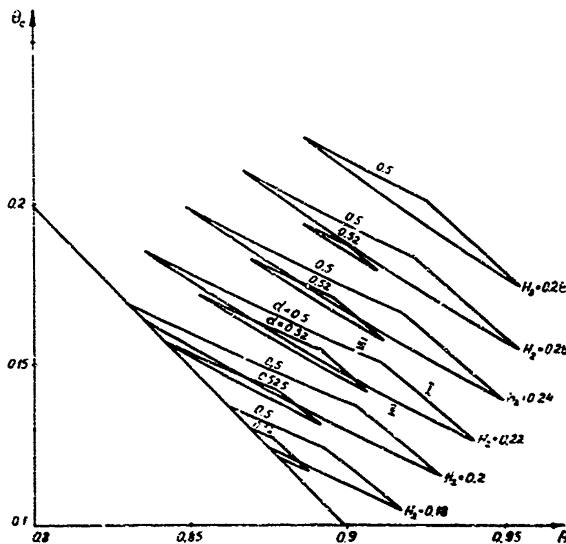
Fig. 3. Domains in which the inequalities are fulfilled for fixed values of H_2 .
