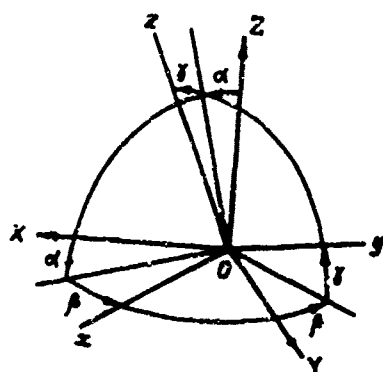
Fig. 2. Relationship between the trihedron Oxyz and the orbital coordinate system.
