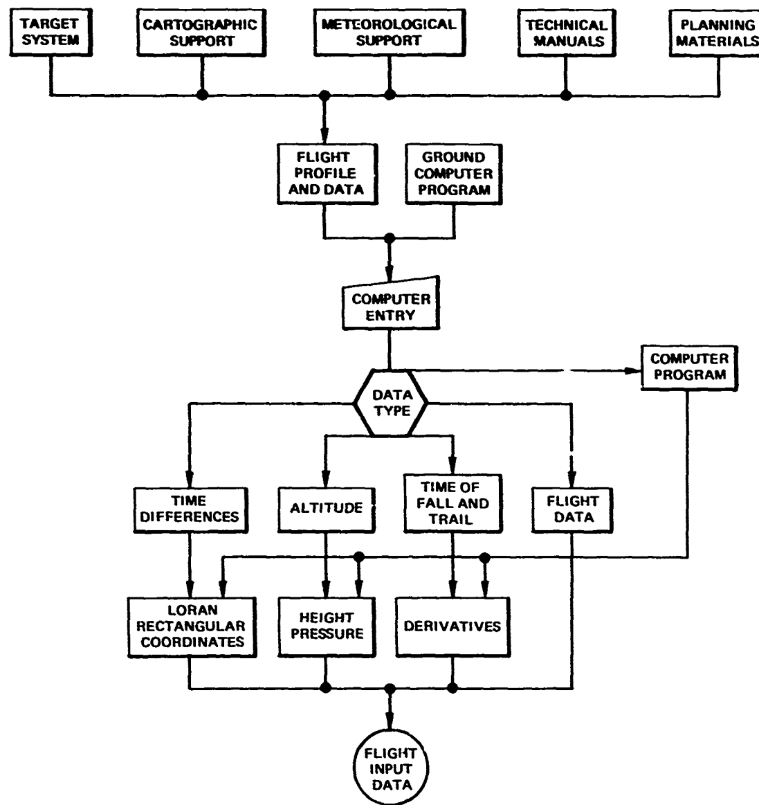
Fig. 10 GROUND SYSTEM
