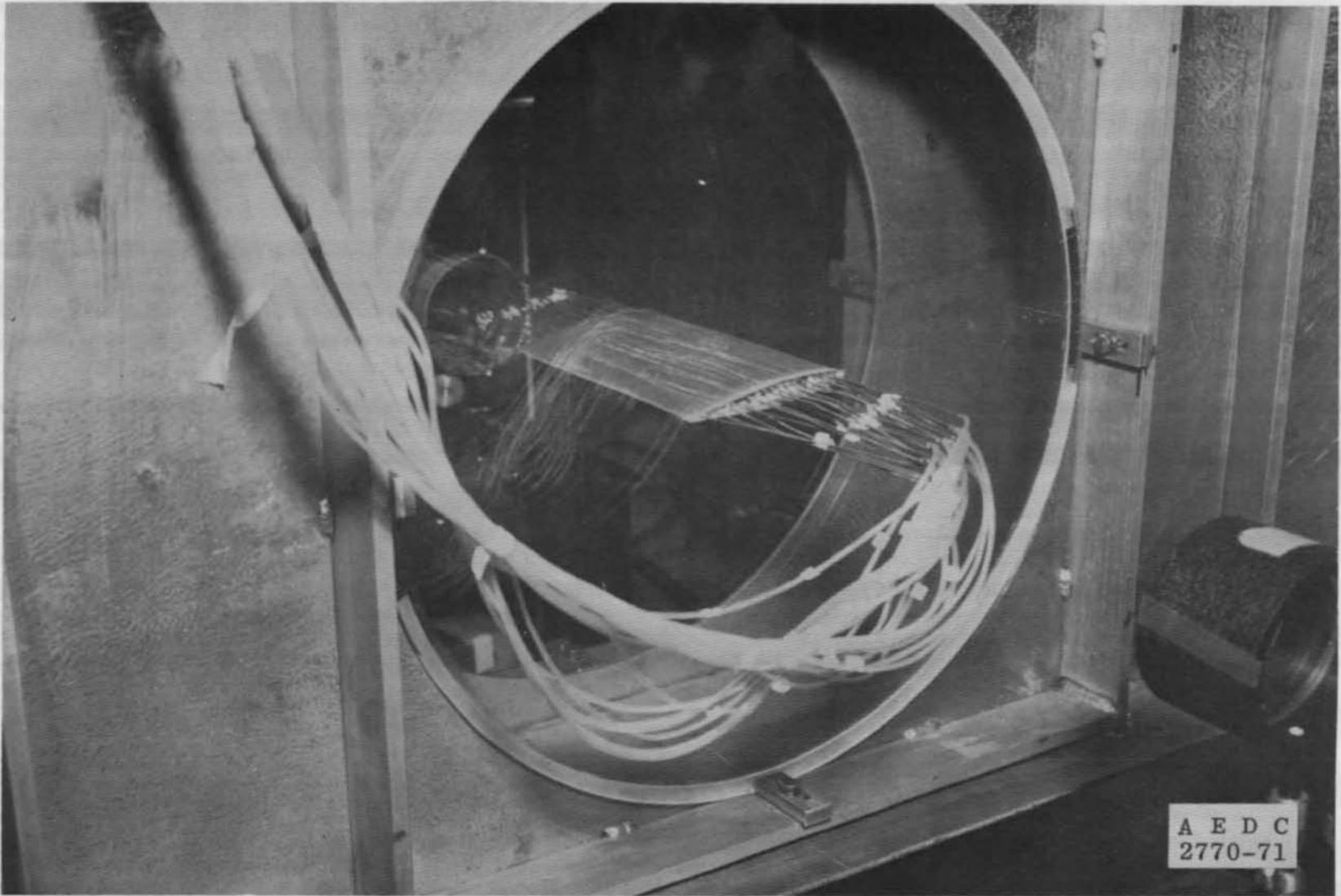
Fig. 2 Wing Mounted in Wind Tunnel Test Section
