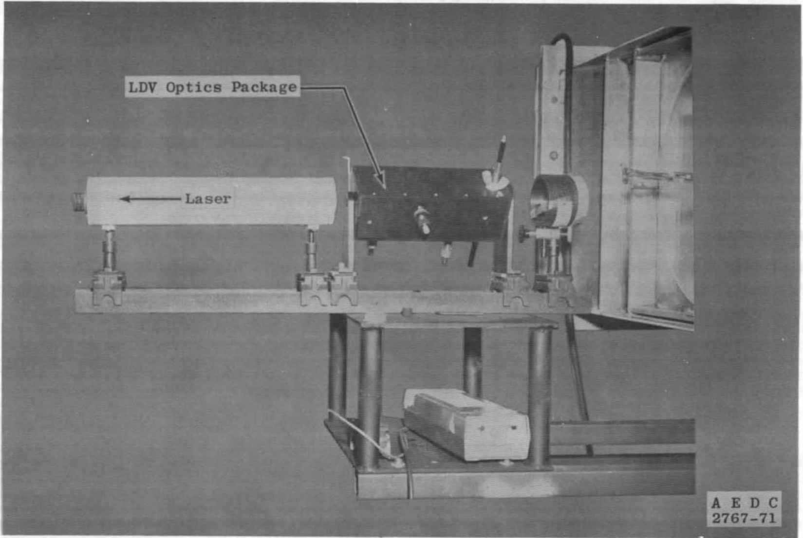
Fig. 6 Laser and Optics Package on Traversing System
