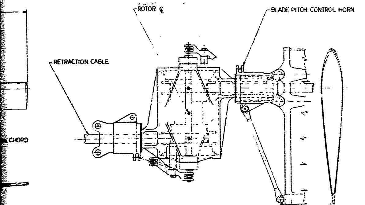
TWO BLADED TEETERING ROTOR HEAD
