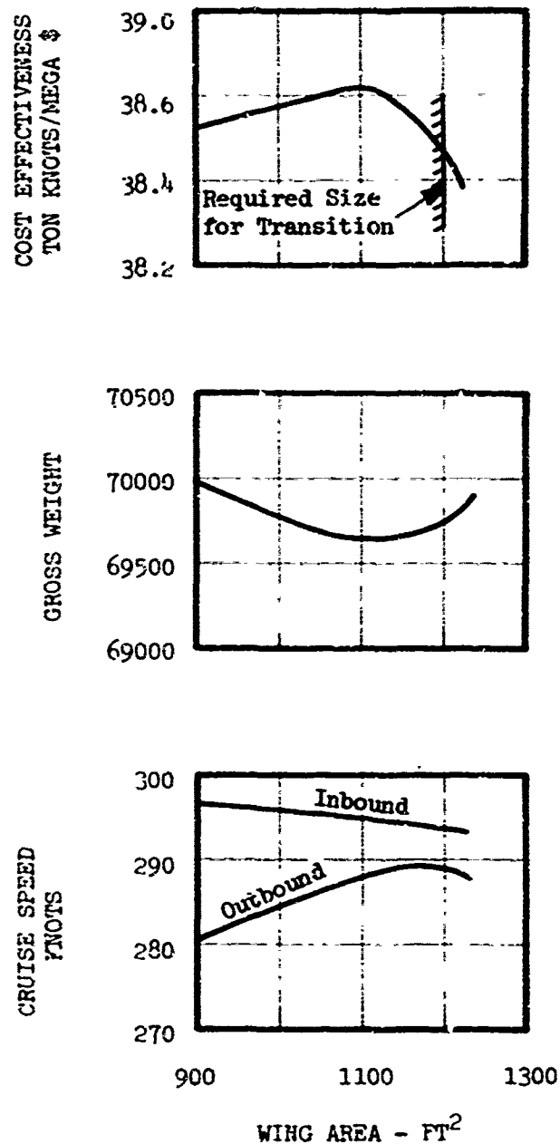
FIGURE 34 WING SIZE TRADE OFF ROLL-UP ROTOR, TWO THIN BLADES
