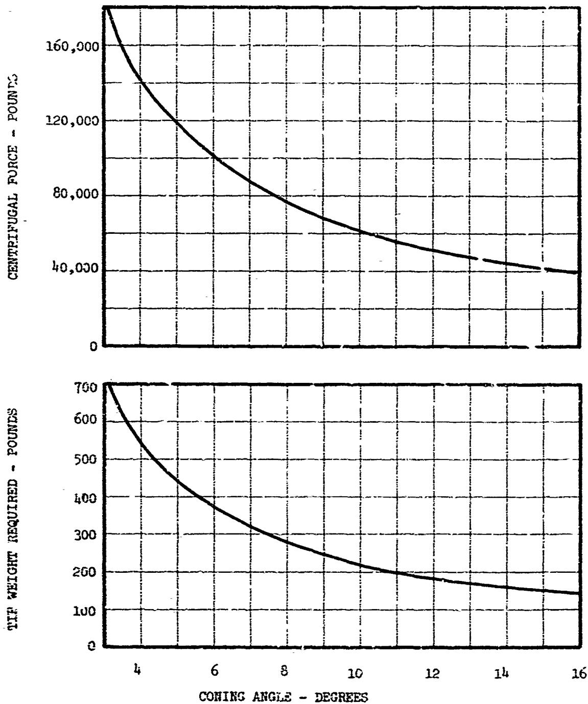
FIGURE 20 FOUR BLADED ROLL-UP ROTOR TIP WEIGHT REQUIRED
