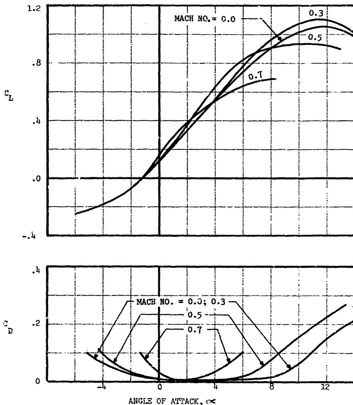
FIGURE 22 ROLL-UP ROTOR AIRFOIL CHARACTERISTICS - 2% THICK REFLEXED CAMBER AIRFOIL C_L AND C_D VERSUS ANGLE OF ATTACK
