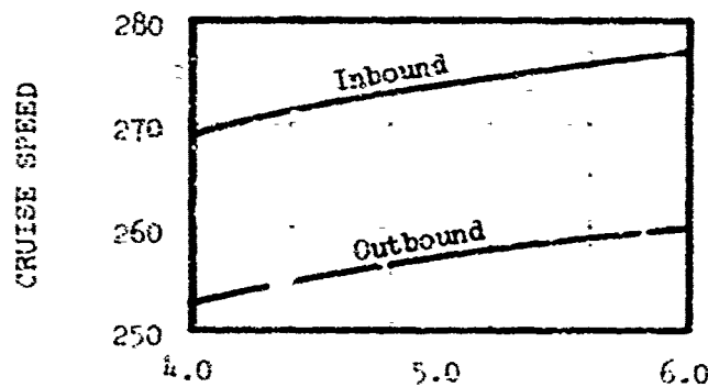
FIGURE 44 DISC LOADING TRADE OFF EIGHT SEGMENT TELESCOPING ROTOR
