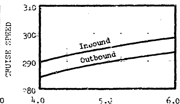
FIGURE 45 DISC LOADING TRADE OFF ROLL-UP ROTOR, TWO THIN BLADES
