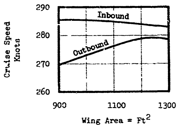
FIGURE 36 WING SIZE TRADE OFF ROLL-UP, FOUR PNEUMATIC BLADES
