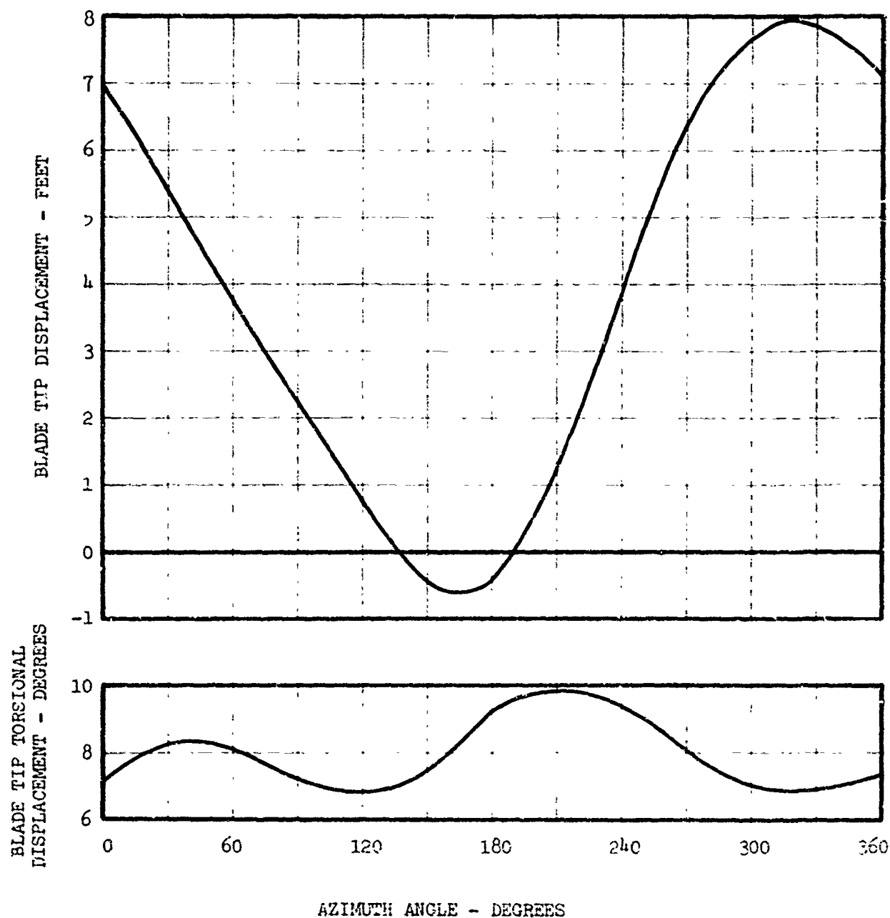
FIGURE 16 ROLL-UP ROTOR FLATWISE AND TORSIONAL RESPONSE AT 100 KNOTS, 36000 LBS LIFT ELASTIC AXIS, MASS AXIS, AND AERODYNAMIC AXIS COINCIDENT AT 25% CHORD INBOARD PITCH CONTROL.
