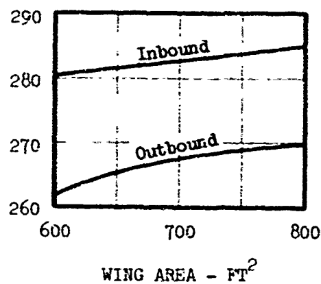
FIGURE 38 WING SIZE TRADE OFF TWO SEGMENT TELESCOPING ROTOR
