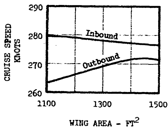
FIGURE 37 WING SIZE TRADE OFF INPLANE FOLD ROTOR
