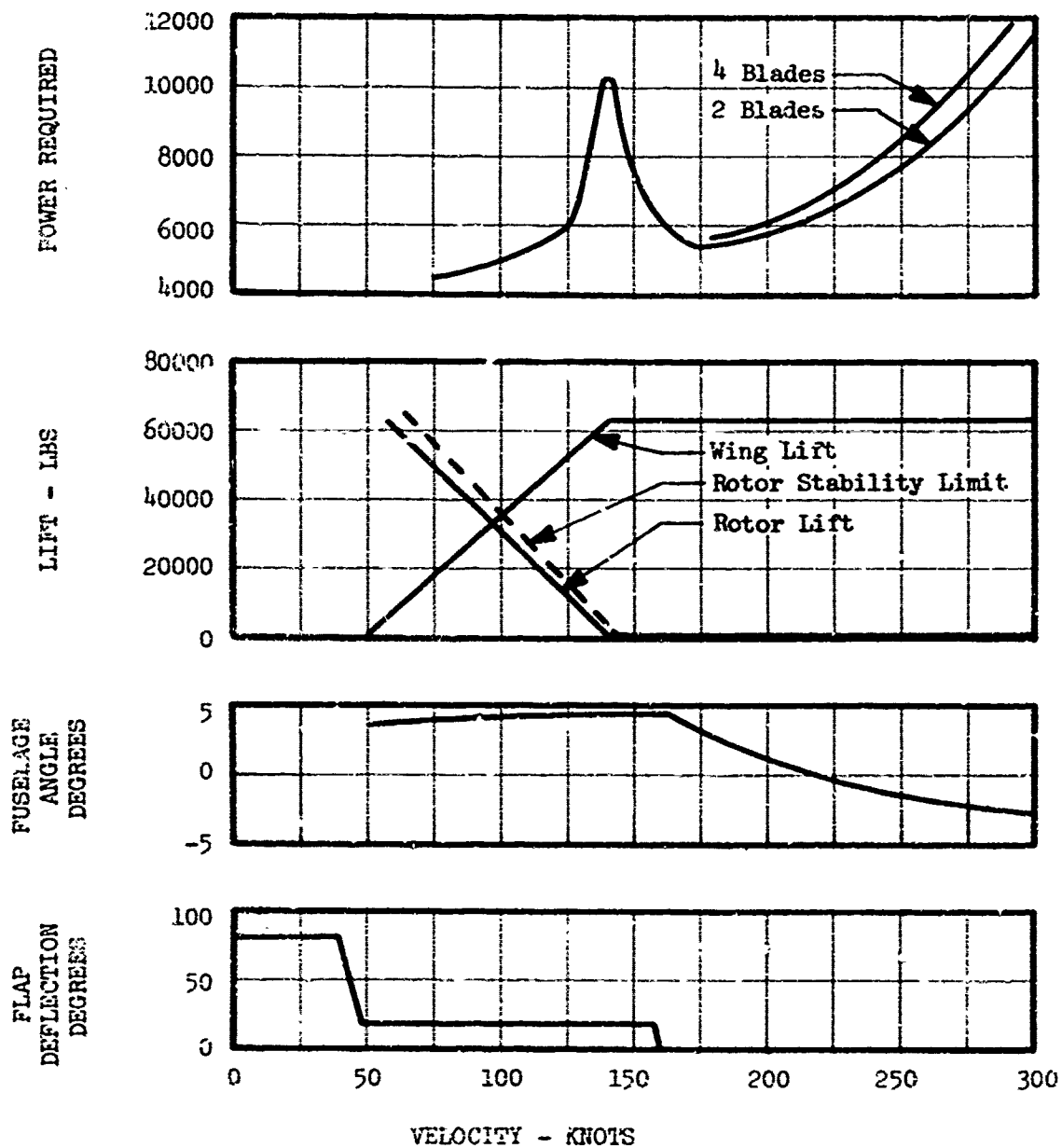
FIGURE 23 ROLL-UP ROTOR, THIN AIRFOIL - PERFORMANCE CHARACTERISTICS 12000 FT, 16°F 62800 LBS GROSS WEIGHT 1080 SQ FT WING AREA
