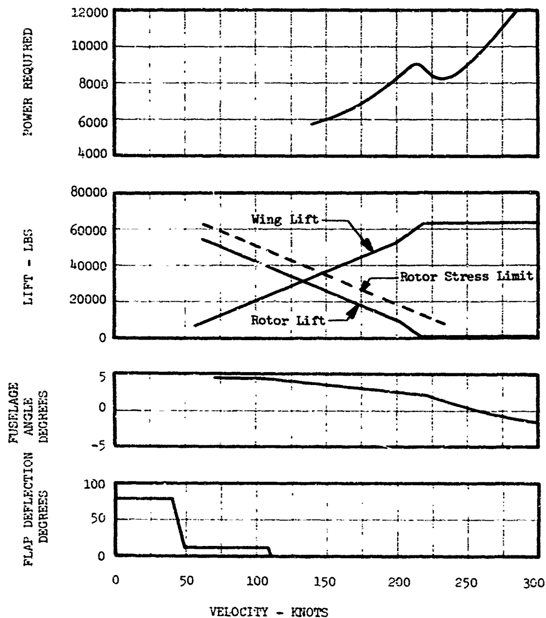
FIGURE 12 EIGHT SEGMENT TELESCOPING ROTOR PERFORMANCE CHARACTERISTICS 12000 FT, 16° F 62900 LBS GROSS WEIGHT 750 SQ FT WING AREA
