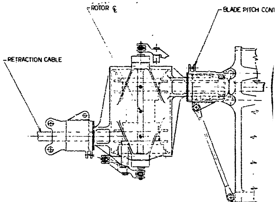
TWO BLADED TEETERING ROTOR HEAD
