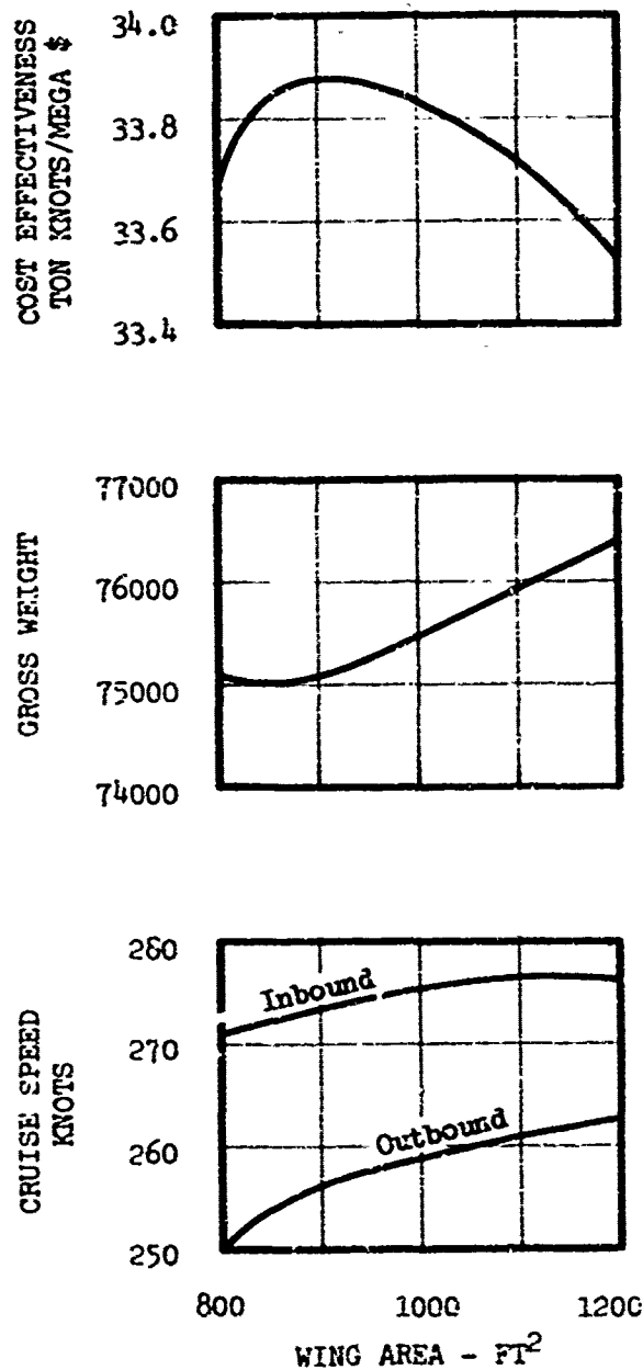
FIGURE 33 WING SIZE TRADE OFF EIGHT SEGMENT TELESOPING ROTOR
