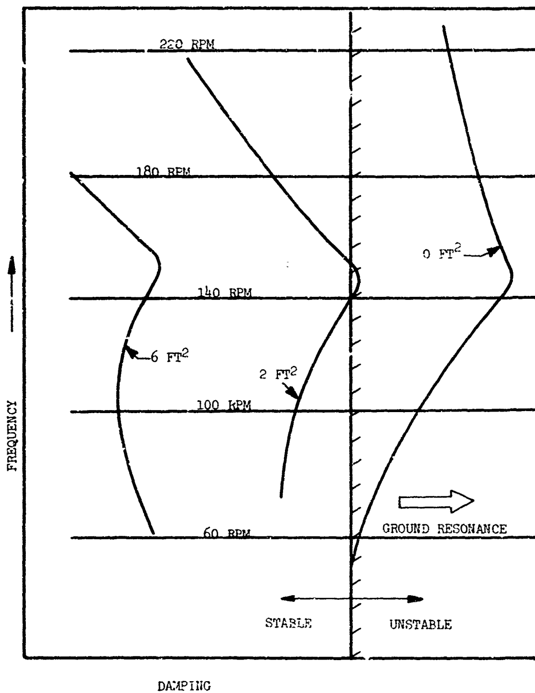
FIGURE 15 ROLL-UP ROTOR EFFECT OF DRAG VALVE AREA AND ROTOR SPEED ON STABILITY
