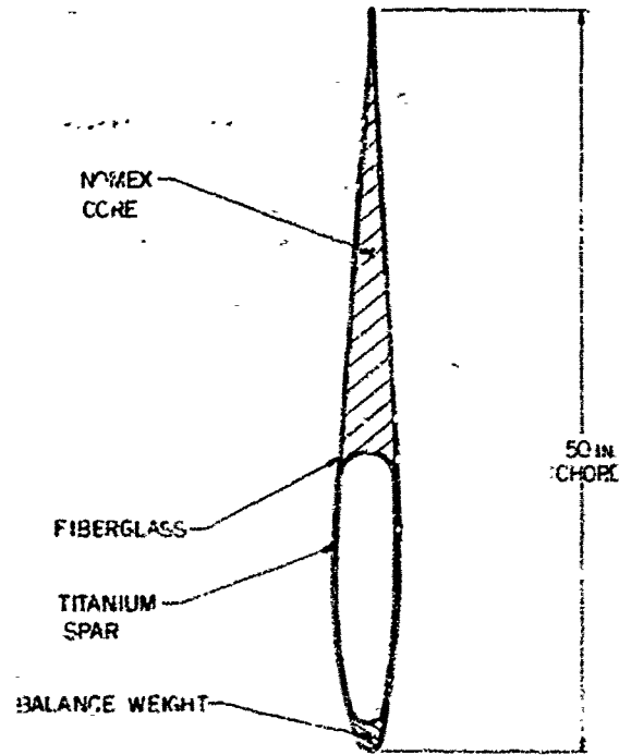
BLADE CONSTRUCTION
