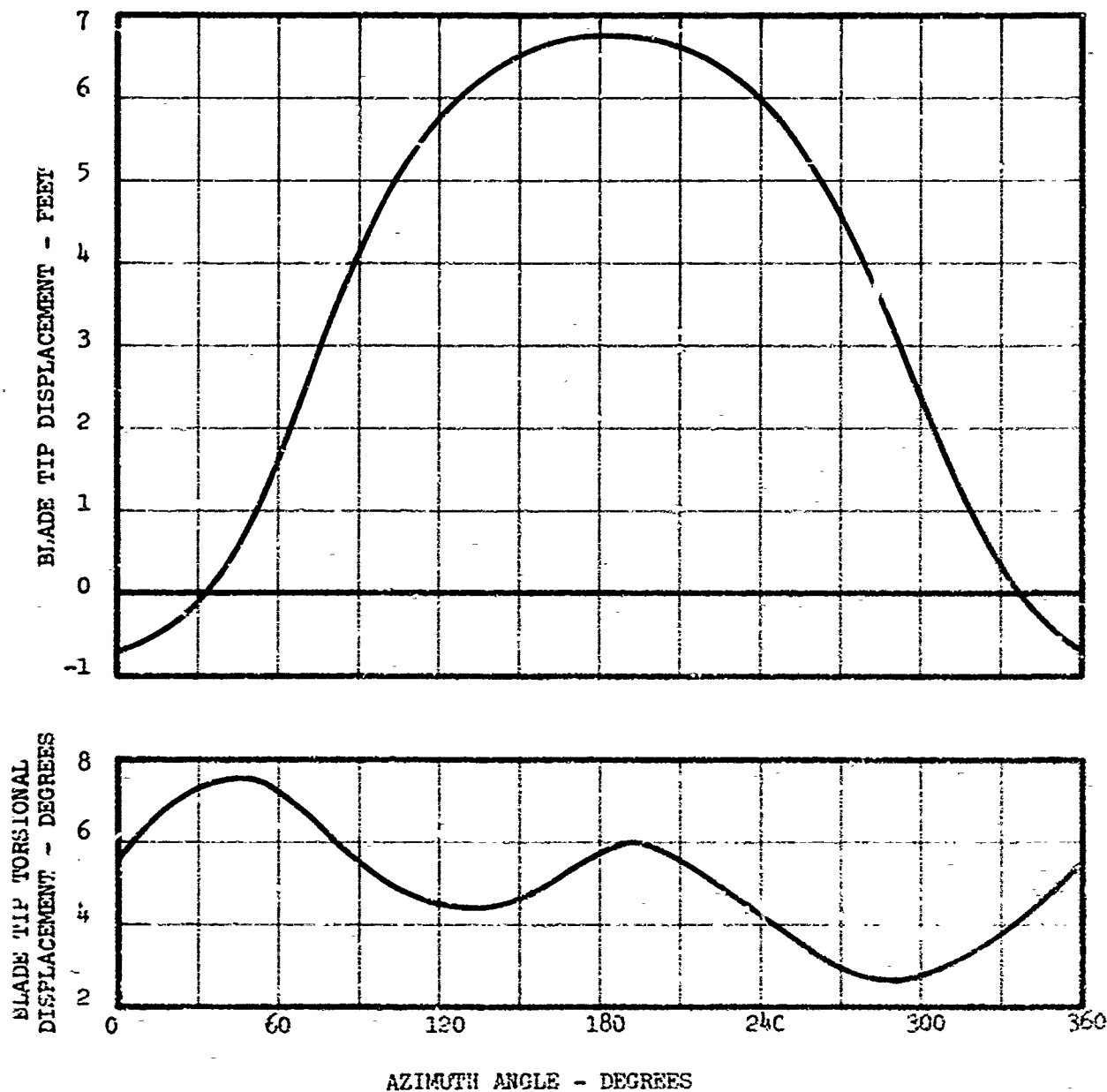
FIGURE 19 ROLL-UP ROTOR FLATWISE AND TORSIONAL RESPONSE AT 100 KNOTS, 36500 LBS LIFT ELASTIC AXIS & MASS AXIS AT 23% CHORD; AERODYNAMIC AXIS AT 25% CHORD BLADE TIP PITCH CONTROL
