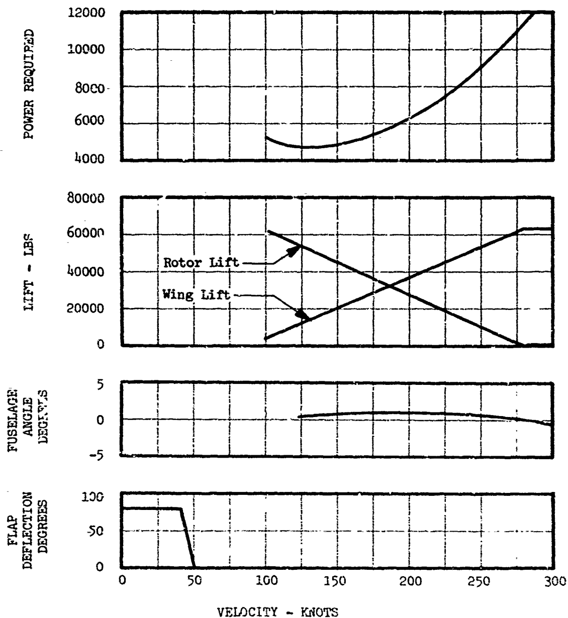
FIGURE 31 TWO SEGMENT TELESCOPING ROTOR - PERFORMANCE CHARACTERISTICS 12000', 16° 62800 LBS GROSS WEIGHT 610 SQ FT WING AREA
