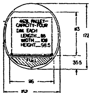
CADN SECTION
