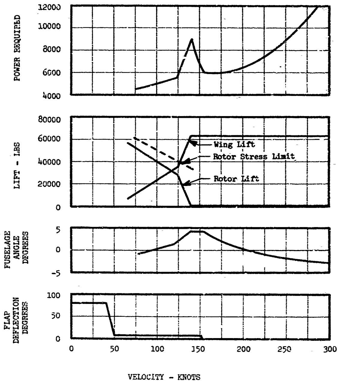
FIGURE 27 INPLANE FOLD ROTOR - PERFORMANCE CHARACTERISTICS 12000', 16° 62000 LBS GROSS WEIGHT 1080 SQ FT WING AREA
