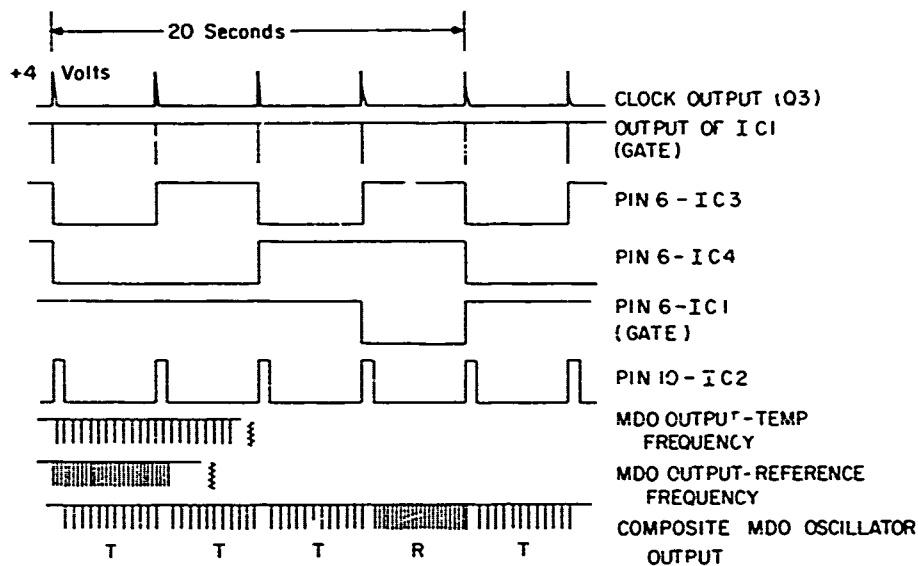
Figure 4. Timing Diagram
