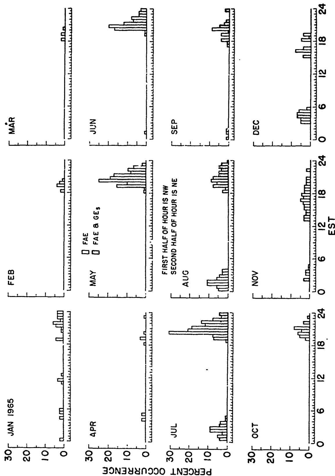
FIG. 6 BACKSCATTER FROM FIELD ALIGNED IRREGULARITIES AT E-LAYER HEIGHTS FOR K F1 0-3 DURING 1965
